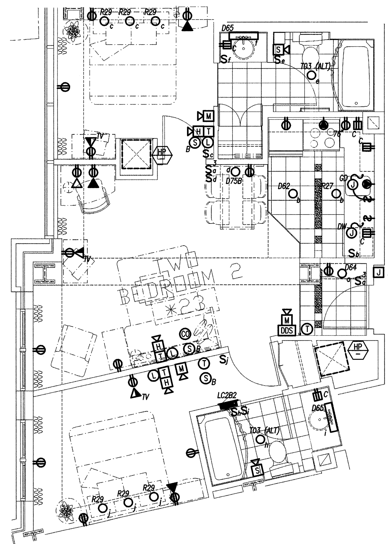
B TWO BEDROOM TWO - ENLARGED FLOOR PLAN 1/4" = 1'-0" (REFERENCE DRAWING A1.33)
