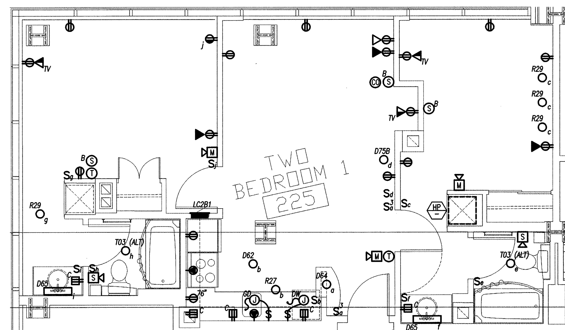
A TWO BEDROOM ONE - ENLARGED FLOOR PLAN 1/4" = 1'-0" (REFERENCE DRAWING A1.31)
