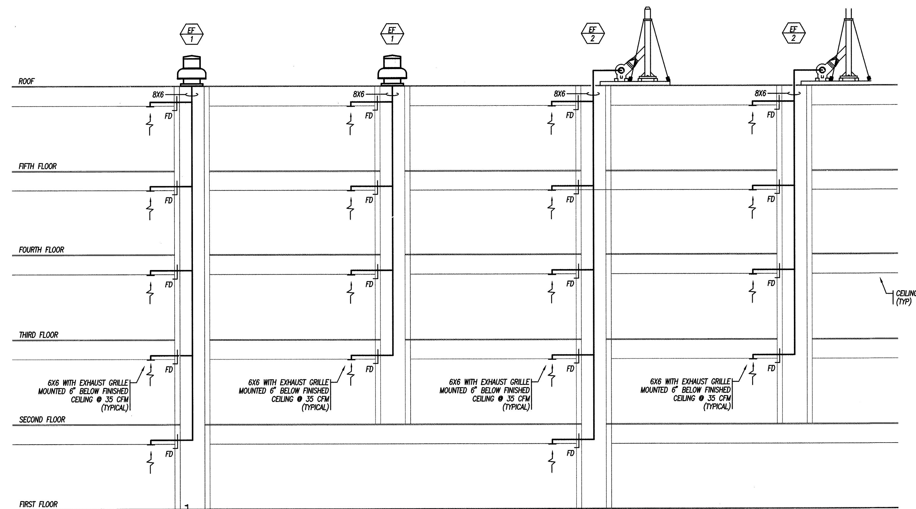
GUEST ROOM EXHAUST RISERS FANS EF-1 AND EF-2
