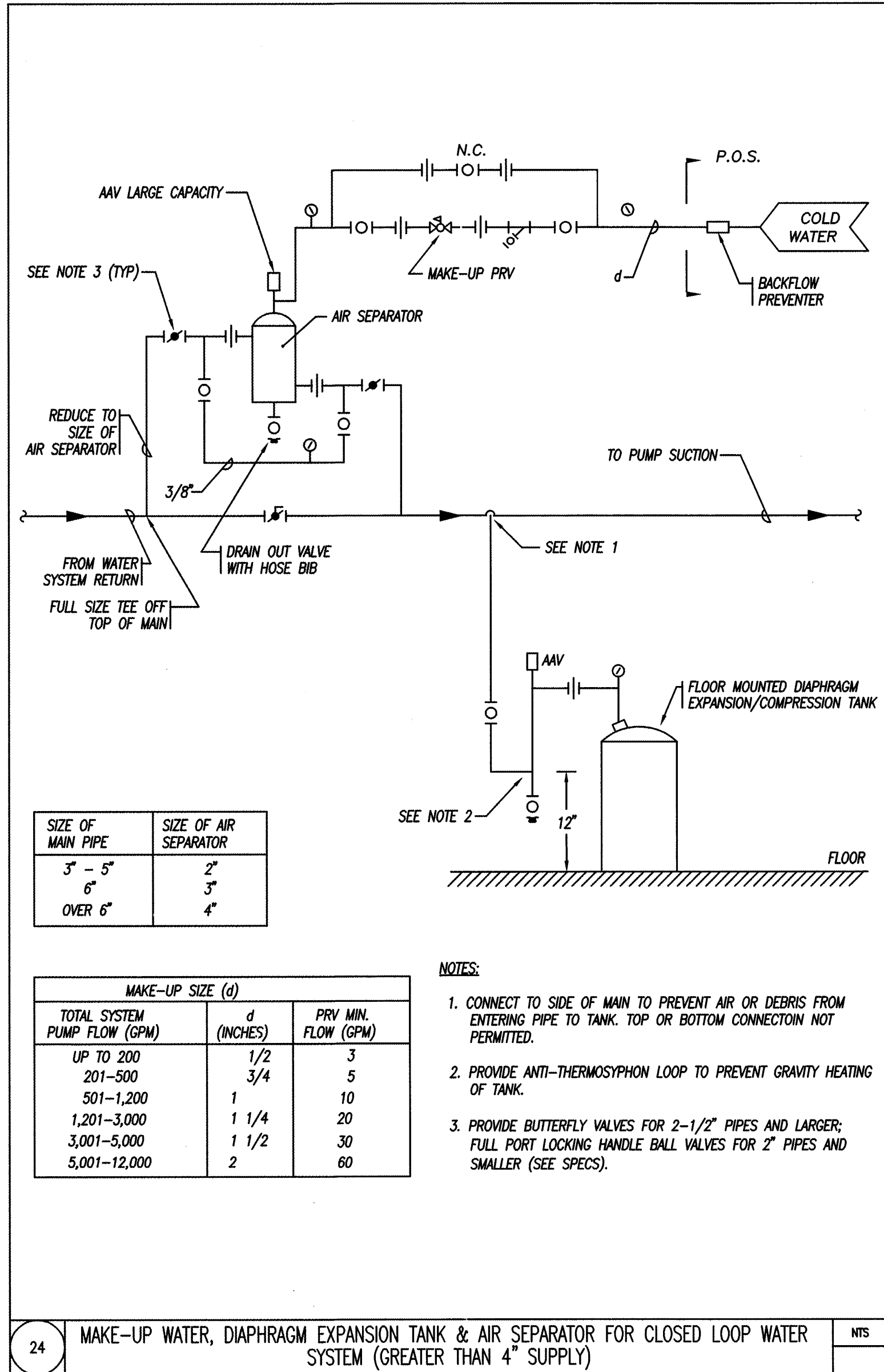
MAKE-UP WATER, DIAPHRAGM EXPANSION TANK & AIR SEPARATOR FOR CLOSED LOOP WATER SYSTEM (GREATER THAN 4" SUPPLY)
