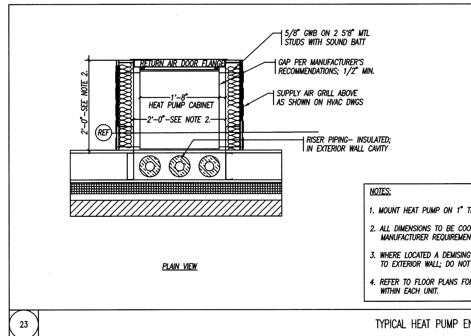
TYPICAL HEAT PUMP ENCLOSURE DETAIL
