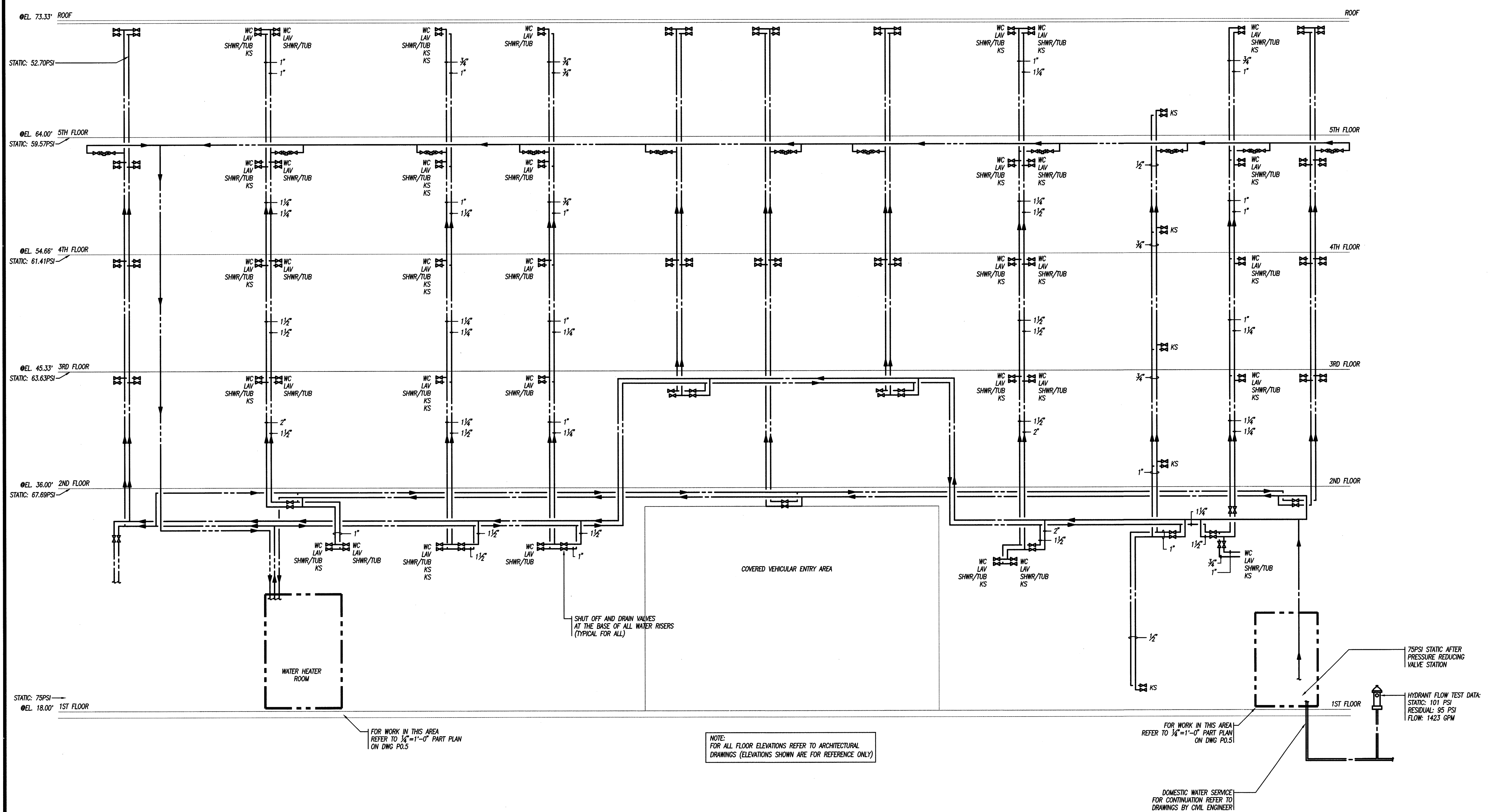
A DIAGRAMATIC WATER RISER NOT TO SCALE. DOES NOT REFLECT ACTUAL NUMBER, ORIENTATION OR LOCATION OF WATER RISERS
