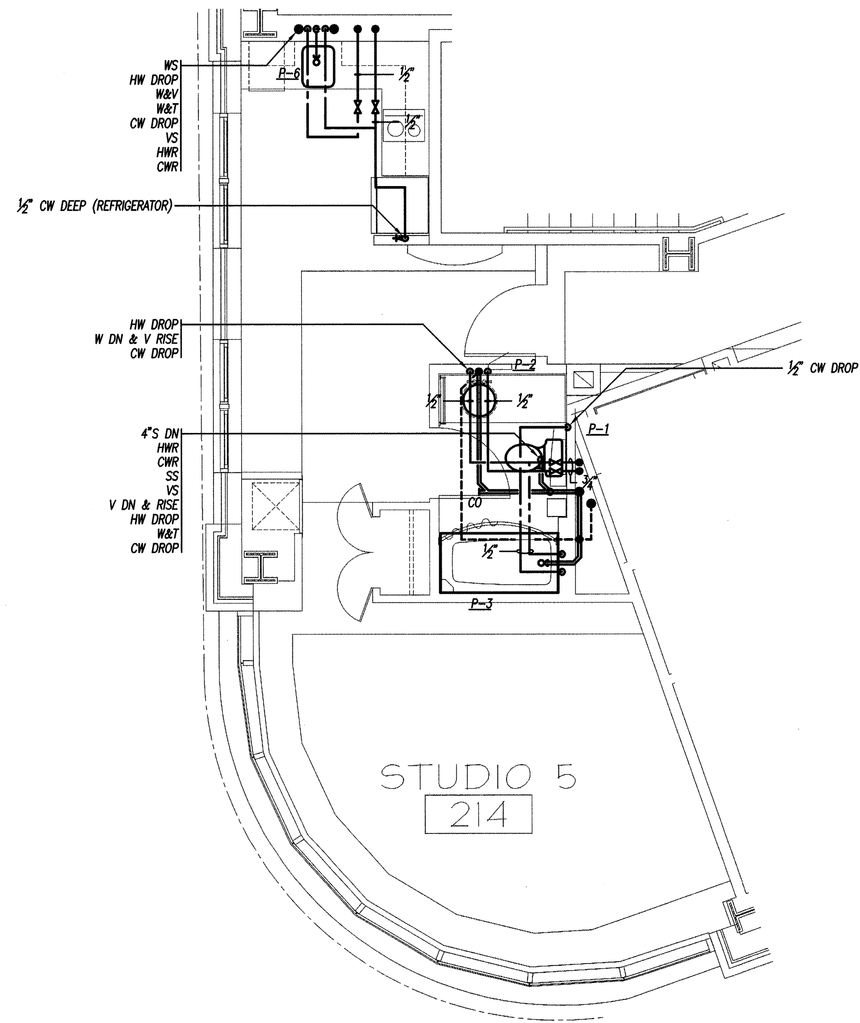
D STUDIO 5 - ENLARGED FLOOR PLAN 1/4" = 1'-0"
