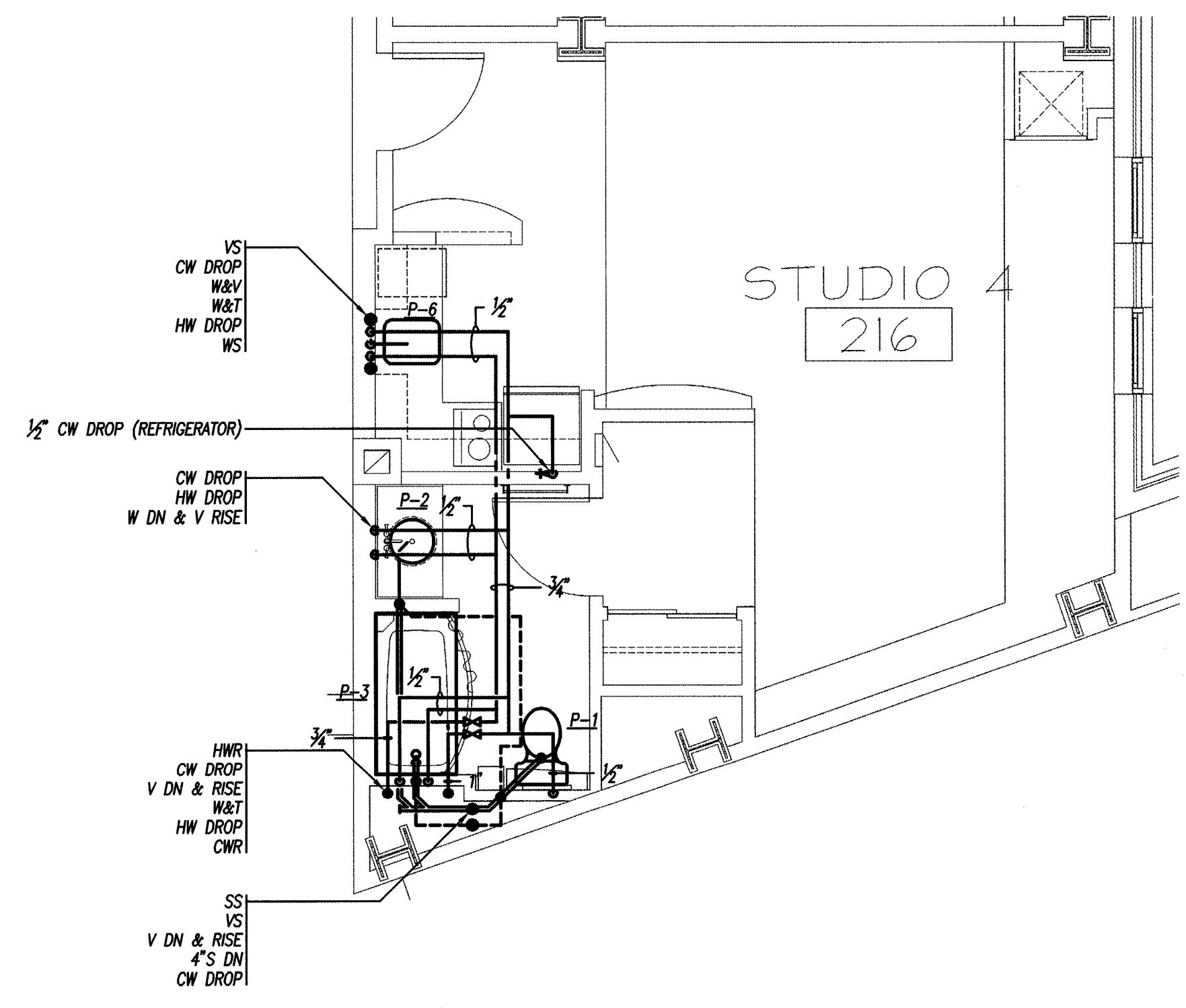
C STUDIO 4 - ENLARGED FLOOR PLAN 1/4" = 1'-0"
