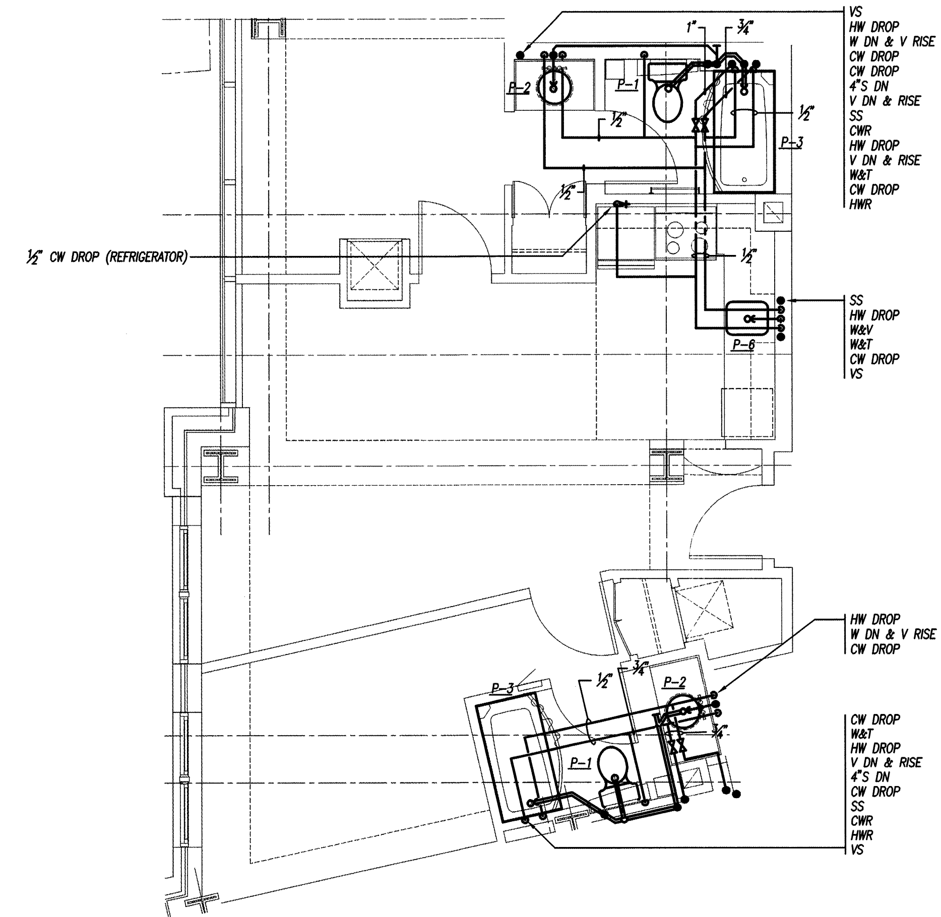
B TWO BEDROOM TWO - ENLARGED FLOOR PLAN 1/4" = 1'-0"
