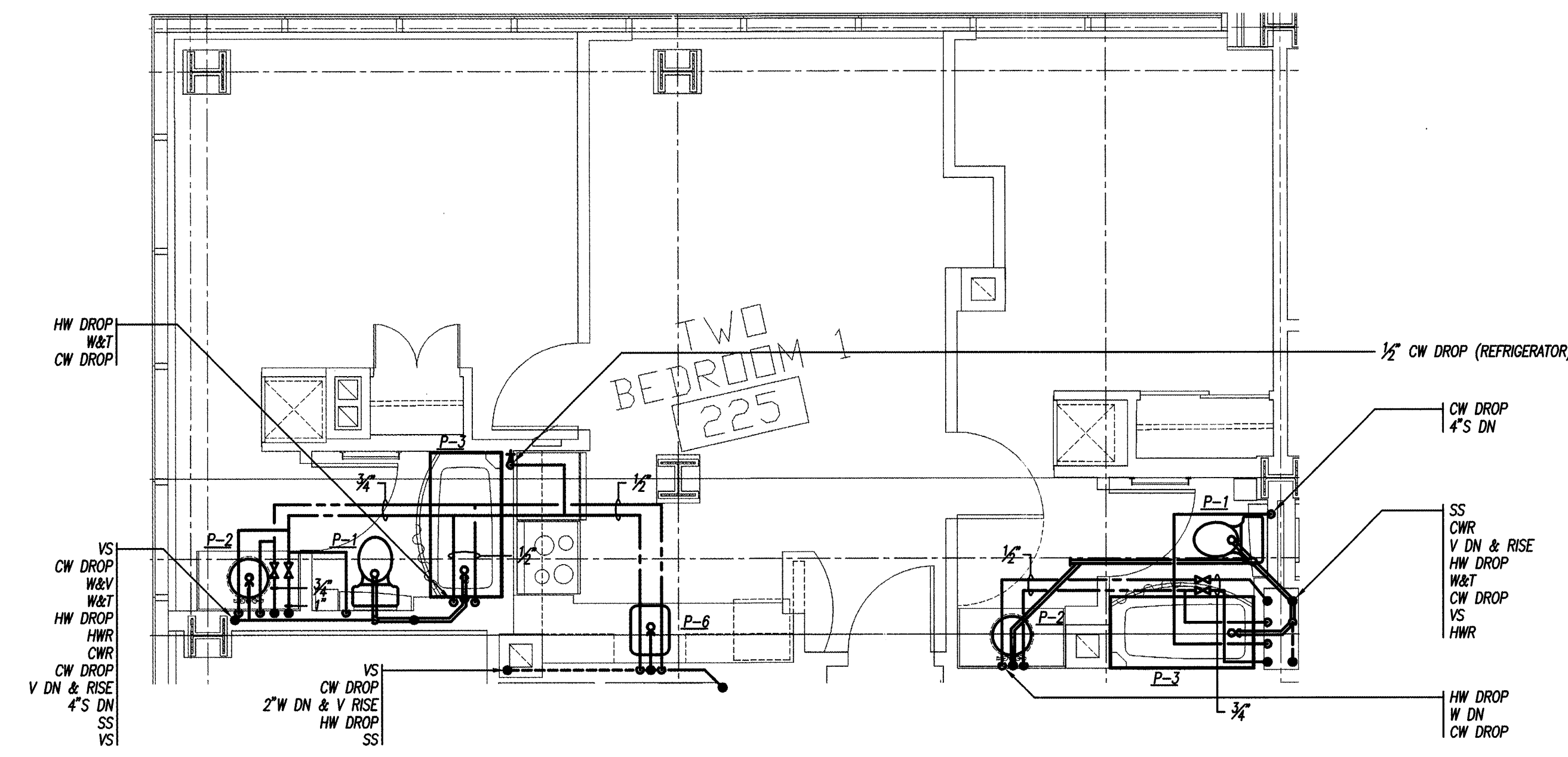
A TWO BEDROOM ONE - ENLARGED FLOOR PLAN 1/4" = 1'-0"
