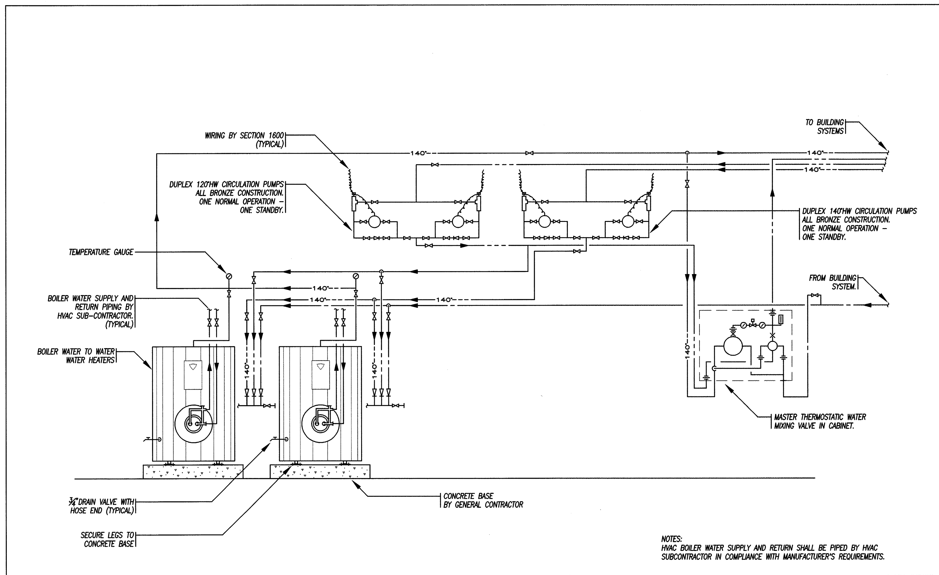
4 DUPLEX BOILER WATER TO WATER, WATER HEATERS (2 temperature system) NOT TO SCALE
