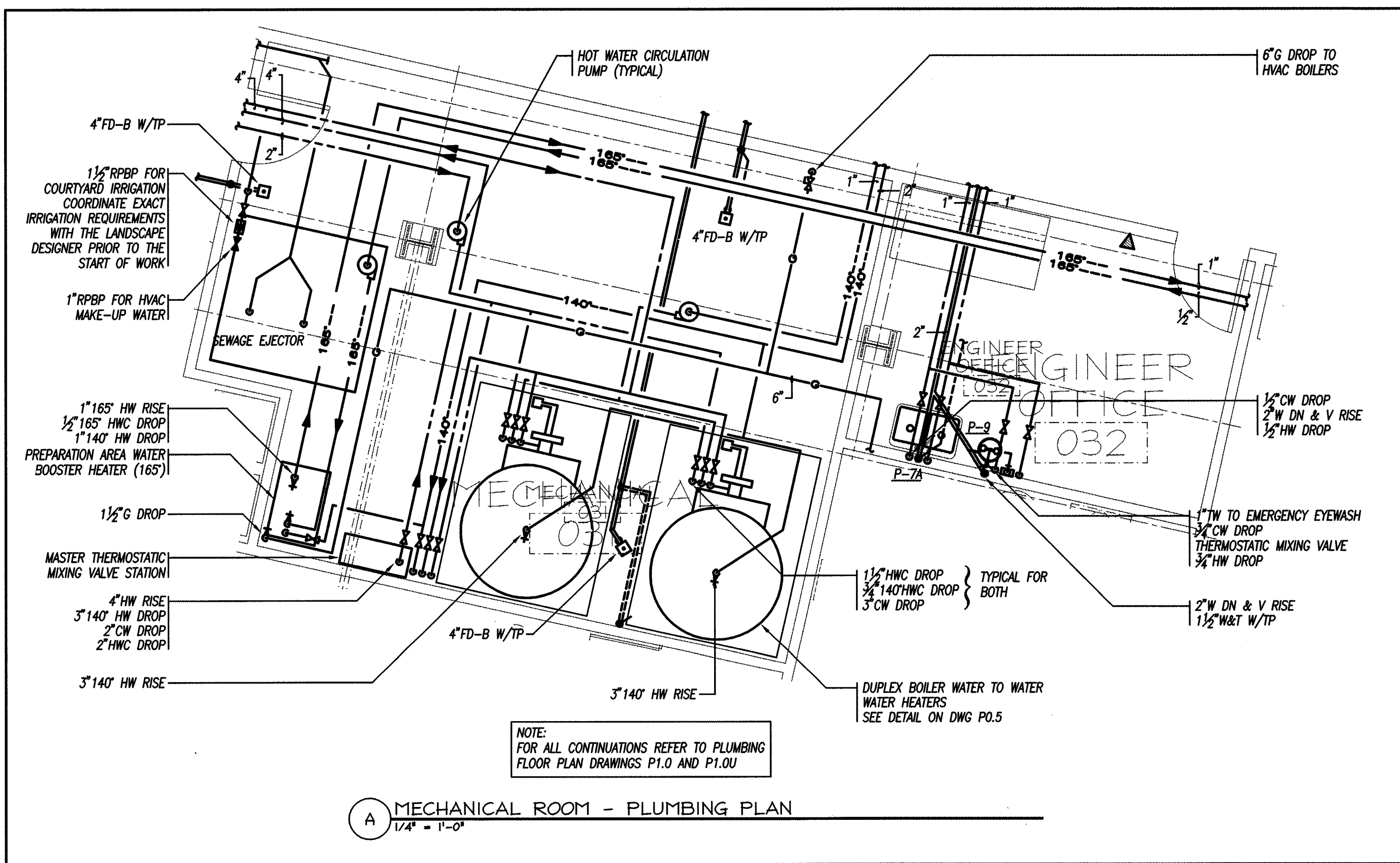
A MECHANICAL ROOM - PLUMBING PLAN 1/4\"/>
