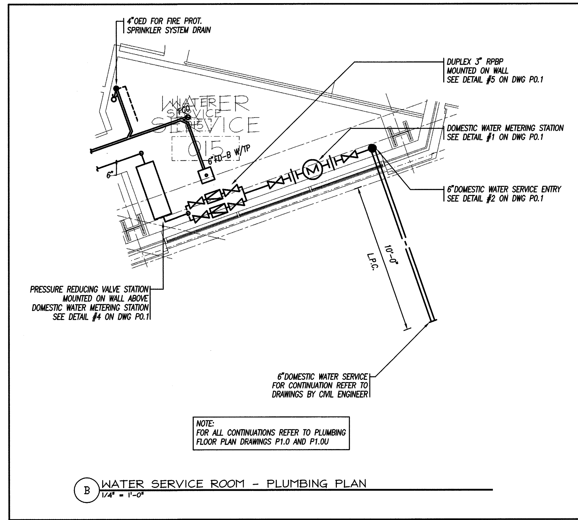
B WATER SERVICE ROOM - PLUMBING PLAN 1/4\"/>
