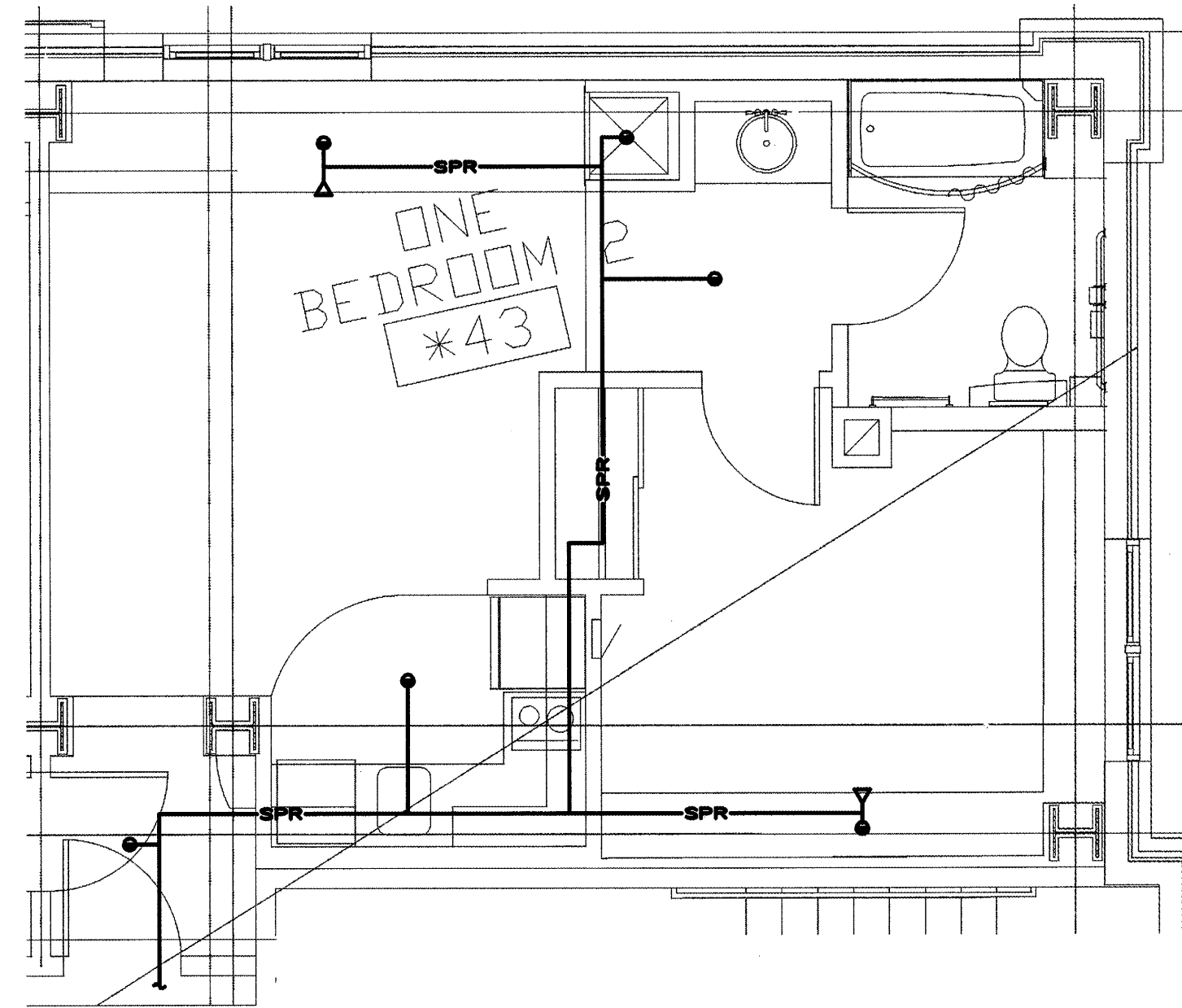
A ONE BEDROOM TWO - ENLARGED FLOOR PLAN 1/4" = 1'-0"
