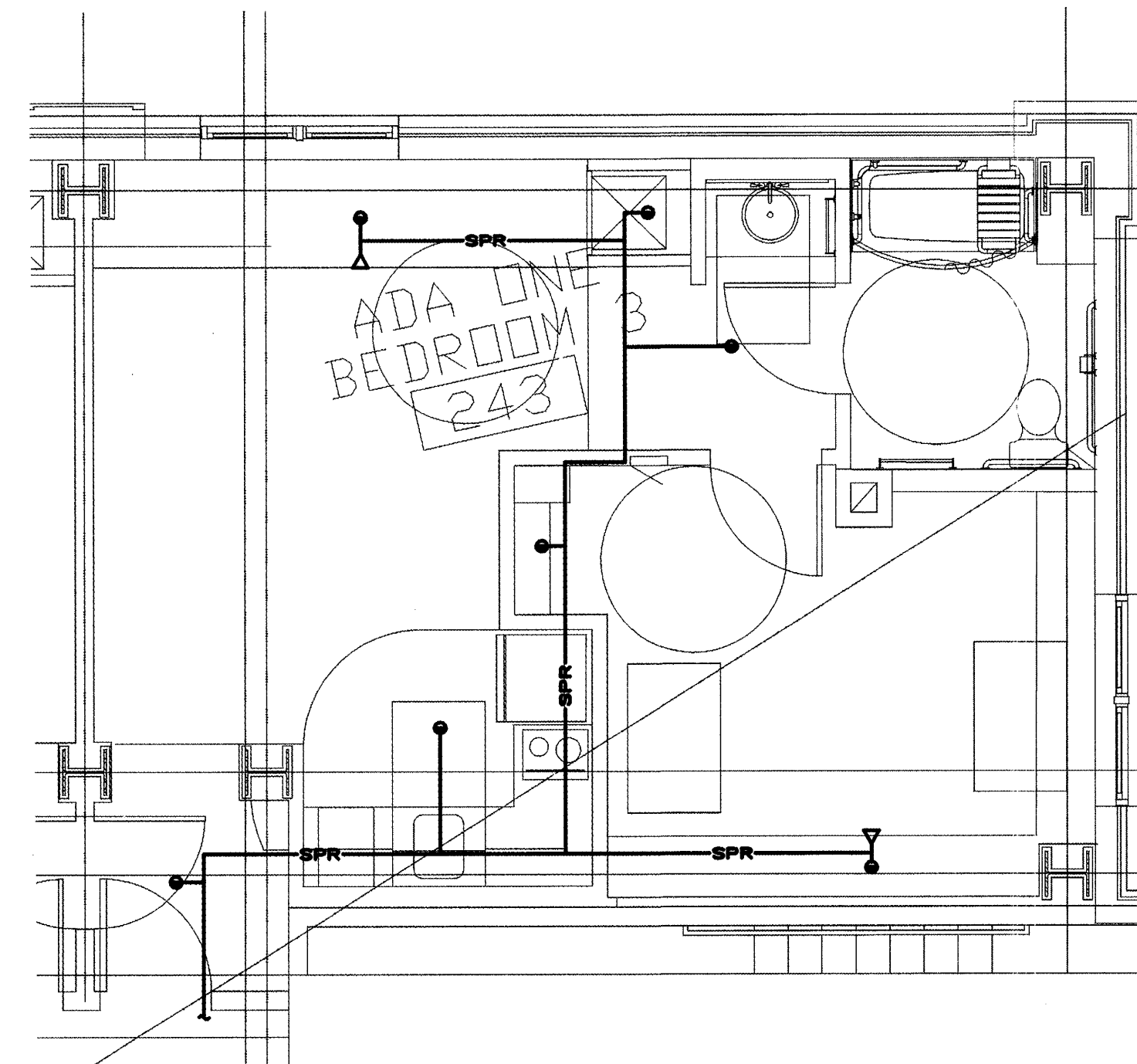
B ONE BEDROOM THREE ADA - ENLARGED FLOOR PLAN 1/4" = 1'-0"
