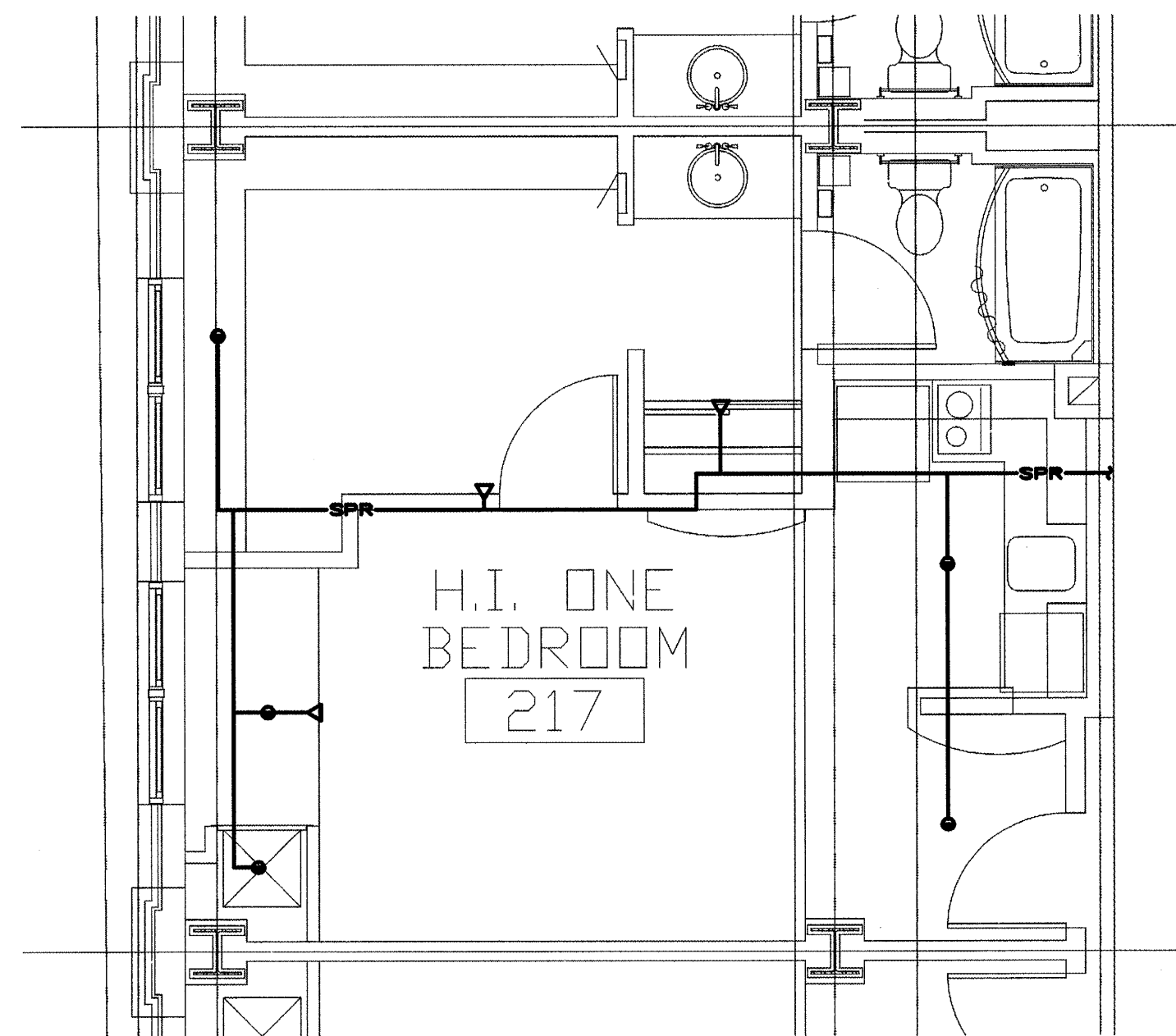
C ONE BEDROOM ONE - ENLARGED FLOOR PLAN 1/4" = 1'-0"
