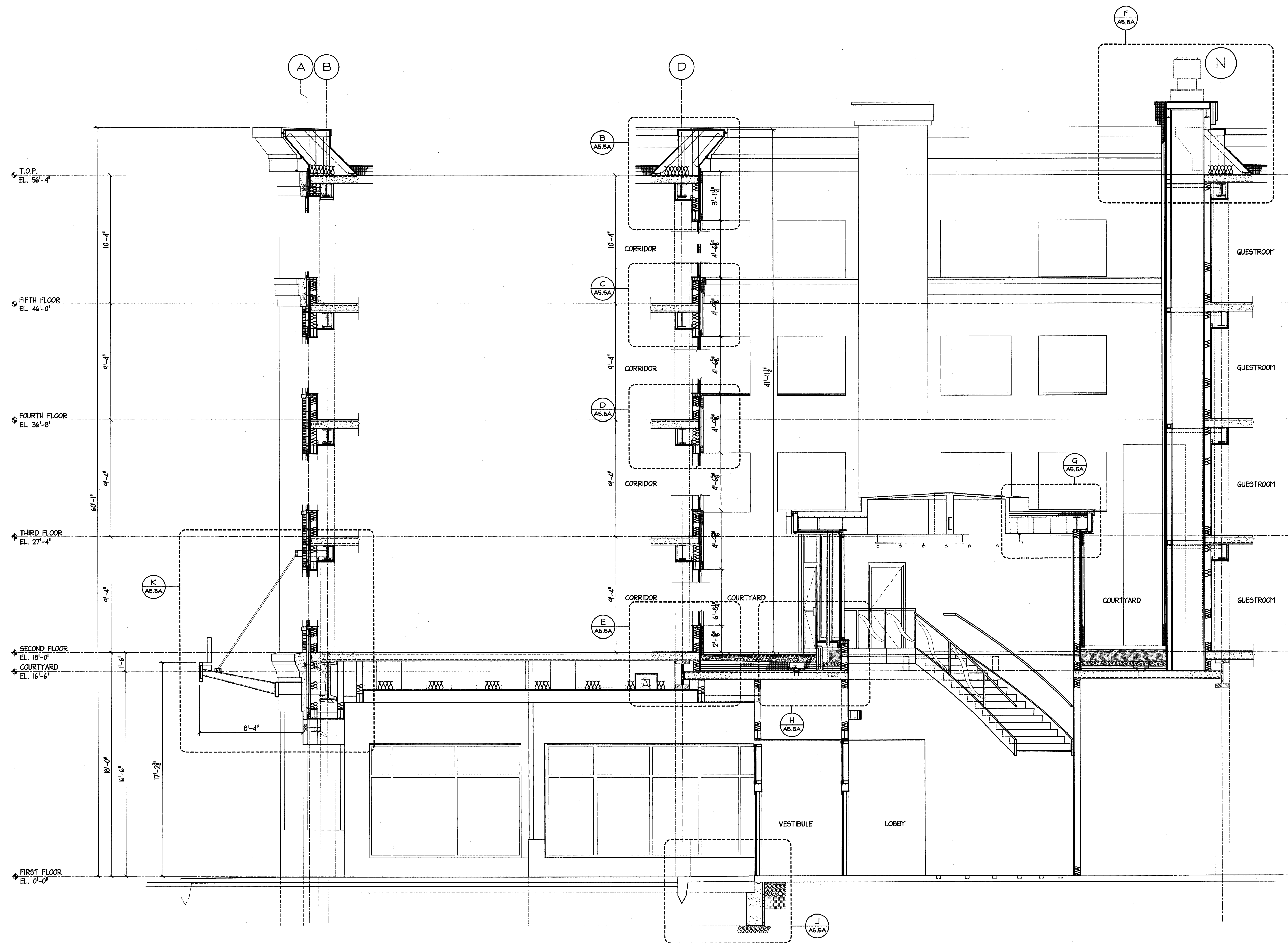
A CROSS SECTION 1/4"=1'-0"
