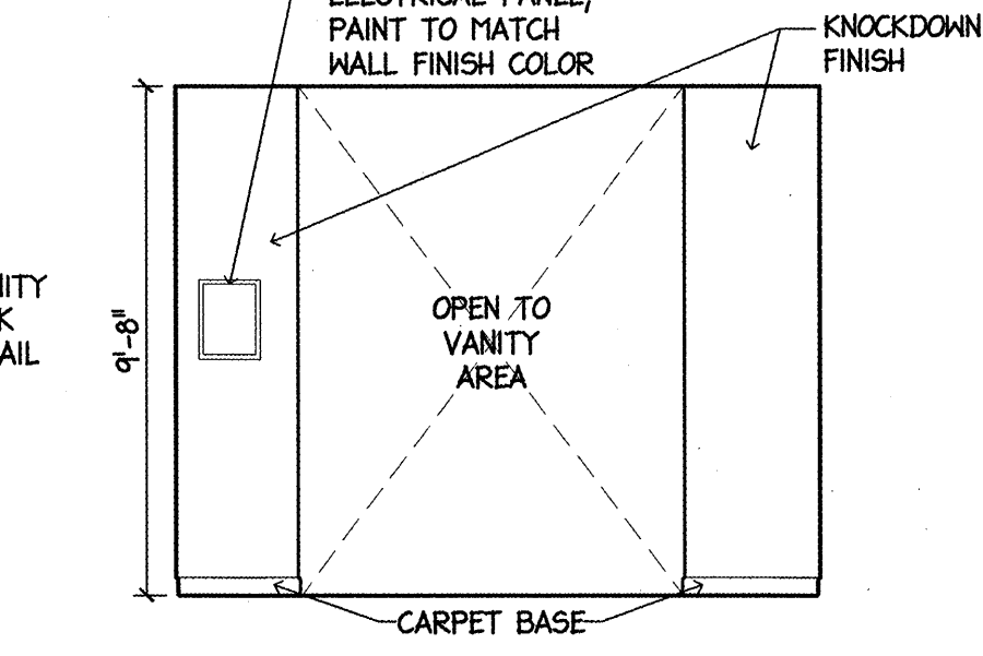
7 I BEDROOM 4 ADA ELEVATION 1/4" = 1'-0"
