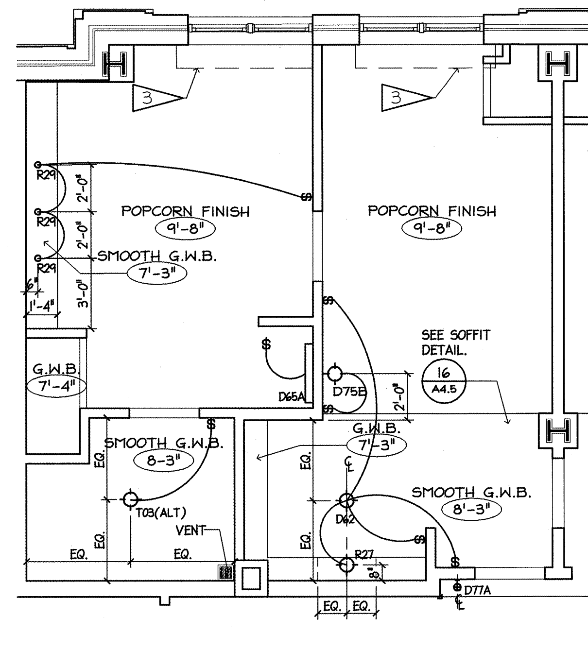
C I BEDROOM 4 ADA - ENLARGED REFLECTED CEILING PLAN 1/4" = 1'-0"
