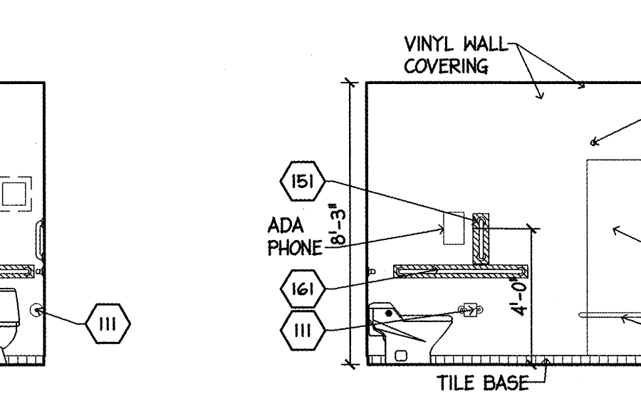
10 I BEDROOM 4 ADA ELEVATION 1/4" = 1'-0"
