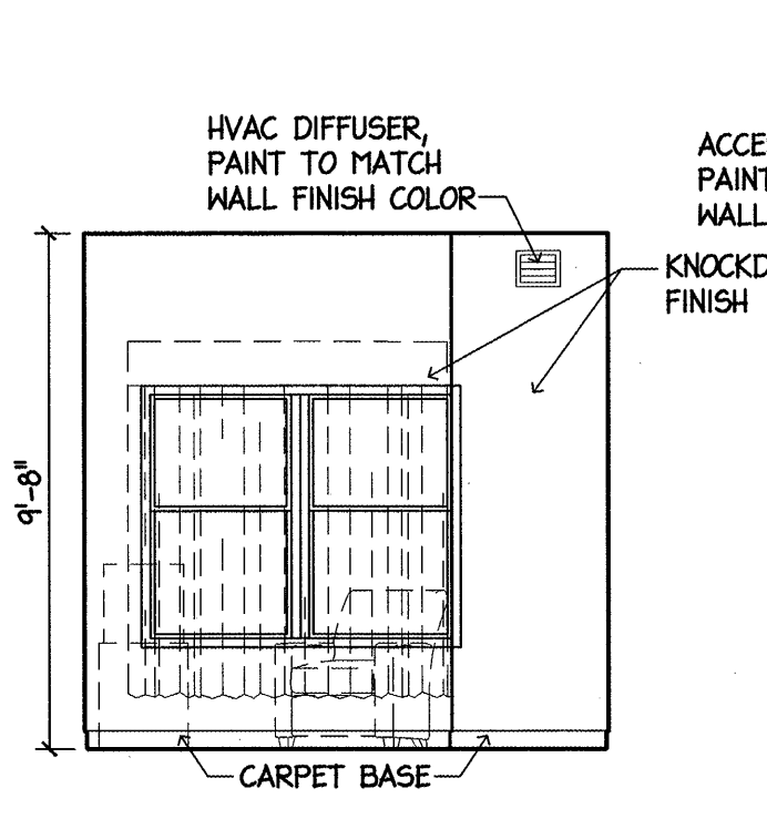
1 I BEDROOM 4 ADA ELEVATION 1/4" = 1'-0"
