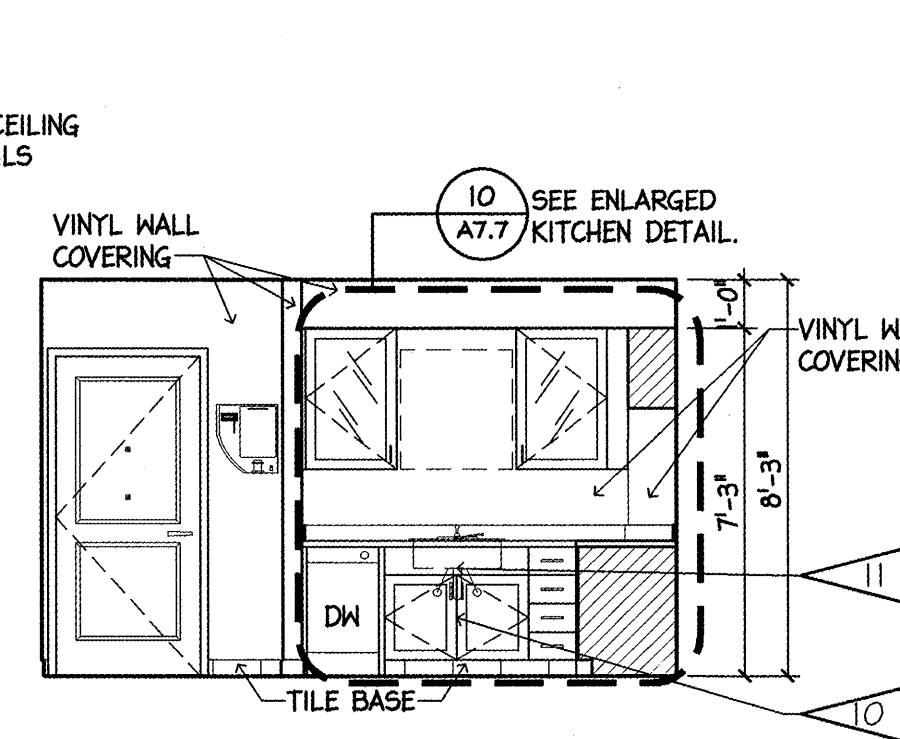
3 I BEDROOM 4 ADA ELEVATION 1/4" = 1'-0"
