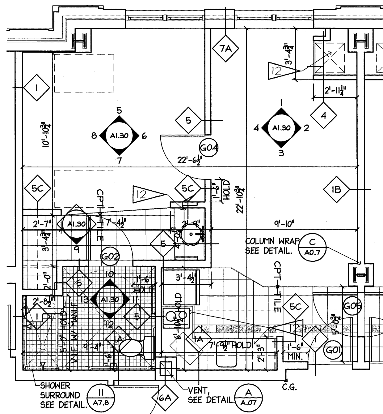
A I BEDROOM 4 ADA - ENLARGED FLOOR PLAN 1/4" = 1'-0"
