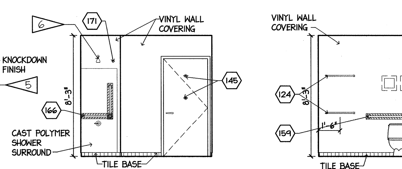
10 I BEDROOM 4 ADA ELEVATION 1/4" = 1'-0"
