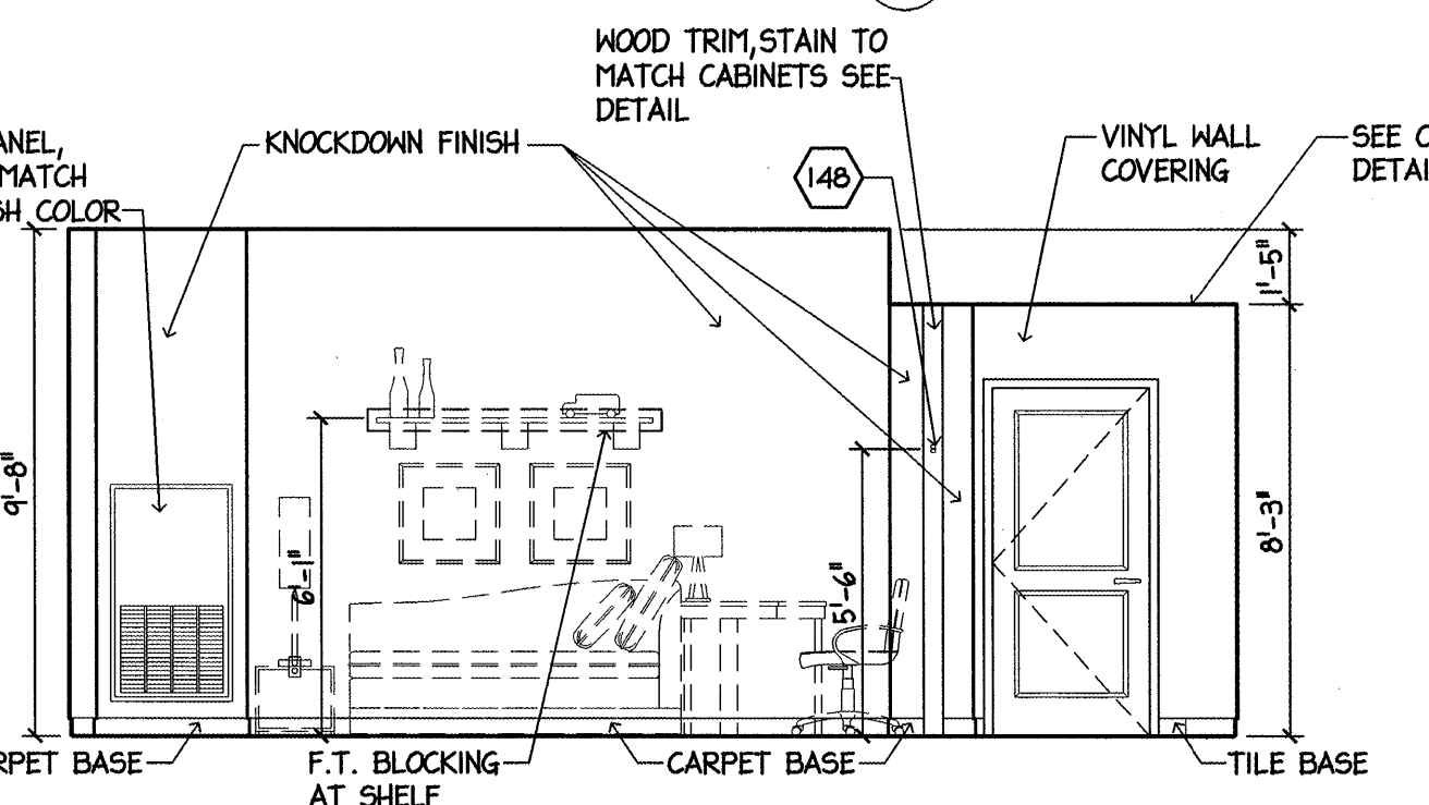
2 I BEDROOM 4 ADA ELEVATION 1/4" = 1'-0"
