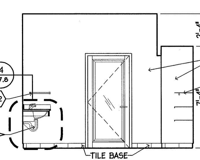
9 I BEDROOM 4 ADA ELEVATION 1/4" = 1'-0"
