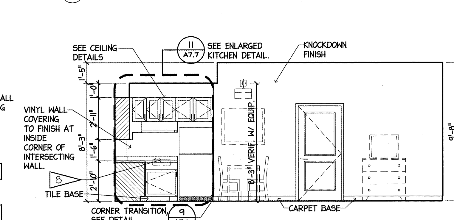
4 I BEDROOM 4 ADA ELEVATION 1/4" = 1'-0"
