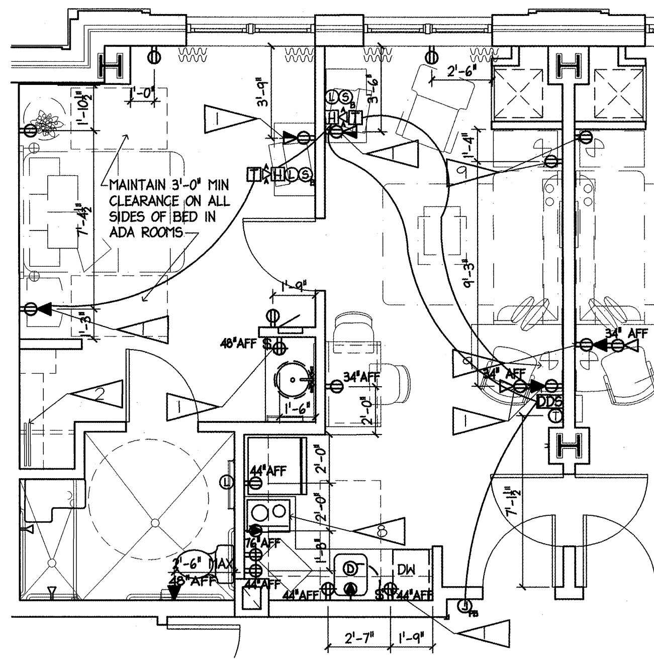
B I BEDROOM 4 ADA - ENLARGED POWER PLAN 1/4" = 1'-0"
