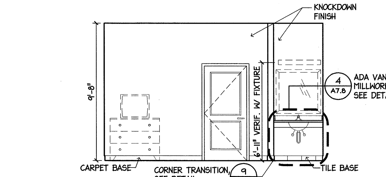
6 I BEDROOM 4 ADA ELEVATION 1/4" = 1'-0"
