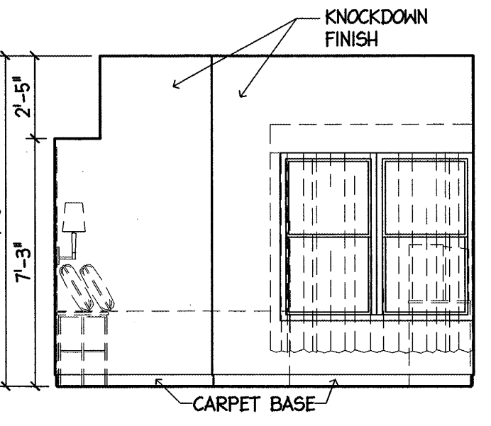
5 I BEDROOM 4 ADA ELEVATION 1/4" = 1'-0"
