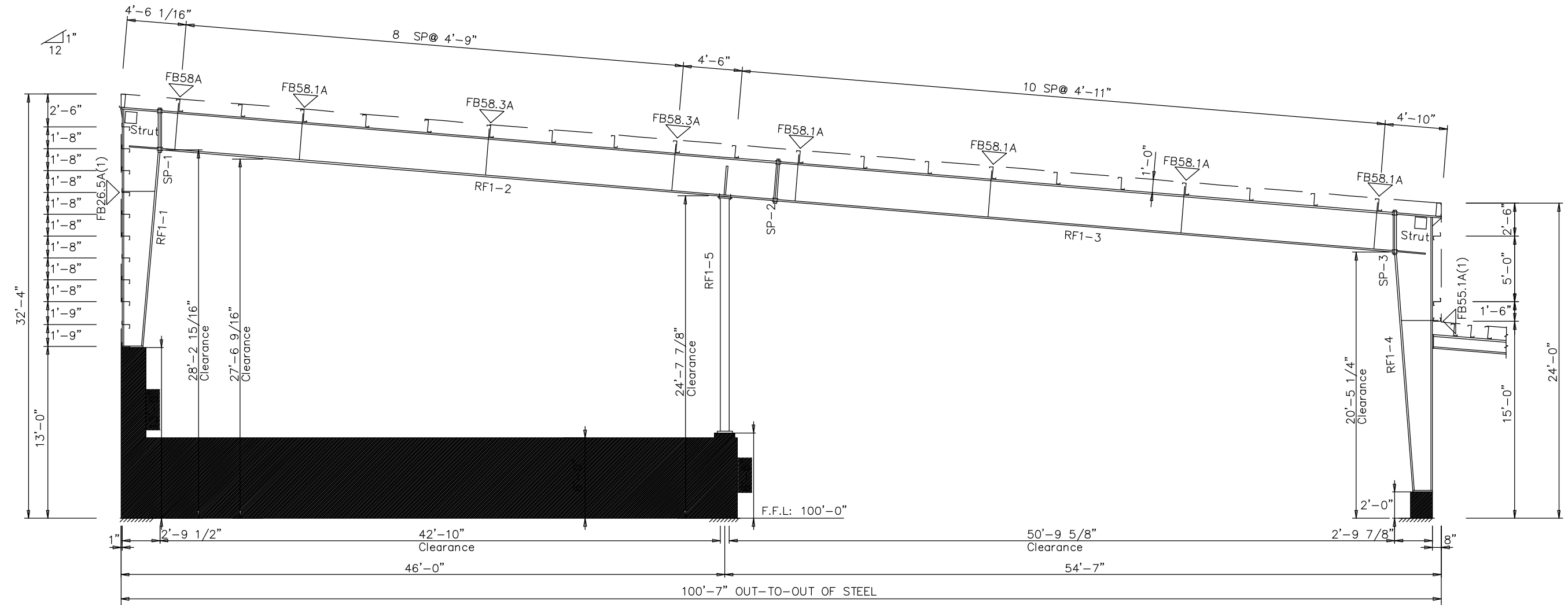
UFRAME CROSS SECTION FOR FRAME LINE 5
