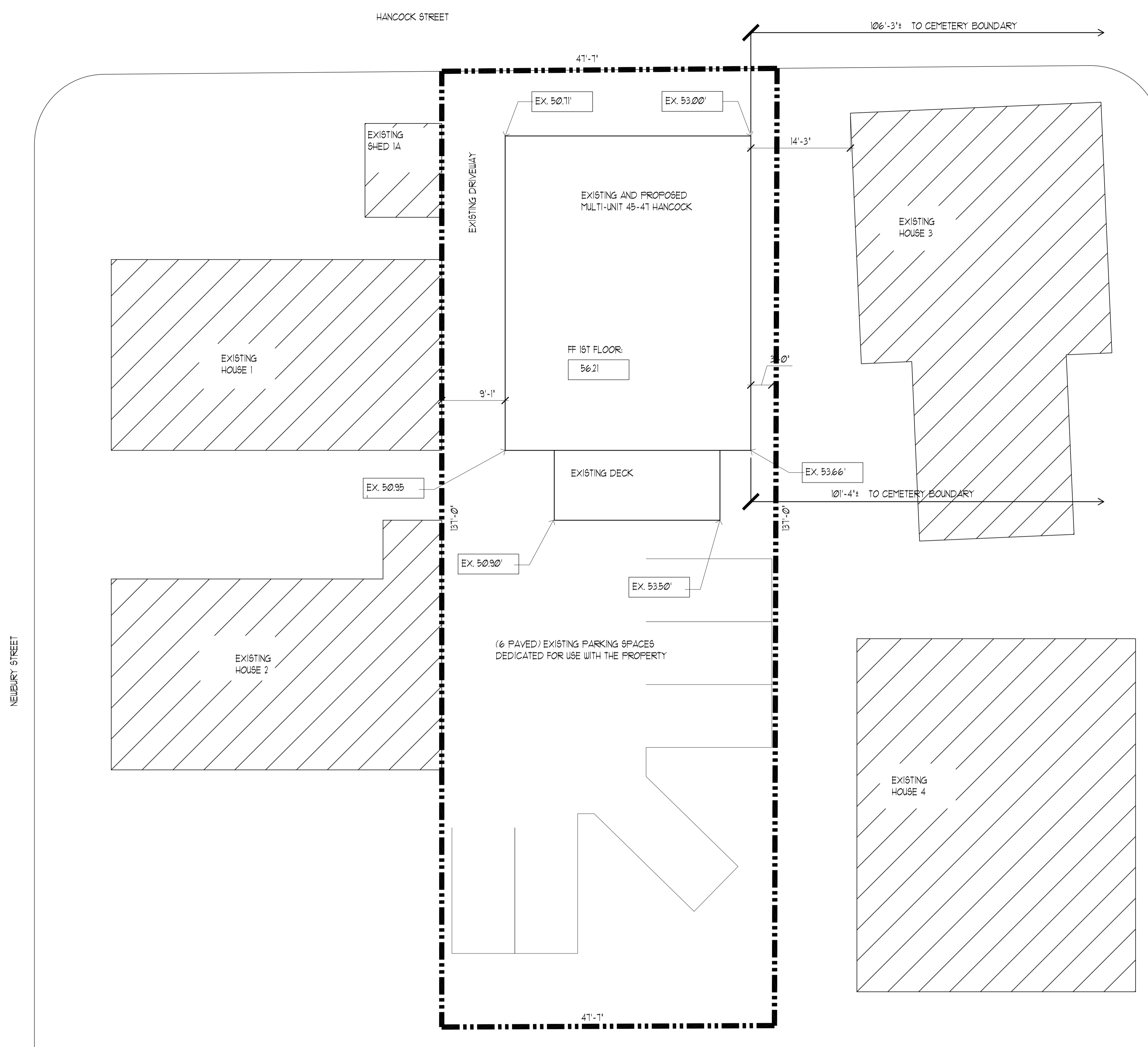
1 SITE PLAN - EXISTING CONDITIONS SCALE: 1/8" = 1'-0"
