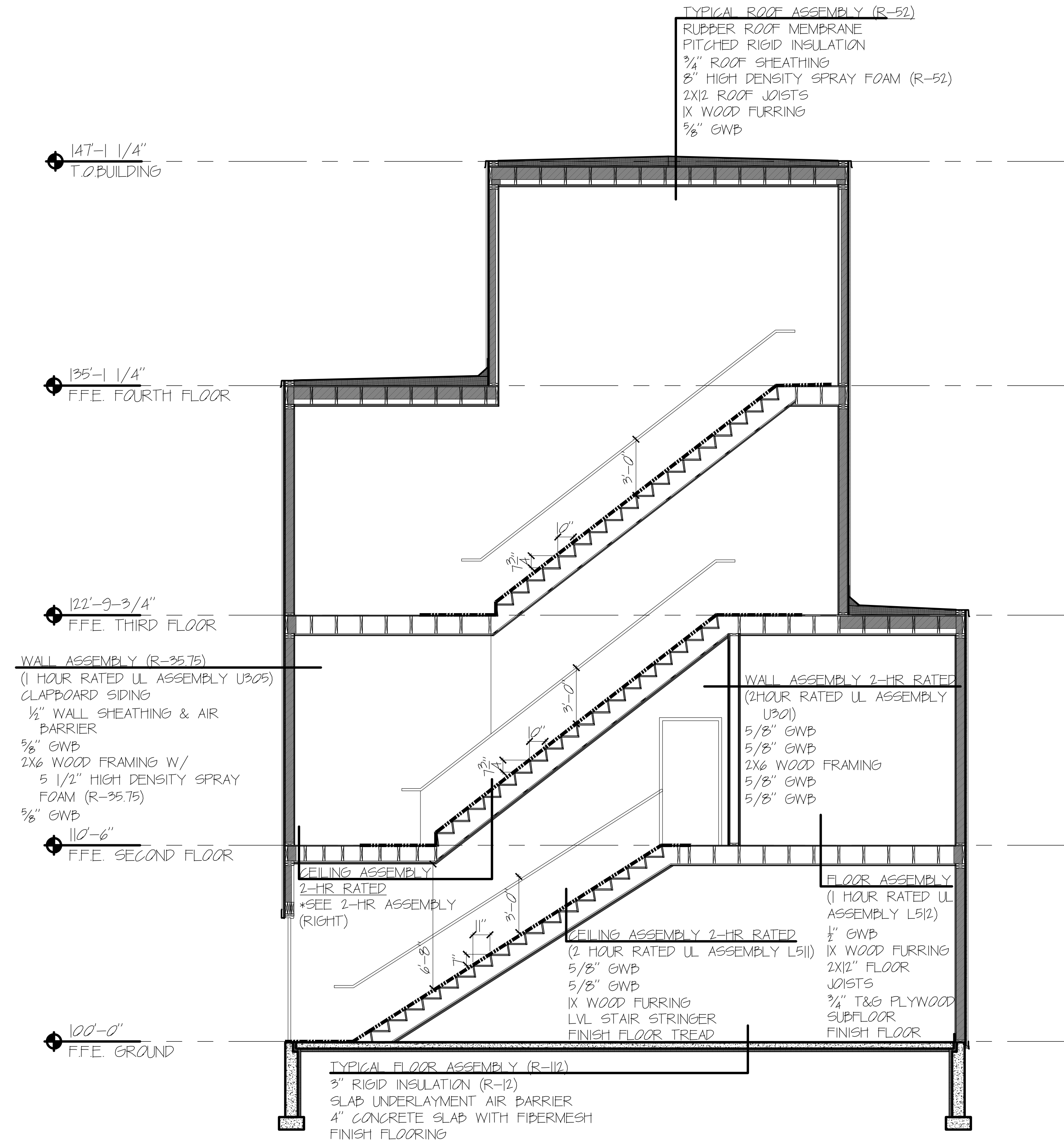
10 STAIR SECTION 0 4'-0" SCALE: 1/4" = 1'-0"
