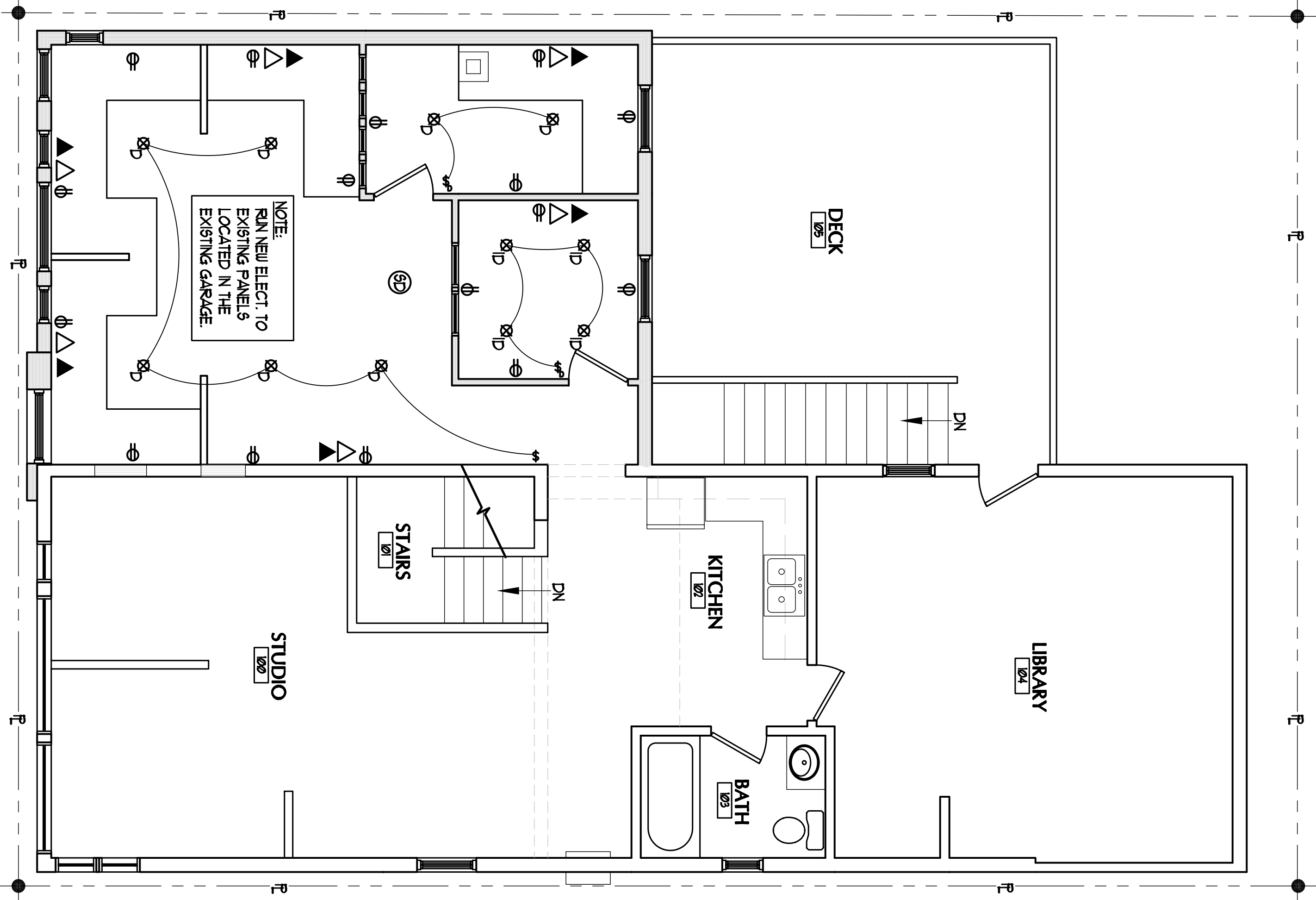
1 ELECTRICAL PLAN SCALE: 1/4" = 1'-0"
