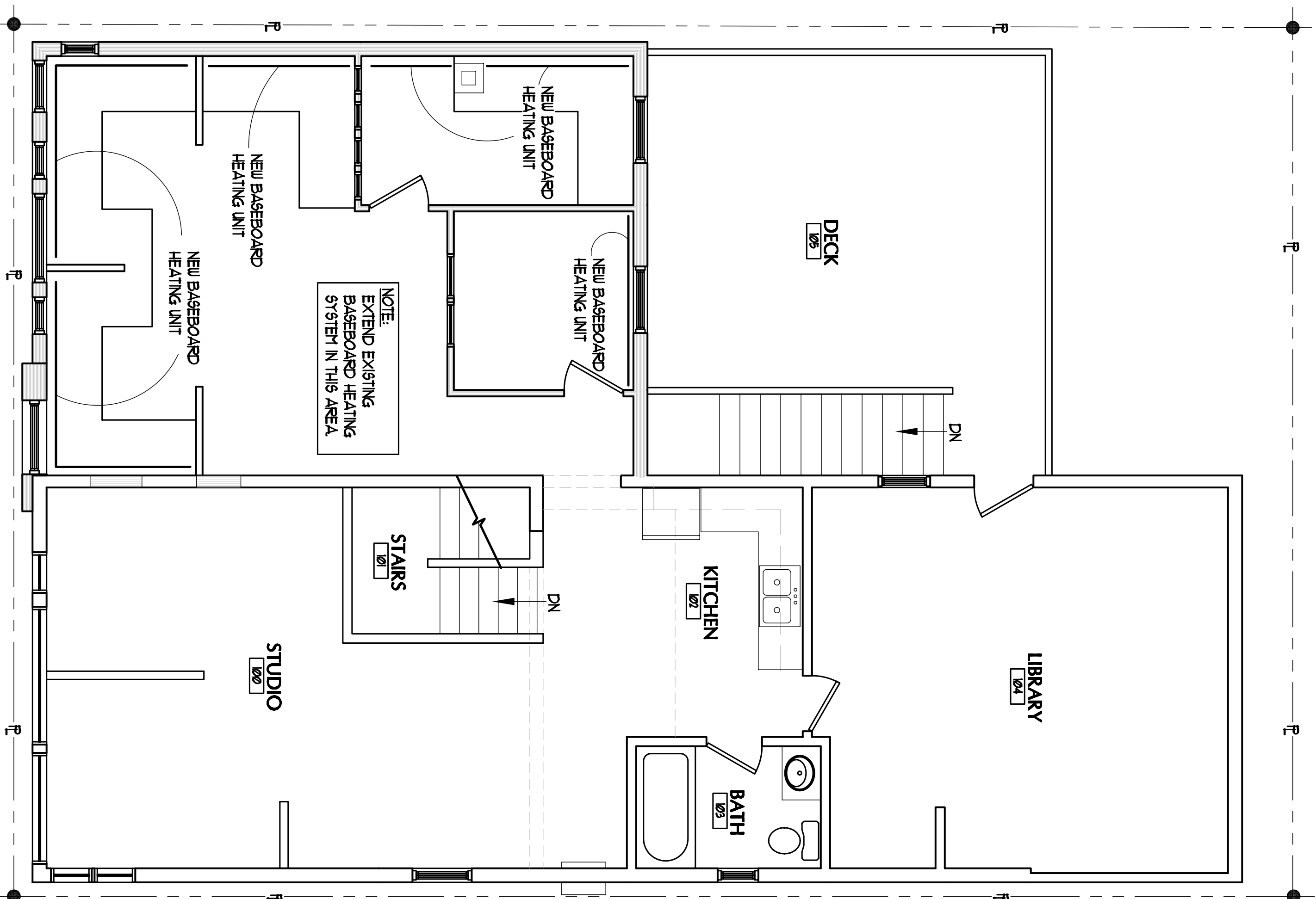
2 UTILITIES PLAN SCALE: 1/4" = 1'-0"
