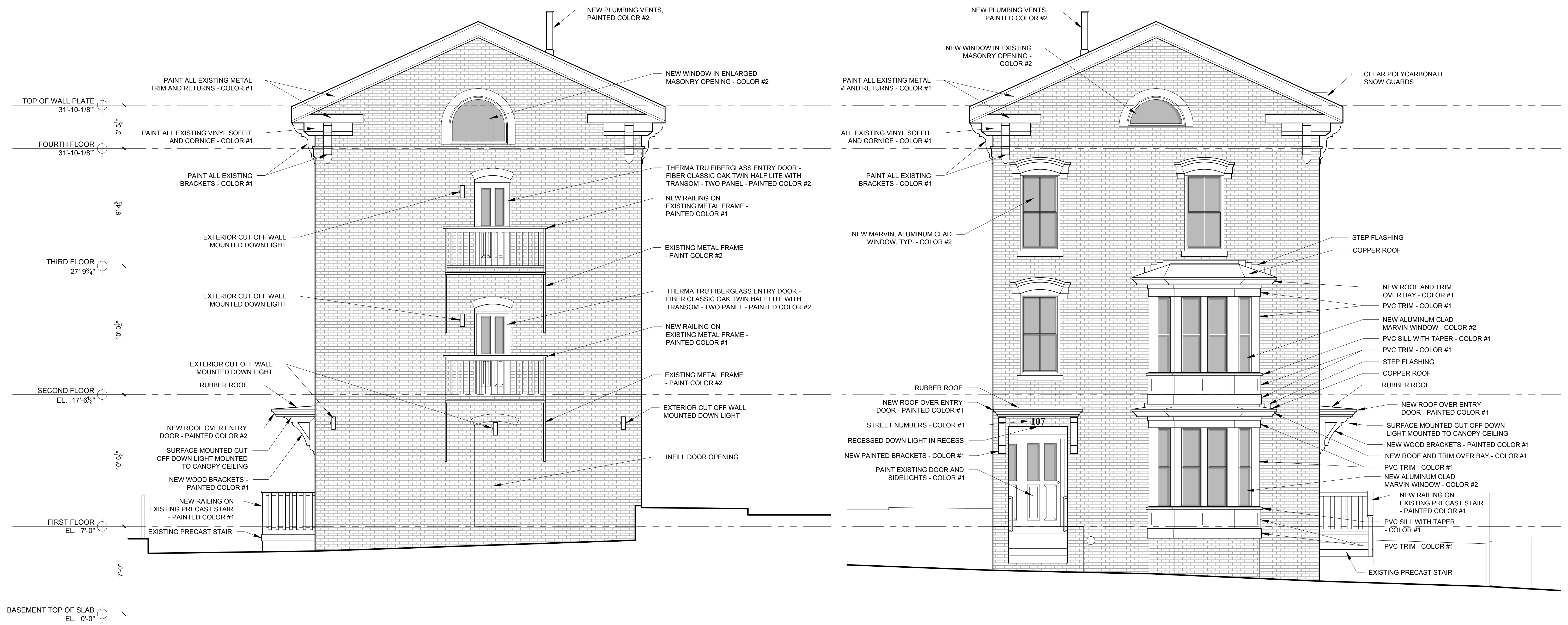
1 EAST ELEVATION 1/4" = 1'-0"
