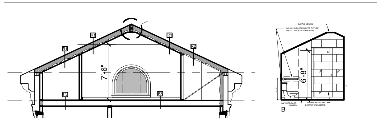
2 FOURTH FLOOR CEILING HEIGHT SECTION 1/8" = 1'-0"
