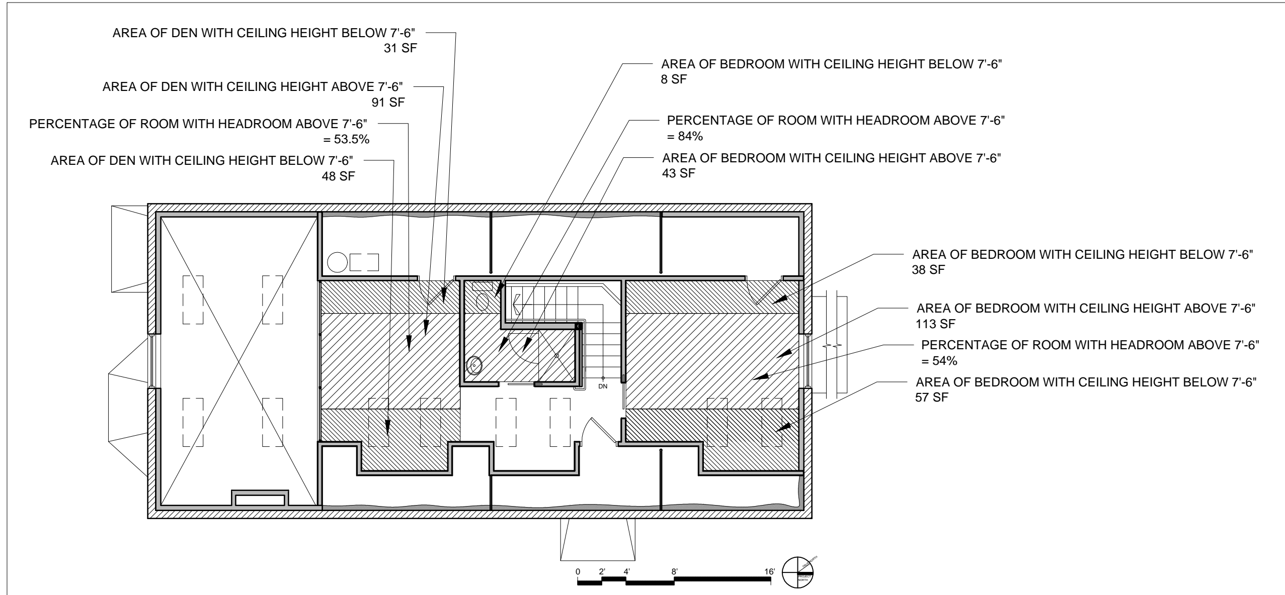
3 FOURTH FLOOR CEILING HEIGHT PLAN 1/8" = 1'-0"
