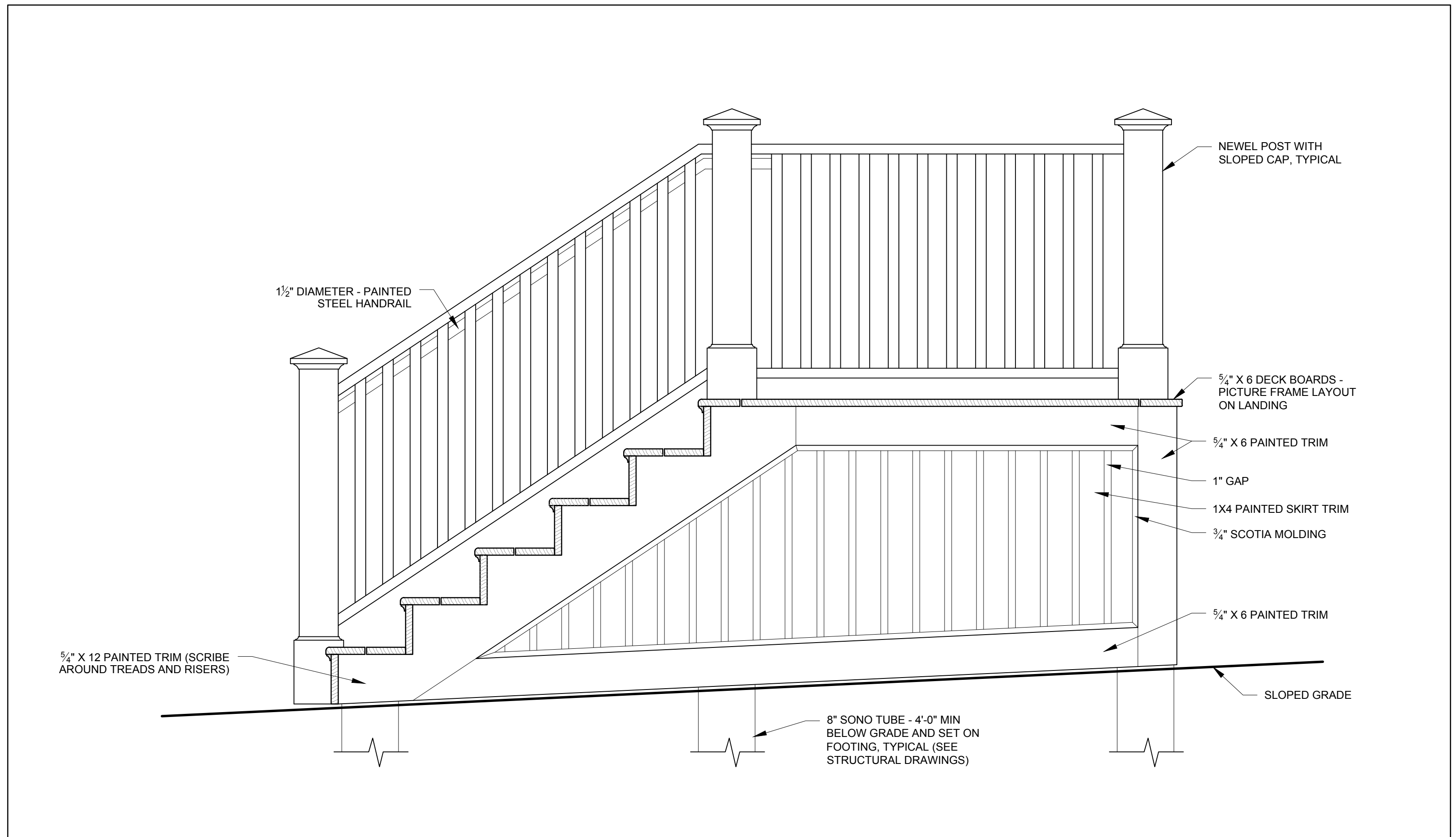
2 ELEVATION OF EXTERIOR WOOD STAIR 1" = 1'-0"
