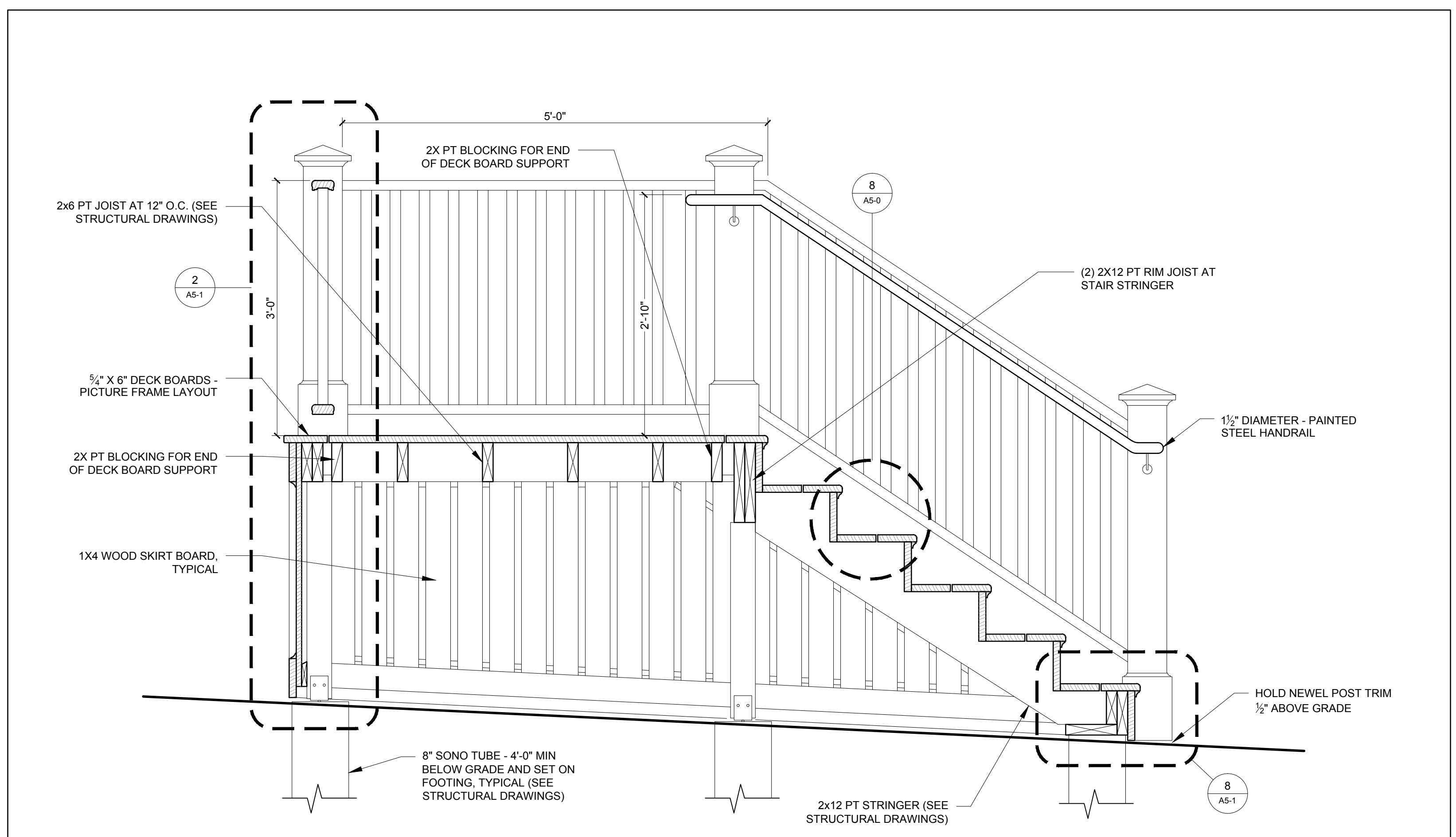
1 SECTION DETAIL OF EXTERIOR WOOD STAIR 1" = 1'-0"
