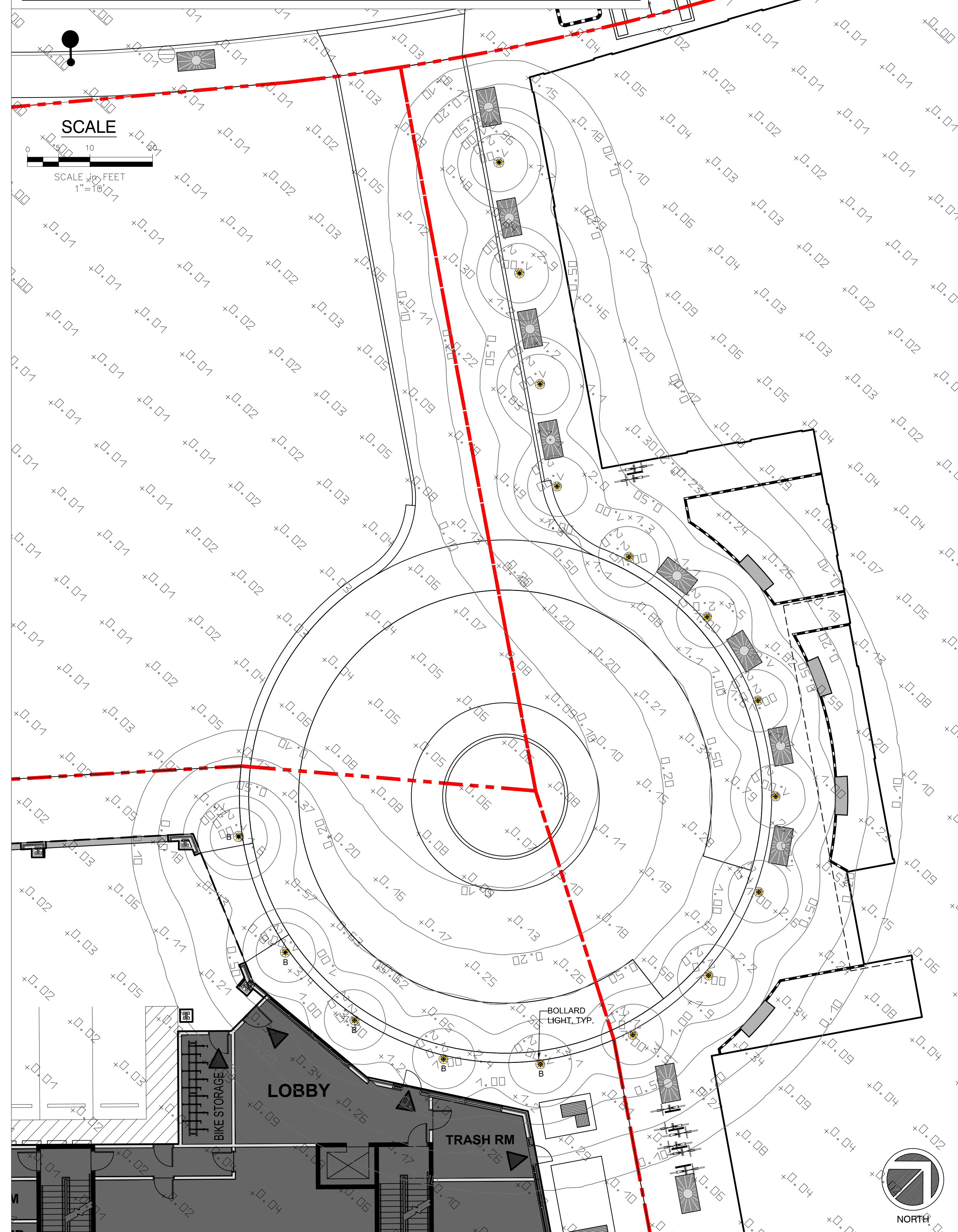
② COMBINED 20 THAMES STREET + AC HOTEL INTERNAL PHOTOMETRIC PLAN
