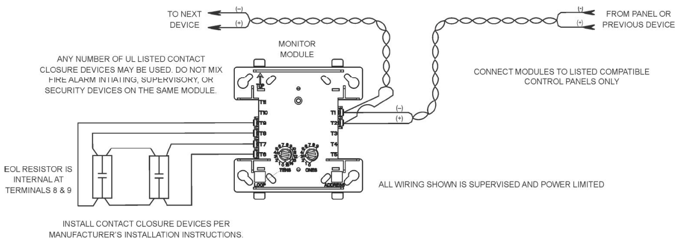
Typical Wiring for IDP-Monitor Module, NFFA Style D
