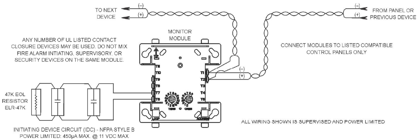
Typical Wiring for IDP-Monitor Module, NFFA Style B
