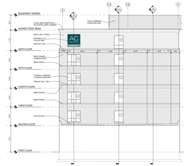
SOUTH LEVELS 2-6 EXTERIOR ELEVATION 6'-9 11/16"
