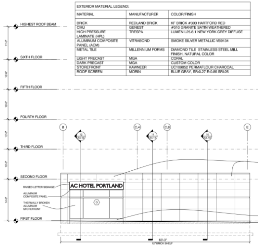
SOUTH LEVEL 1 EXTERIOR ELEVATION
