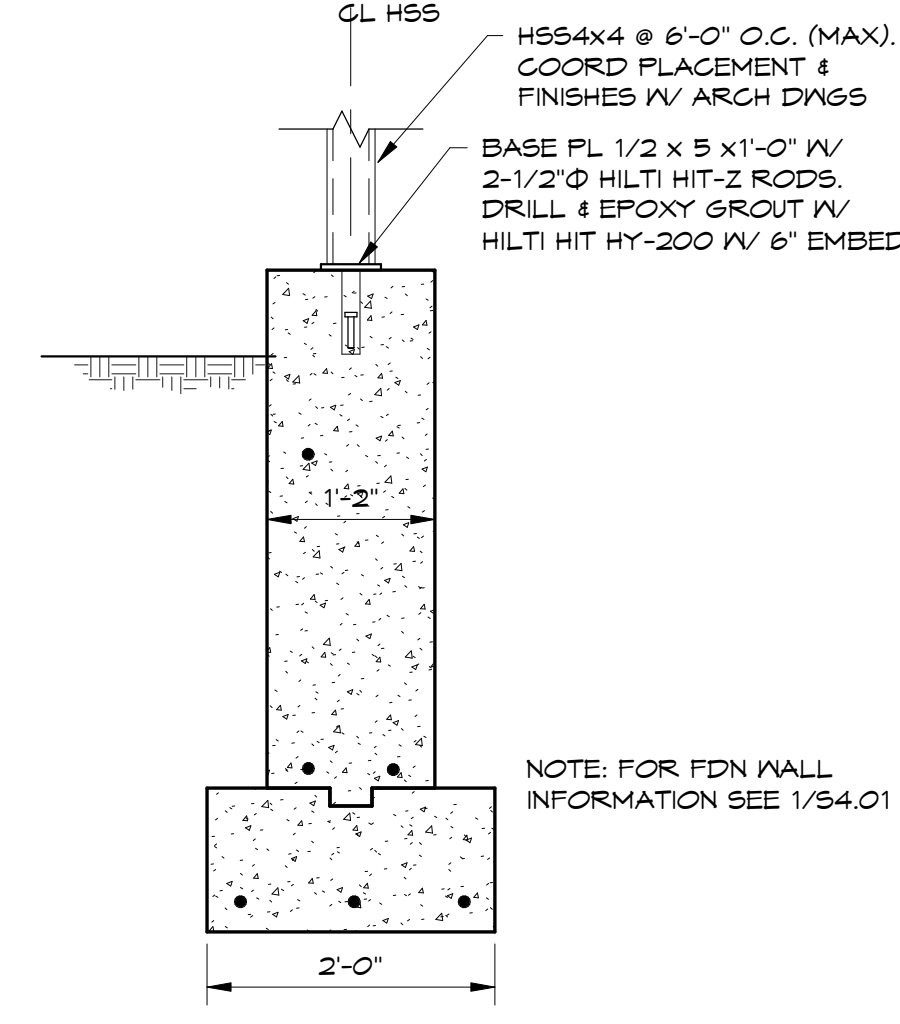
2 SECTION S4.02 3/4" = 1'-0"
