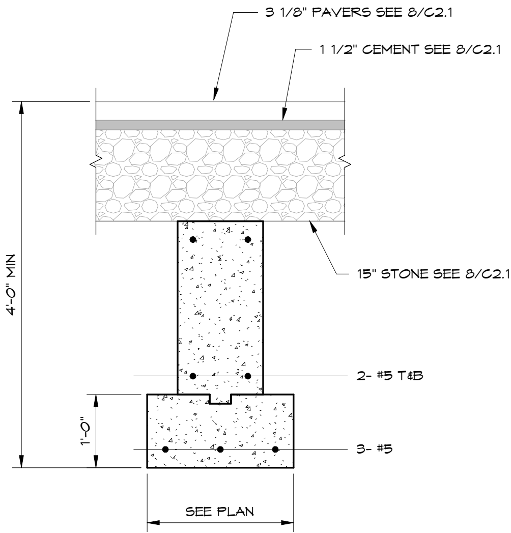
5 SECTION S4.02 3/4" = 1'-0"
