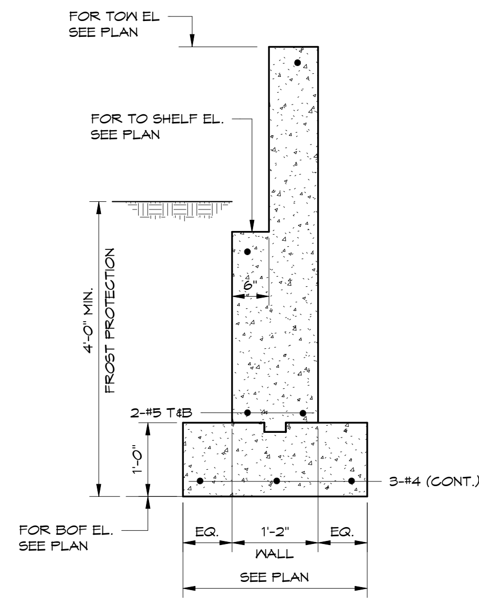
4 SECTION S4.02 3/4" = 1'-0"
