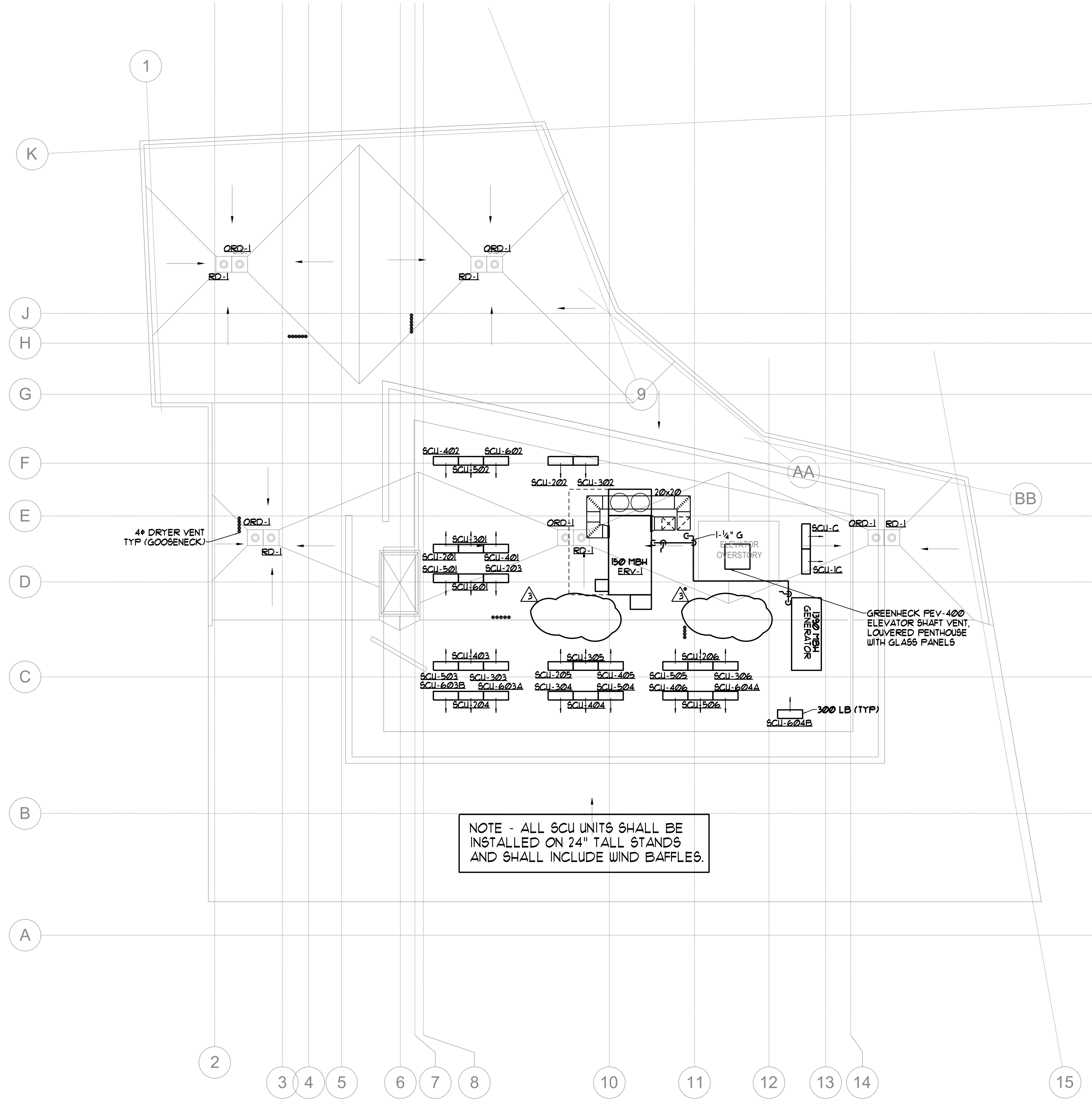
ROOF MECHANICAL PLAN SCALE - 1/8" = 1'-0"
