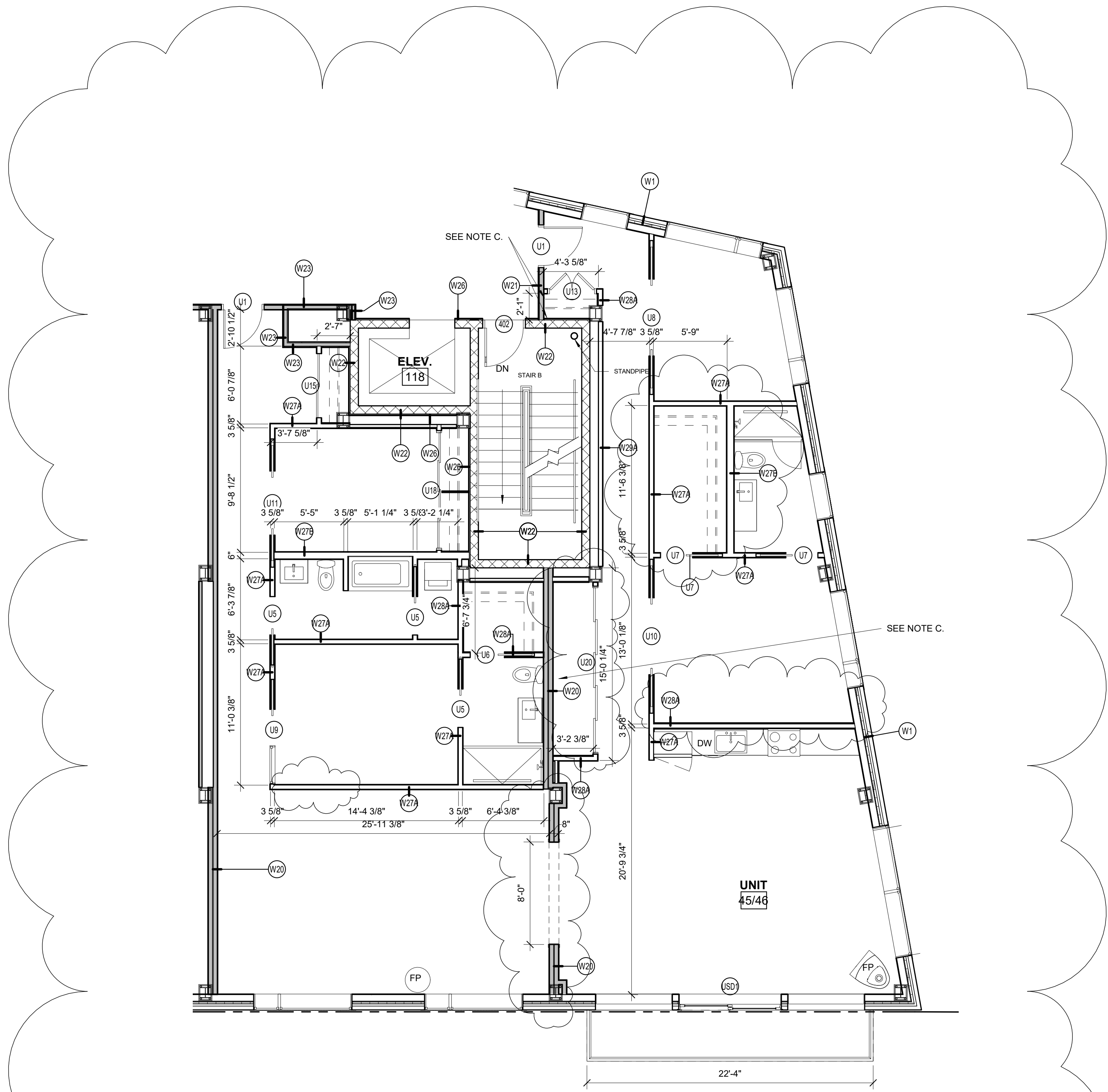
1 | ENLARGED UNIT 45/46 3/16" = 1'-0"
