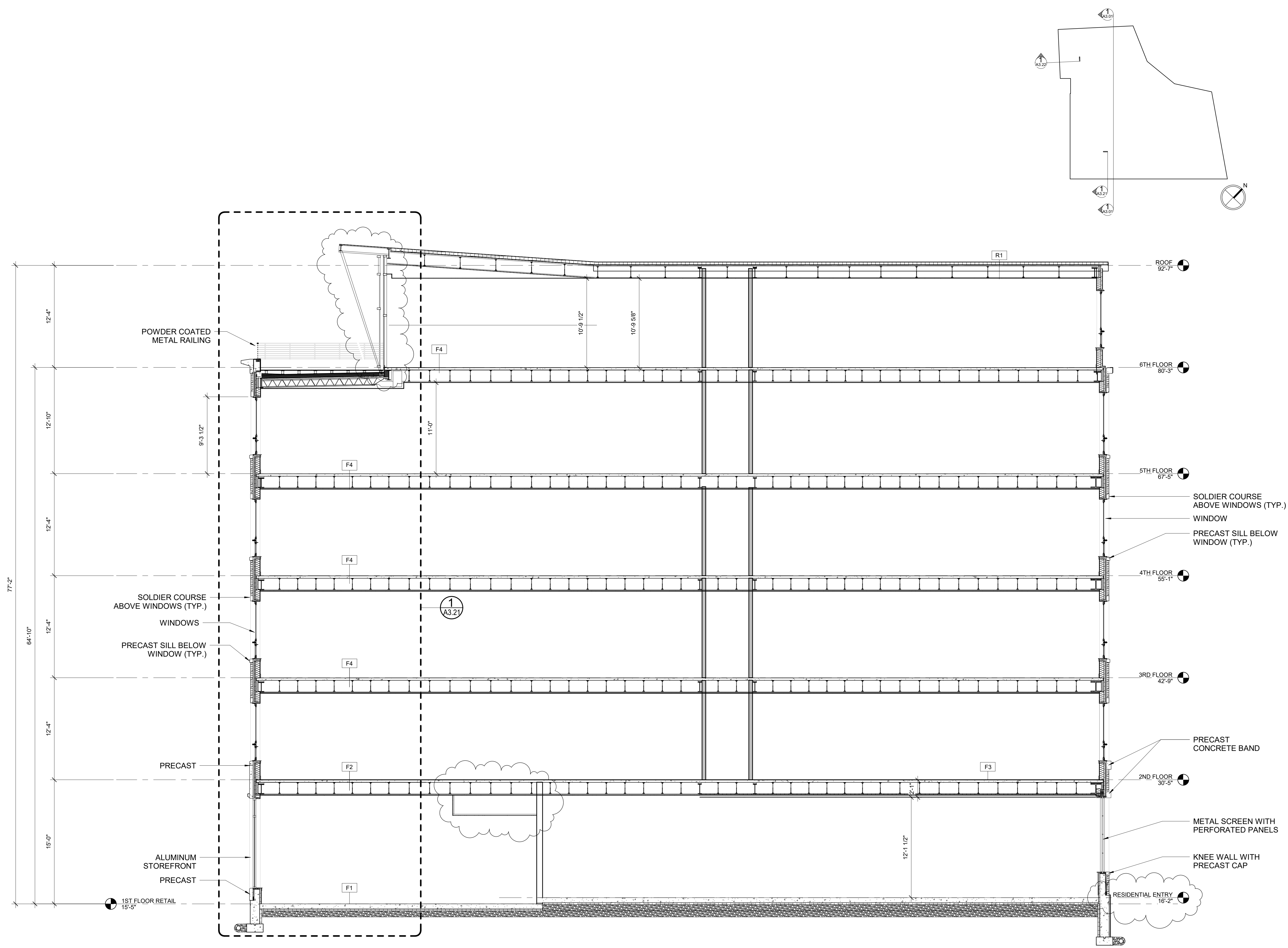
1 | BUILDING SECTION 3/16" = 1'-0"
