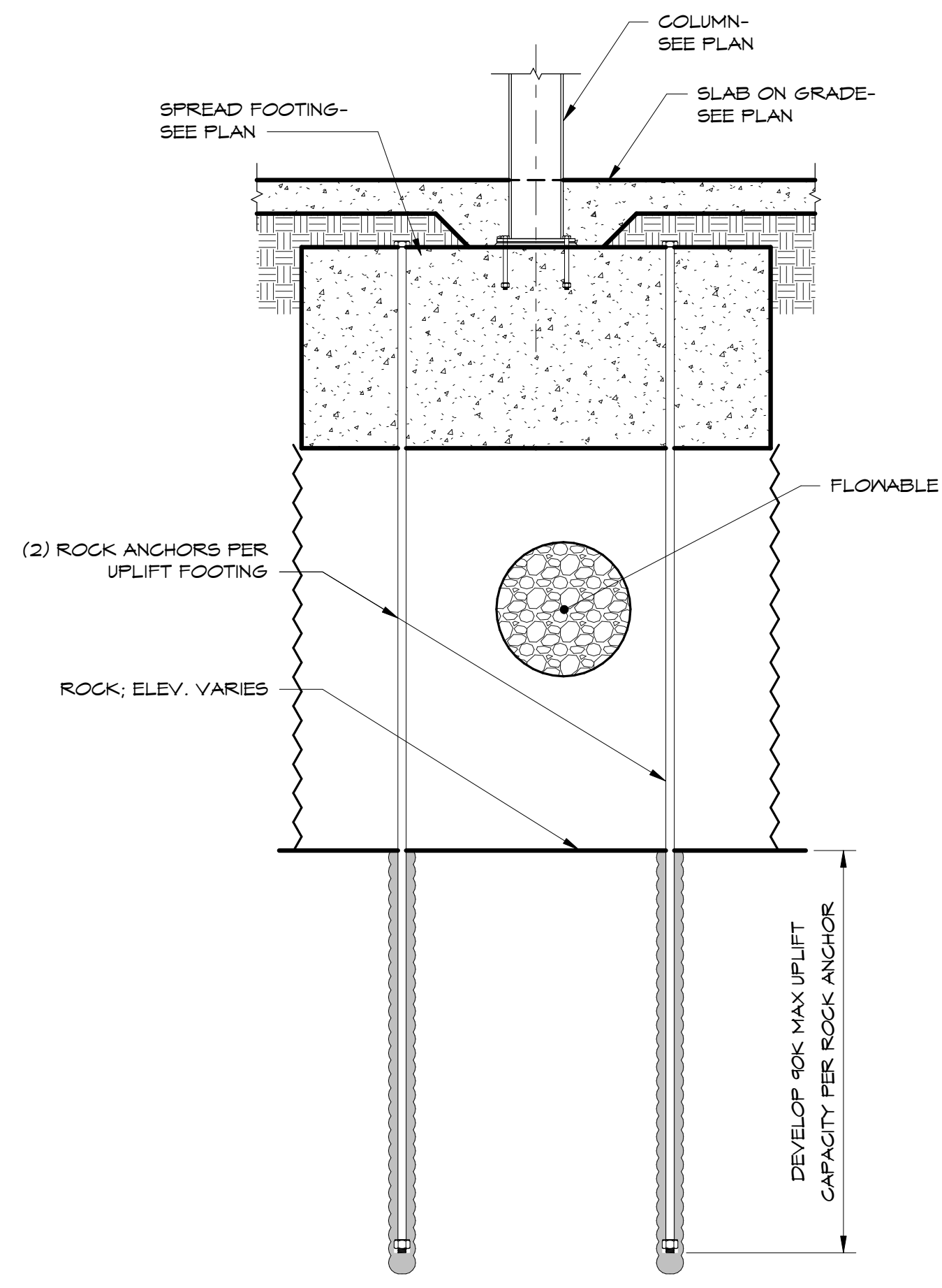
1 SECTION 1/2" = 1'-0"
