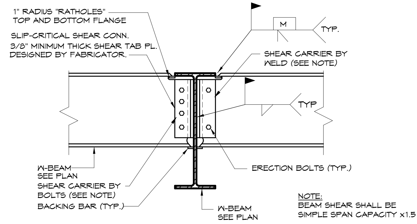
BEAM TO BEAM TYPICAL MOMENT CONNECTION
