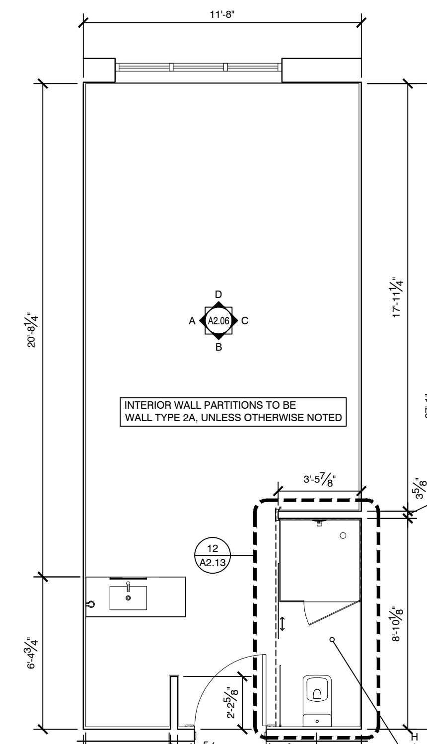
1 ARCHITECTURAL PLAN 1/4" = 1'-0"
