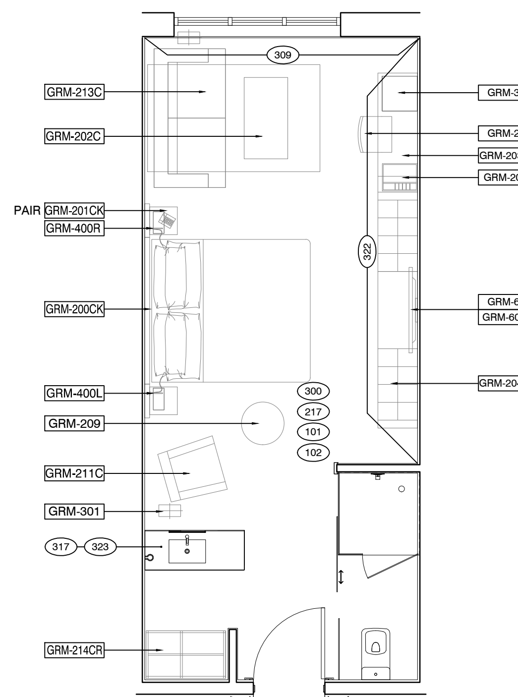
2 FURNITURE PLAN - METRO KING (RIGHT) 1/4" = 1'-0" RIGHT: 301, 352, 401, 452, 501, 552, 601, 652
