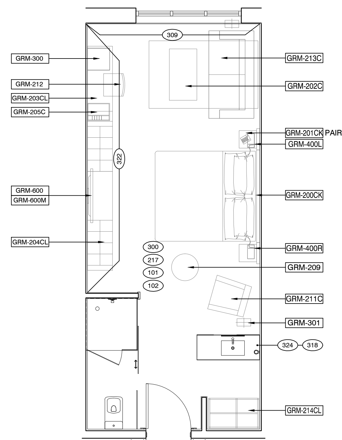
4 FURNITURE PLAN - METRO KING (LEFT) 1/4" = 1'-0" LEFT: 202, 251, 302, 351, 402, 451, 502, 551, 602, 651
