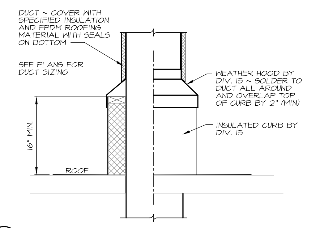
6 DUCTWORK PENETRATING ROOF NO SCALE
