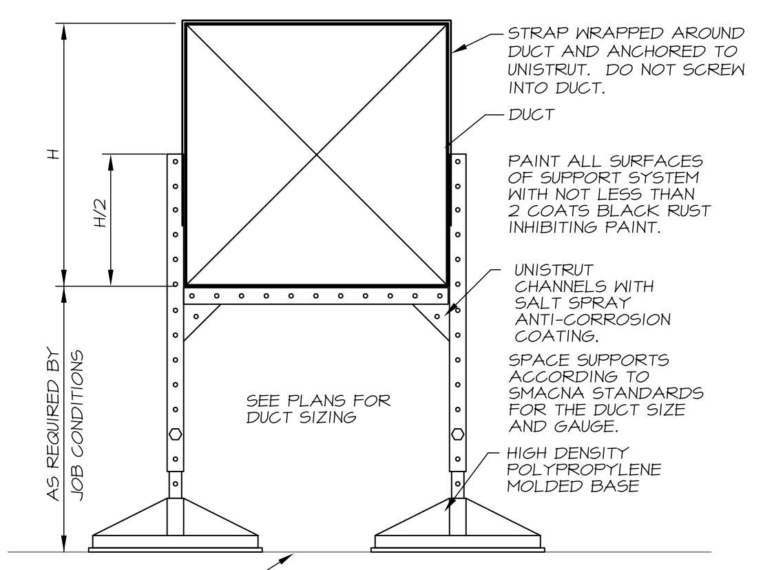
4 EXTERIOR DUCT SUPPORT NO SCALE
