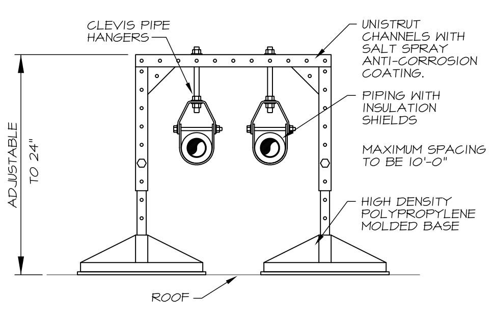
3 EXTERIOR PIPE SUPPORT SYSTEM NO SCALE
