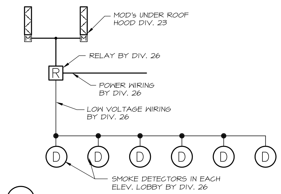
5 ELEVATOR SHAFT VENTING NO SCALE
