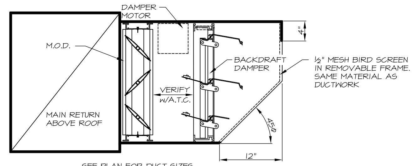
2 RTU-4 RELIEF AIR DETAIL NO SCALE
