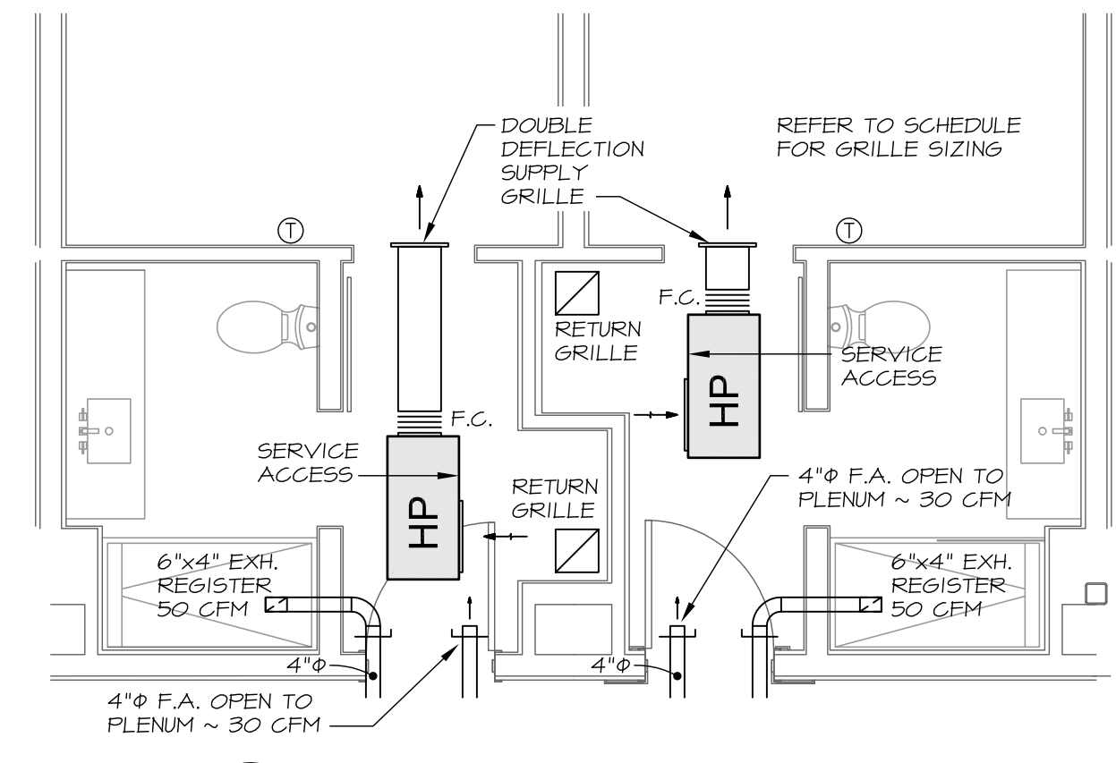
2 TYPICAL GUEST ROOM SCALE: 1/4" = 1'-0"
