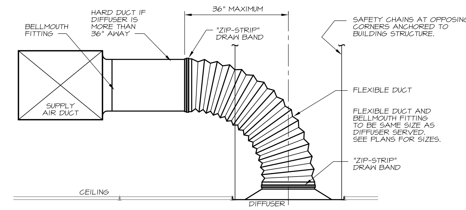
4 FLEXIBLE DUCT & DIFFUSER CONNECTION DETAIL NO SCALE
