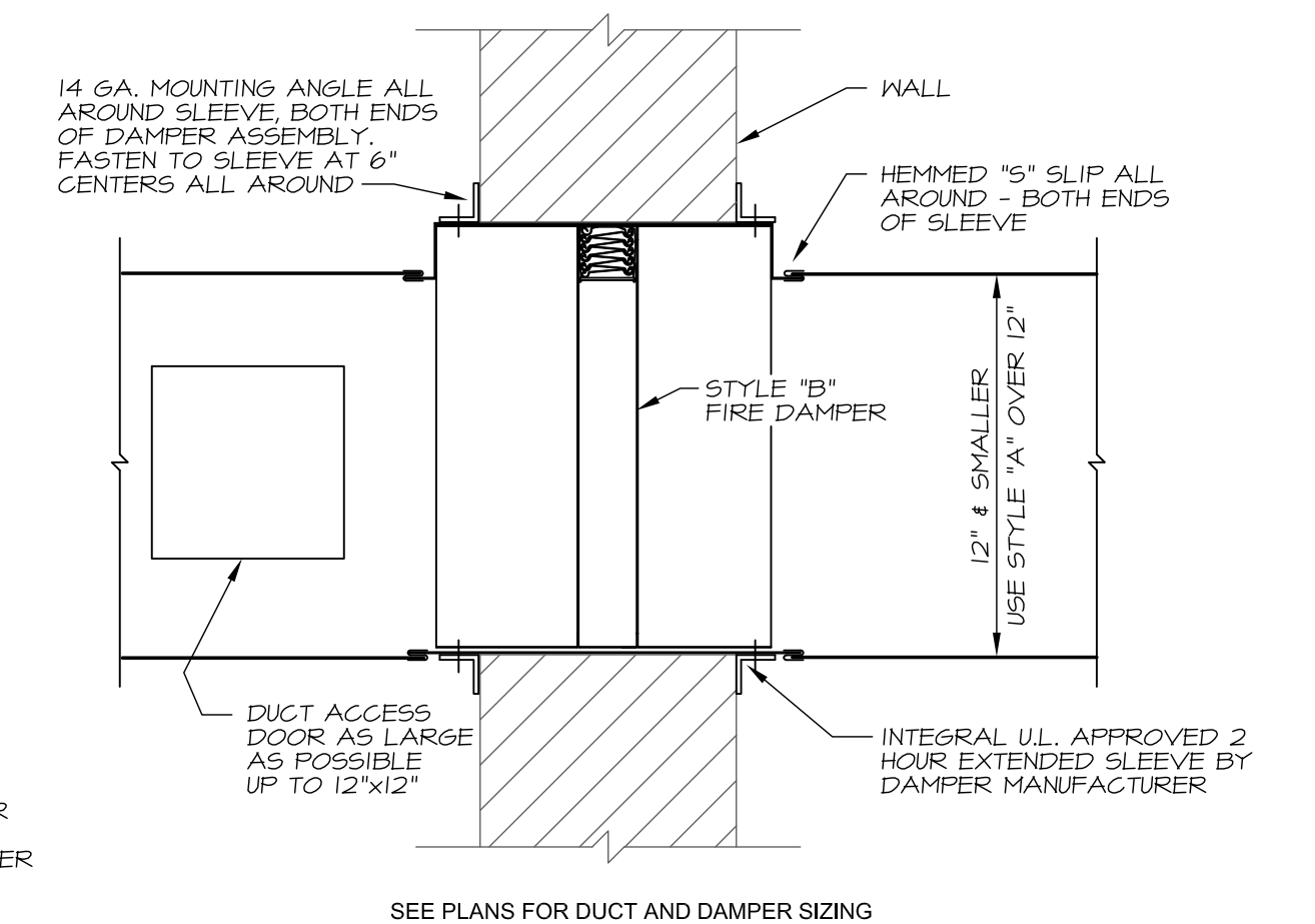
3 WALL FIRE DAMPER STYLE "B" NO SCALE
