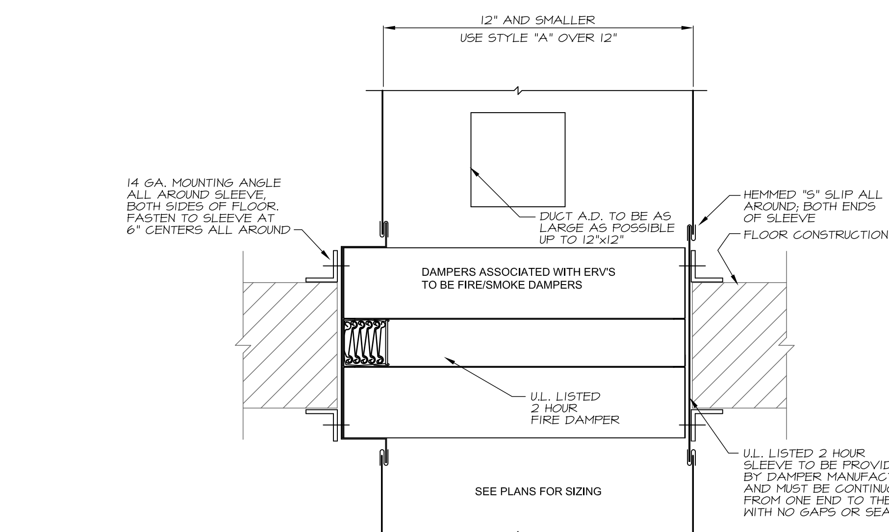
2 FLOOR FIRE DAMPER STYLE "B" NO SCALE
