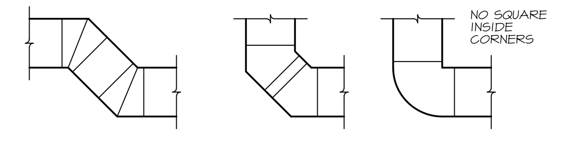
5 UNACCEPTABLE DUCT FITTINGS NO SCALE
