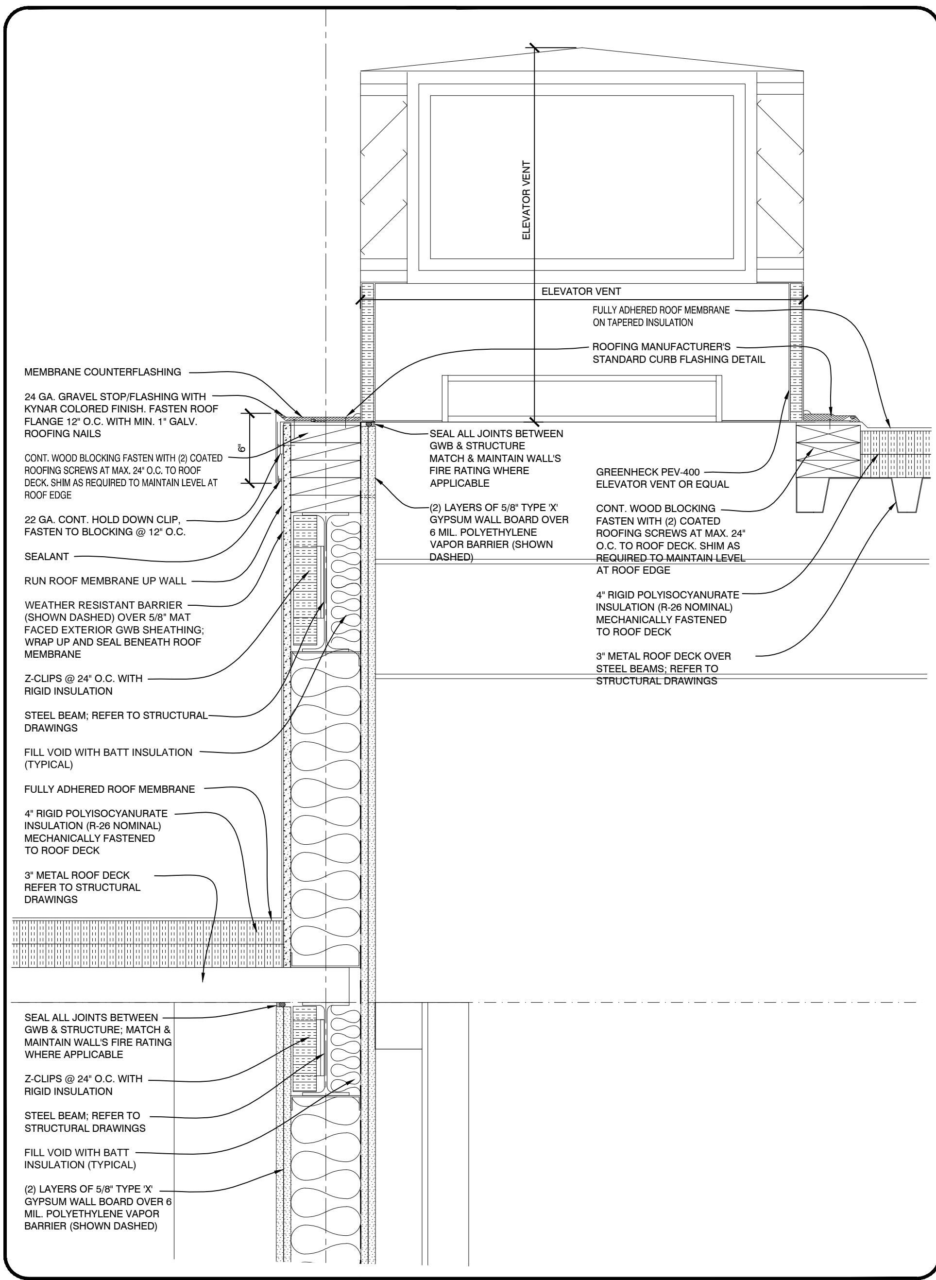
ELEVATOR ROOF VENT DETAIL
