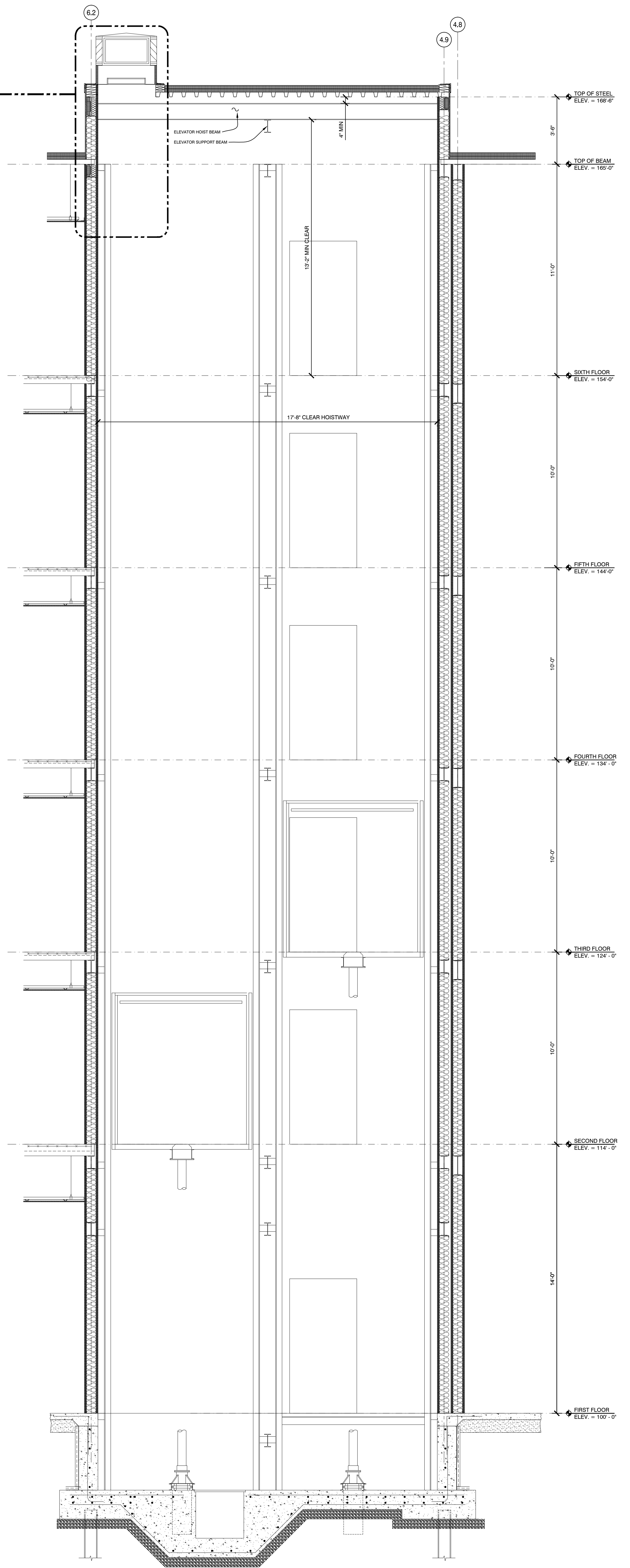
1 ELEVATOR SECTION
