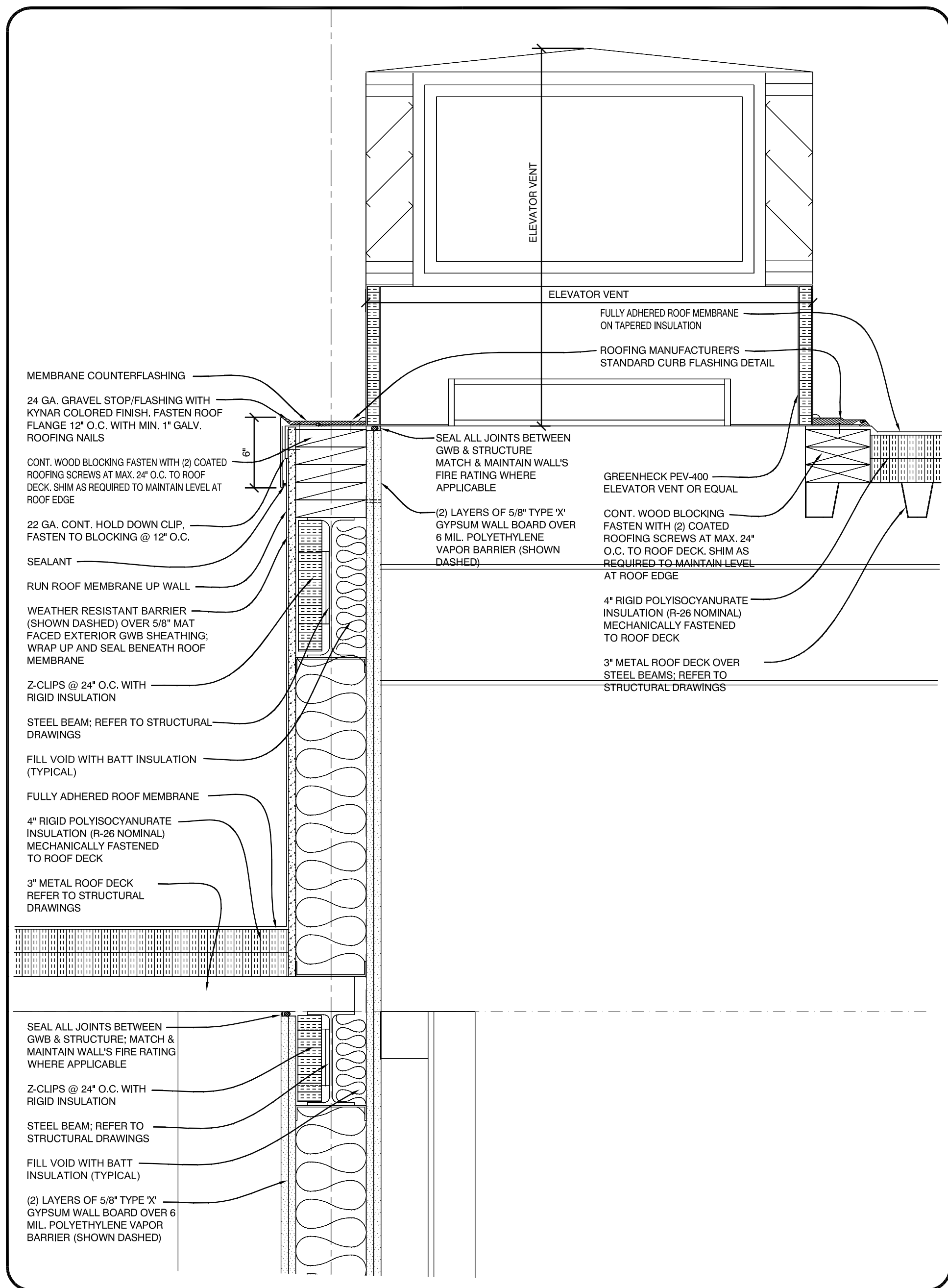
ELEVATOR ROOF VENT DETAIL 1 1/2" = 1'-0"
