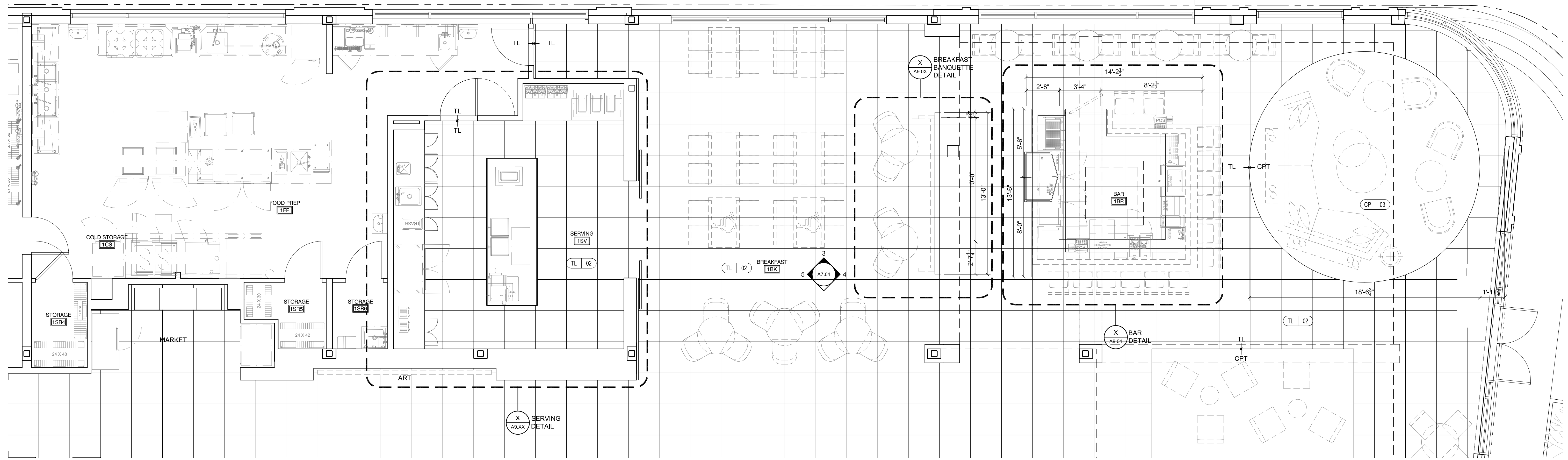
A ENLARGED FINISH PLAN - BREAKFAST & BAR SCALE: 1/4" = 1'-0"
