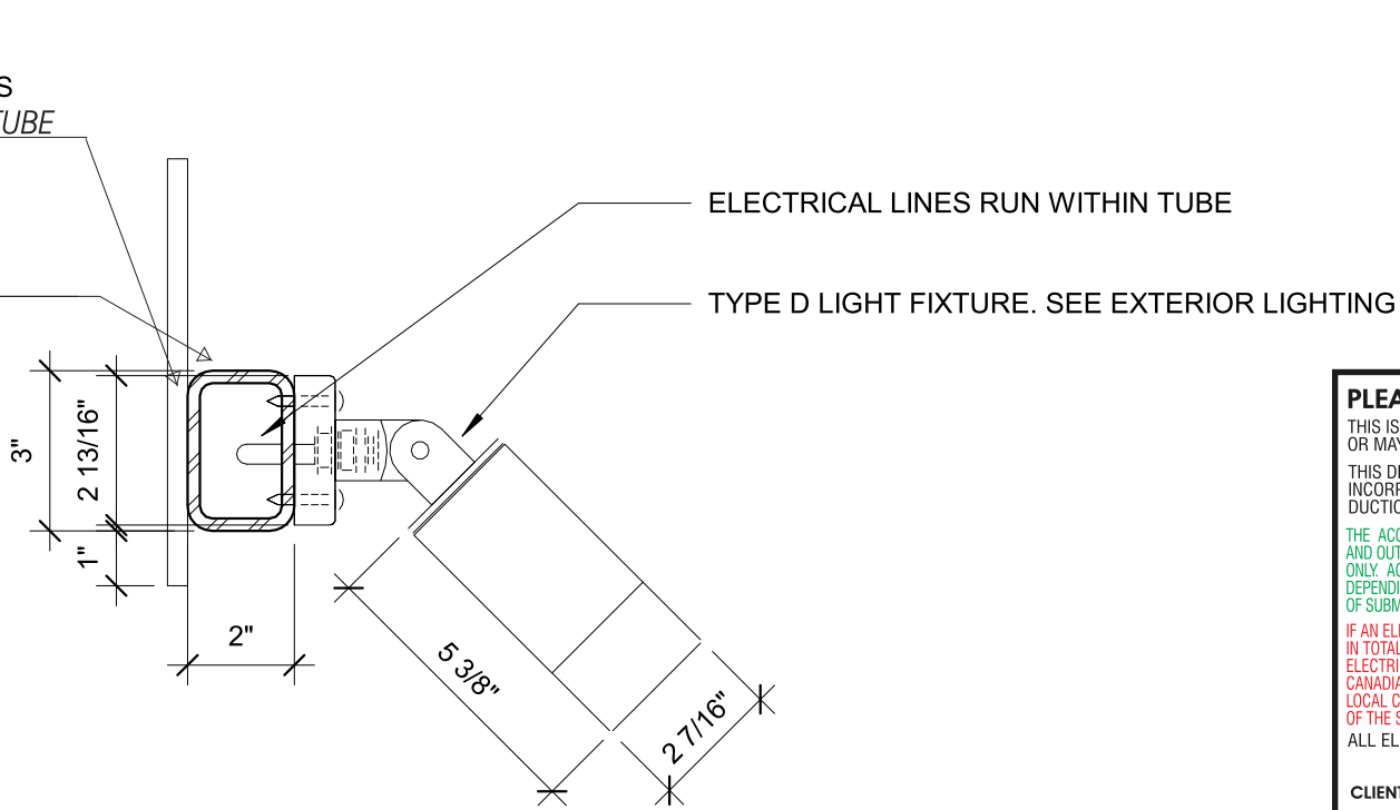
7 | ENTRANCE LIGHT FIXTURE DETAIL 3" = 1'-0"
