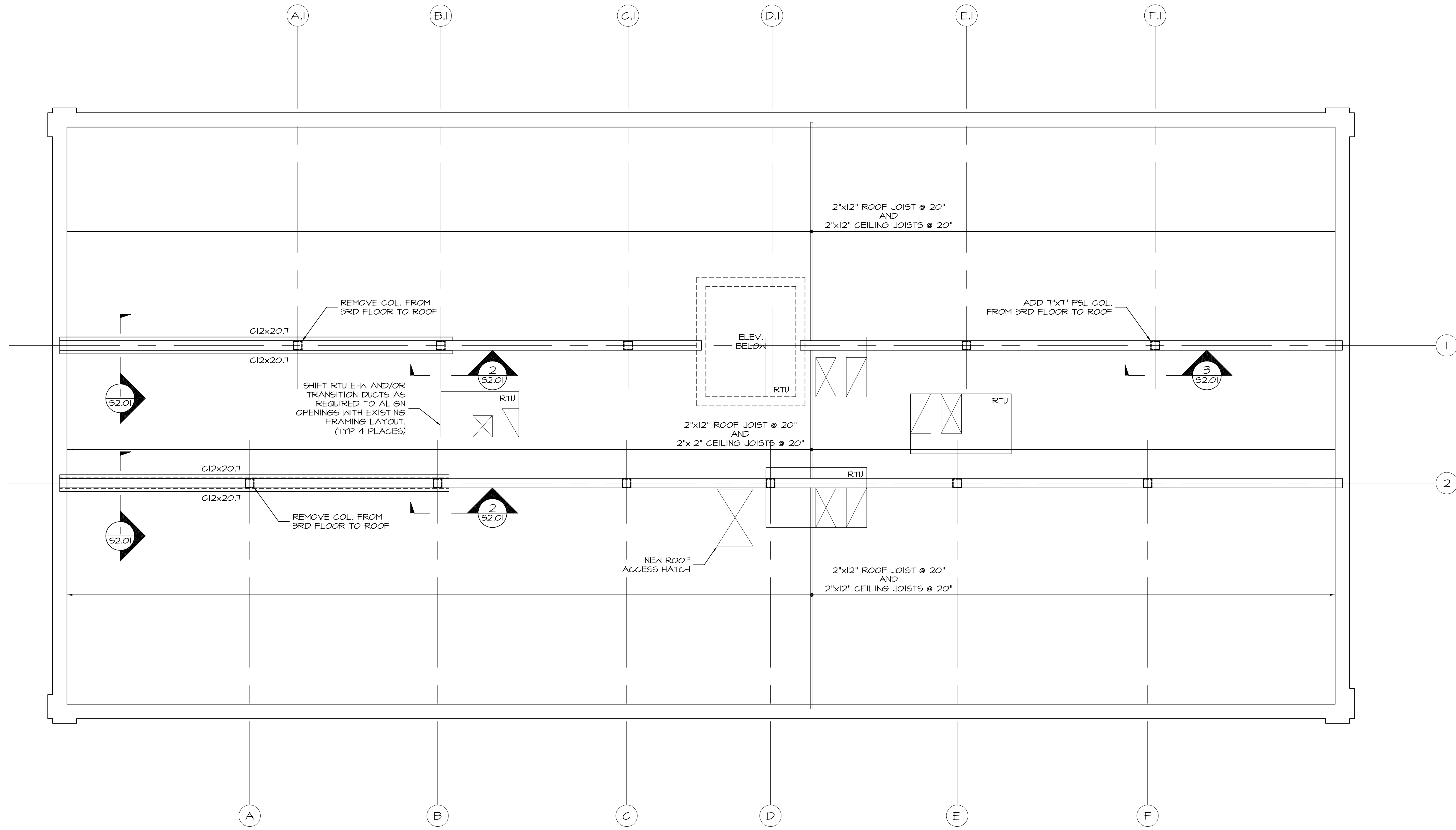
ROOF FRAMING PLAN 1/4"=1'-0"
