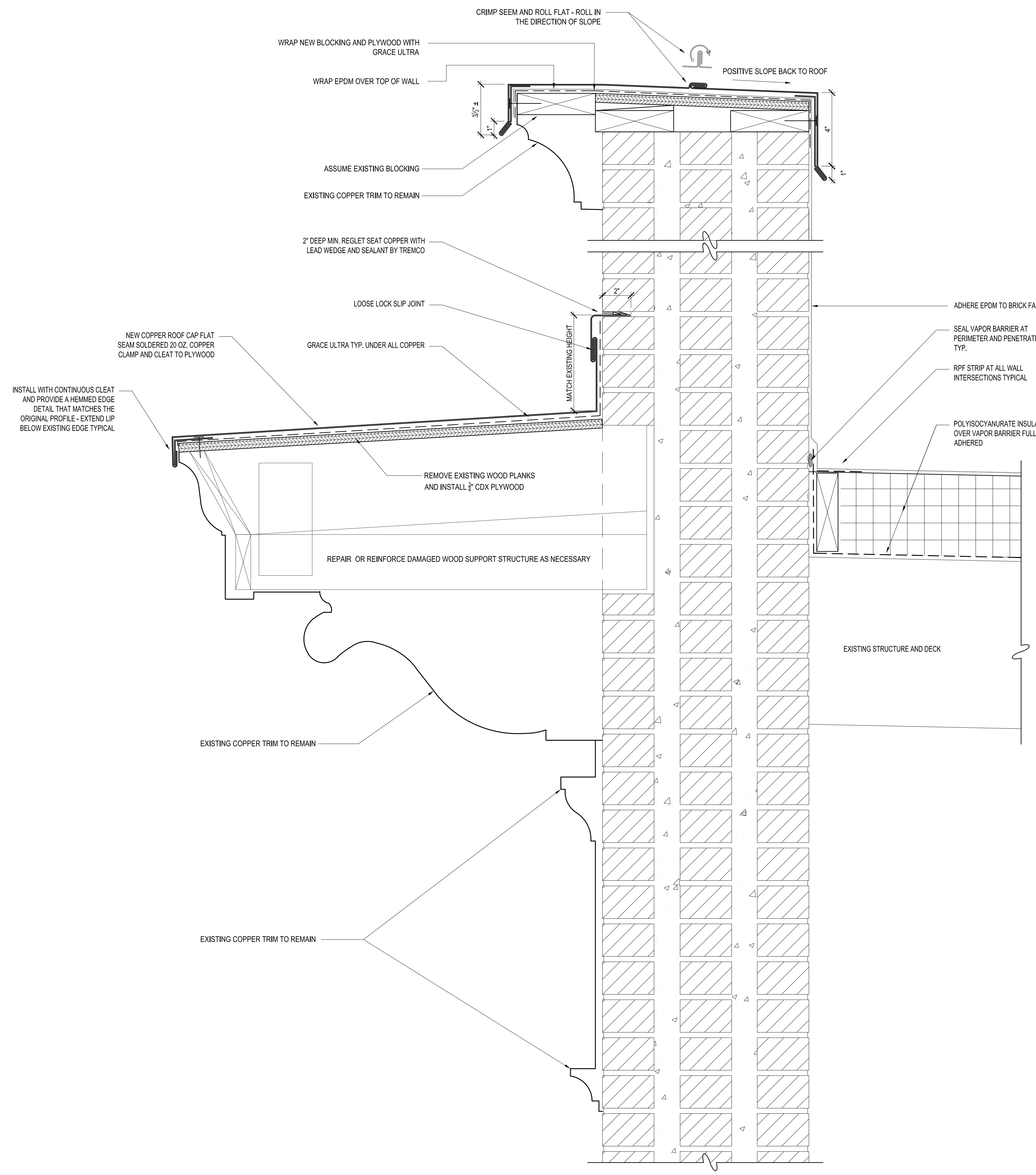
2 PARAPET WALL DETAIL
