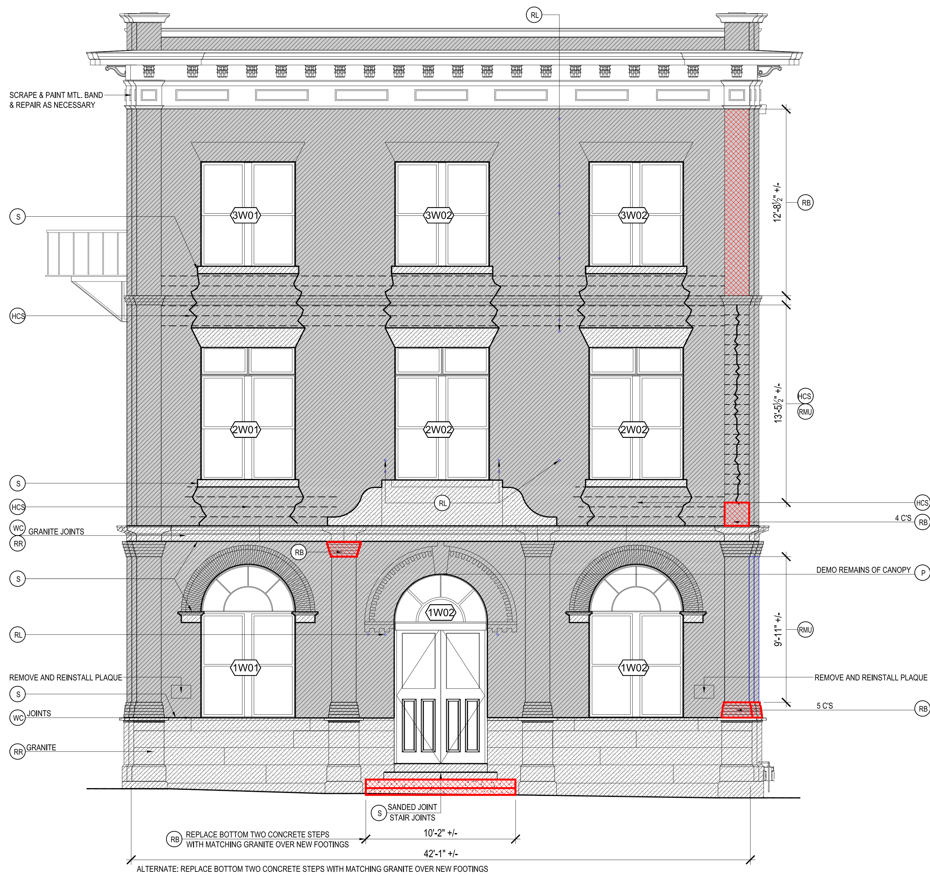
1 WEST ELEVATION
