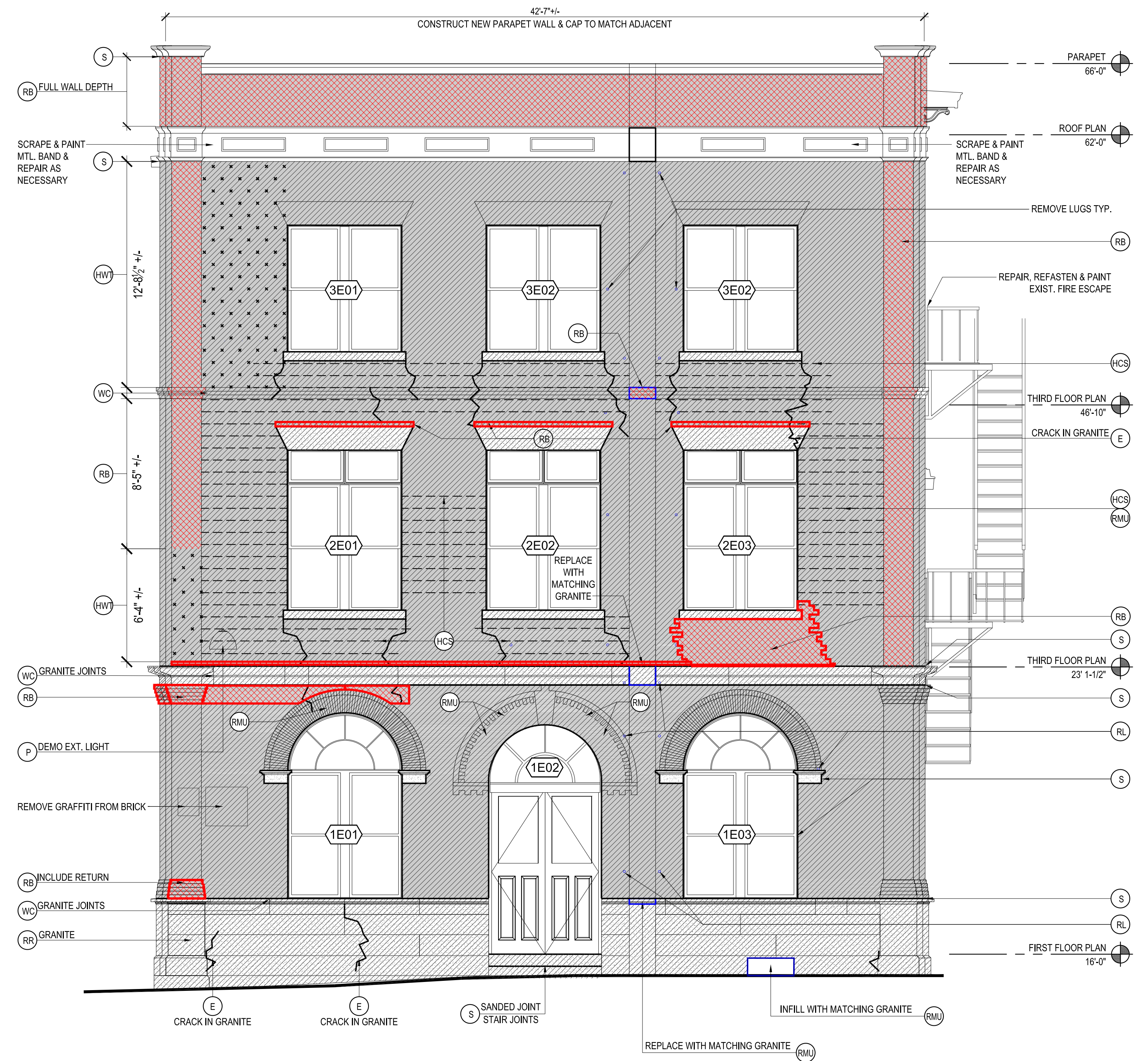
2 EAST ELEVATION
