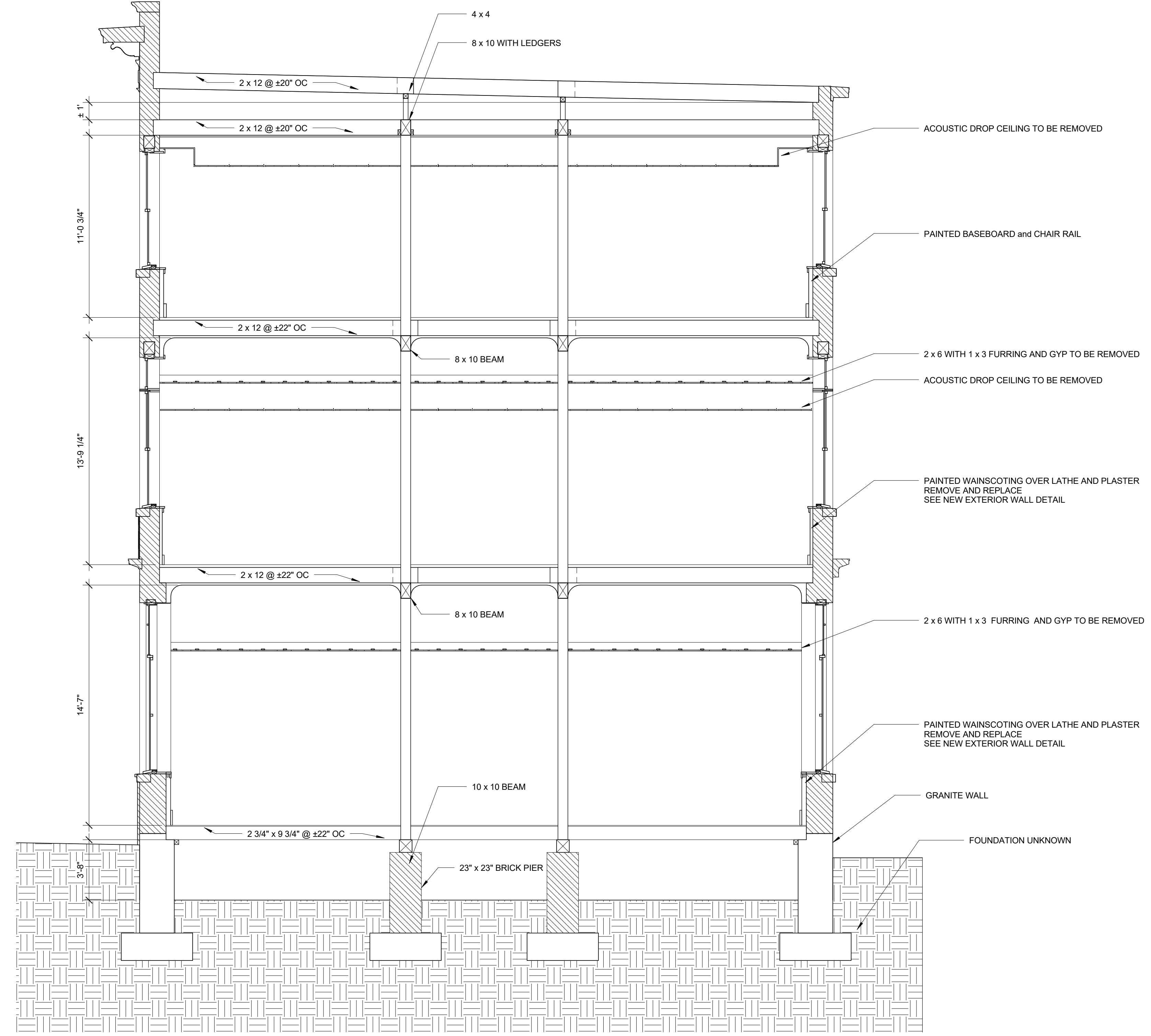
3 | EXISTING SECTION 1/4" = 1'-0"
