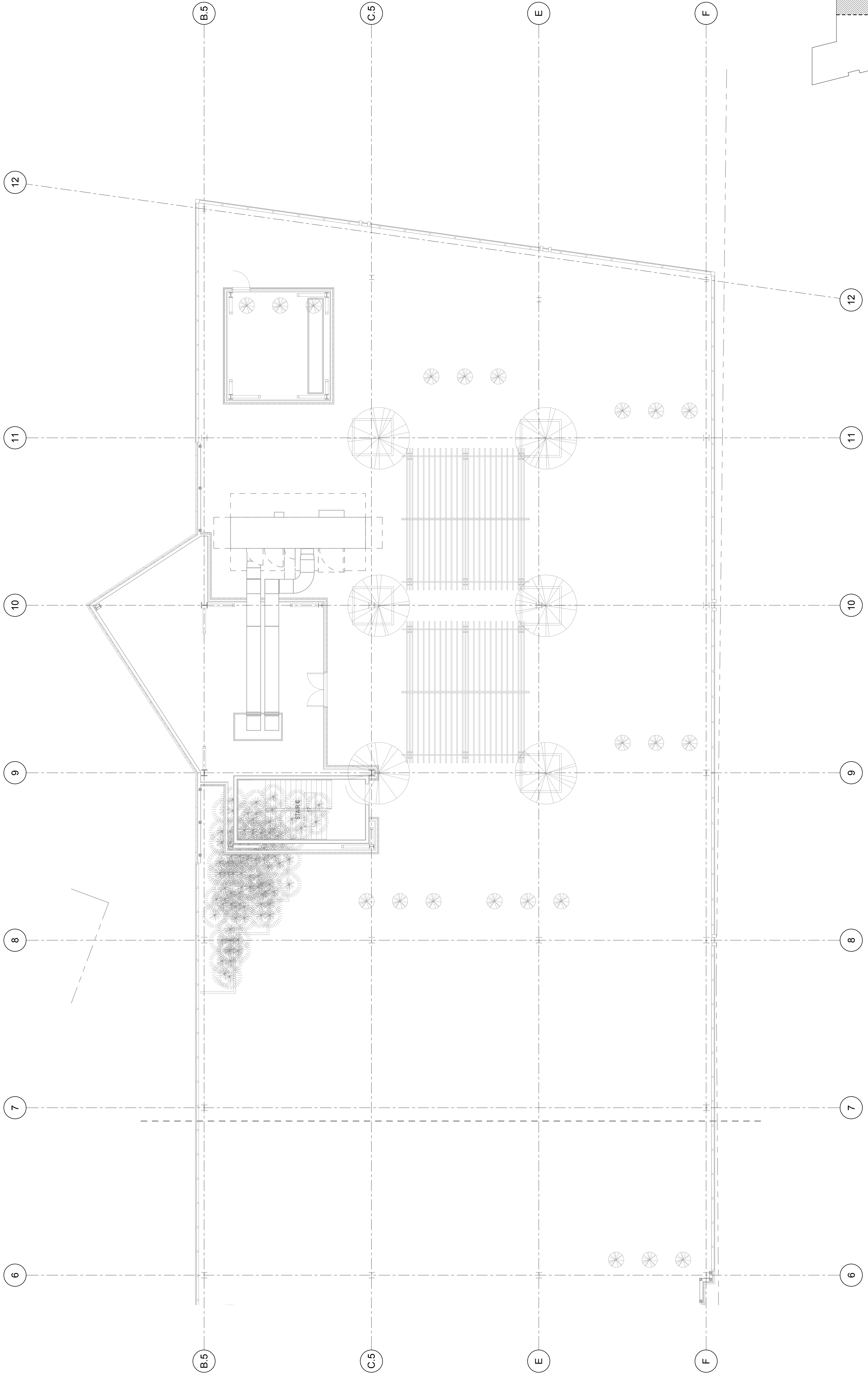
① 4TH FLOOR HVAC DUCTWORK PLAN B 1/8" = 1'-0"
