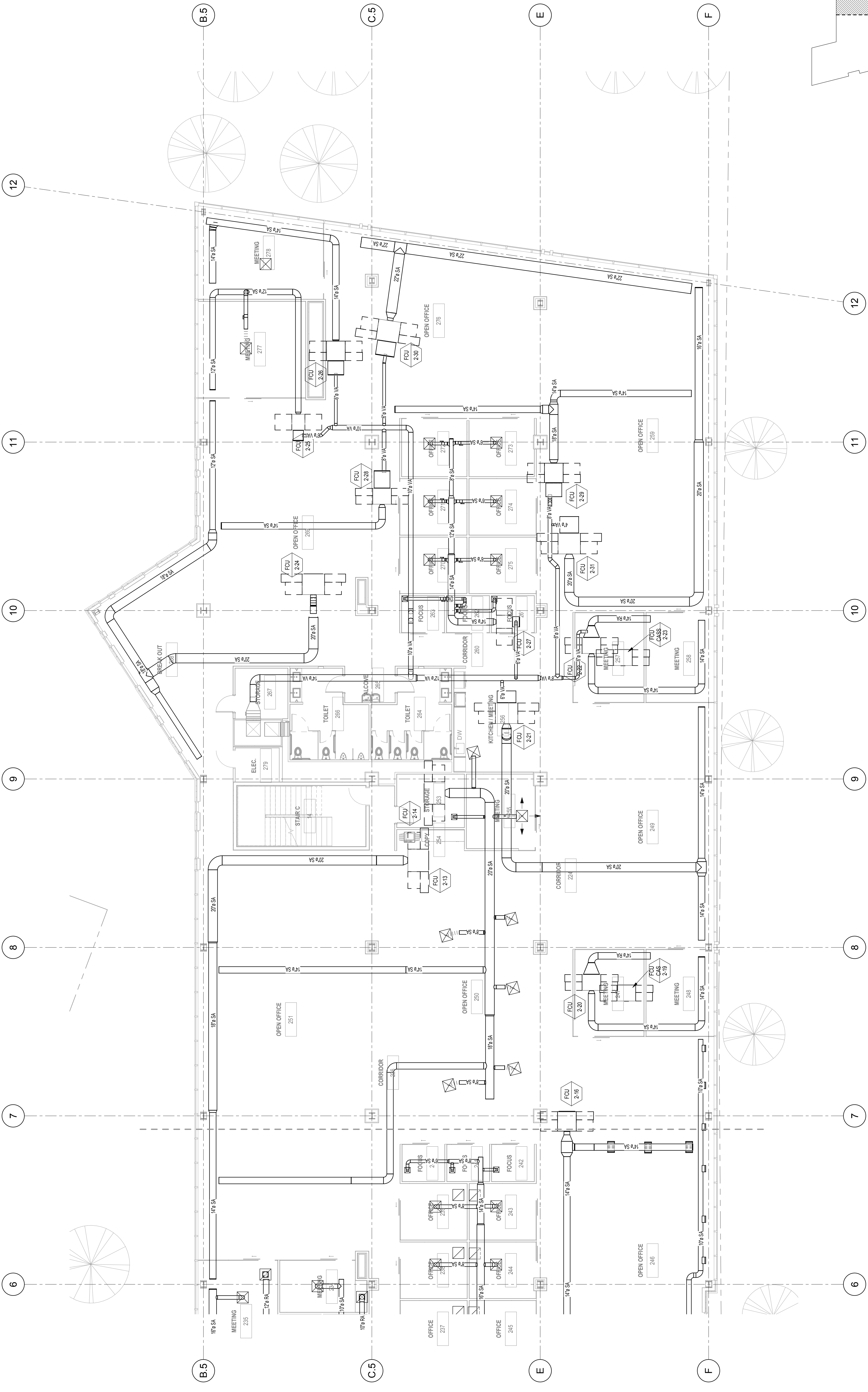
1 2ND FLOOR HVAC DUCTWORK PLAN B 1/8" = 1'-0"
