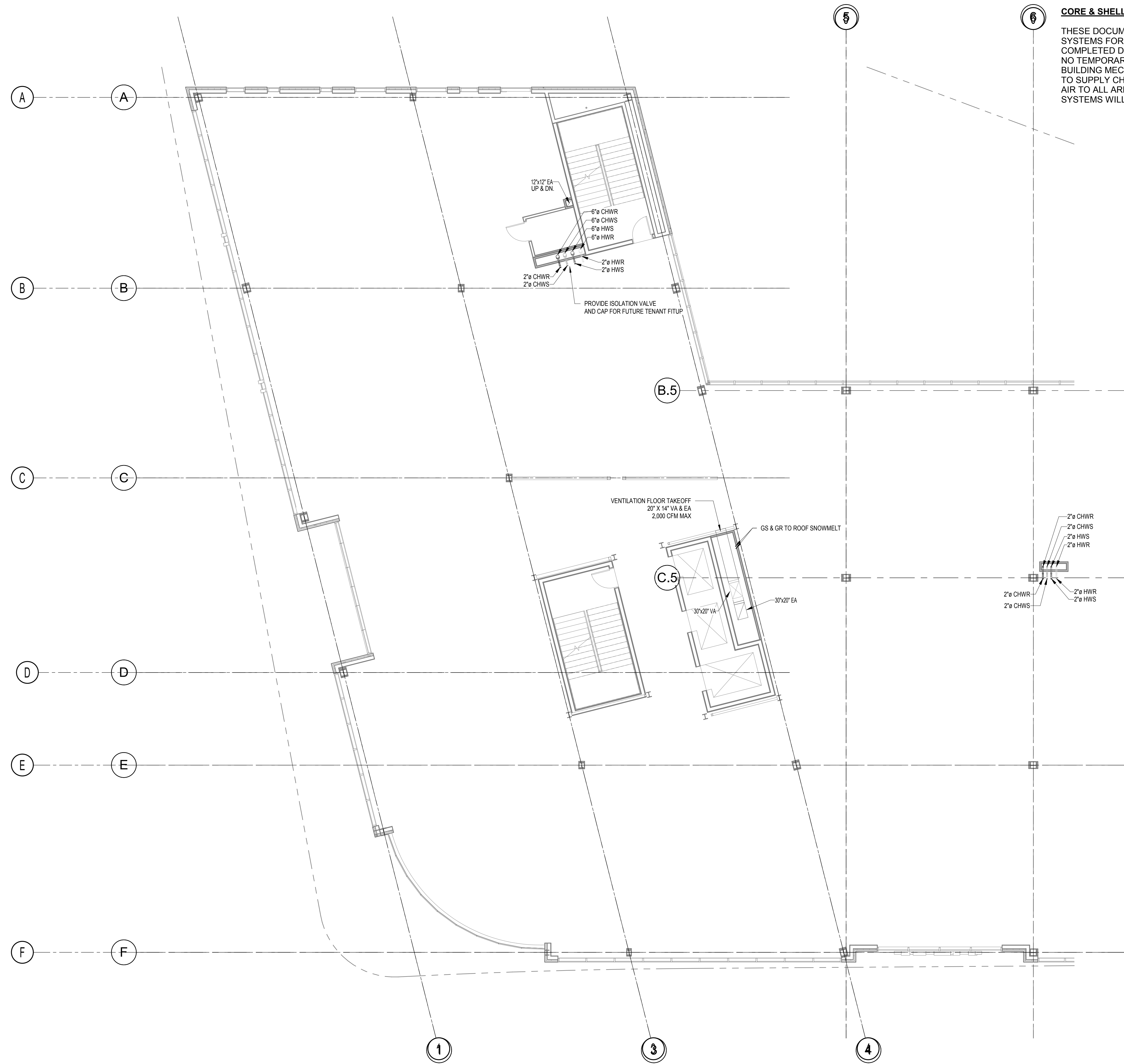
① 3RD FLOOR HVAC A 1/8" = 1'-0"
