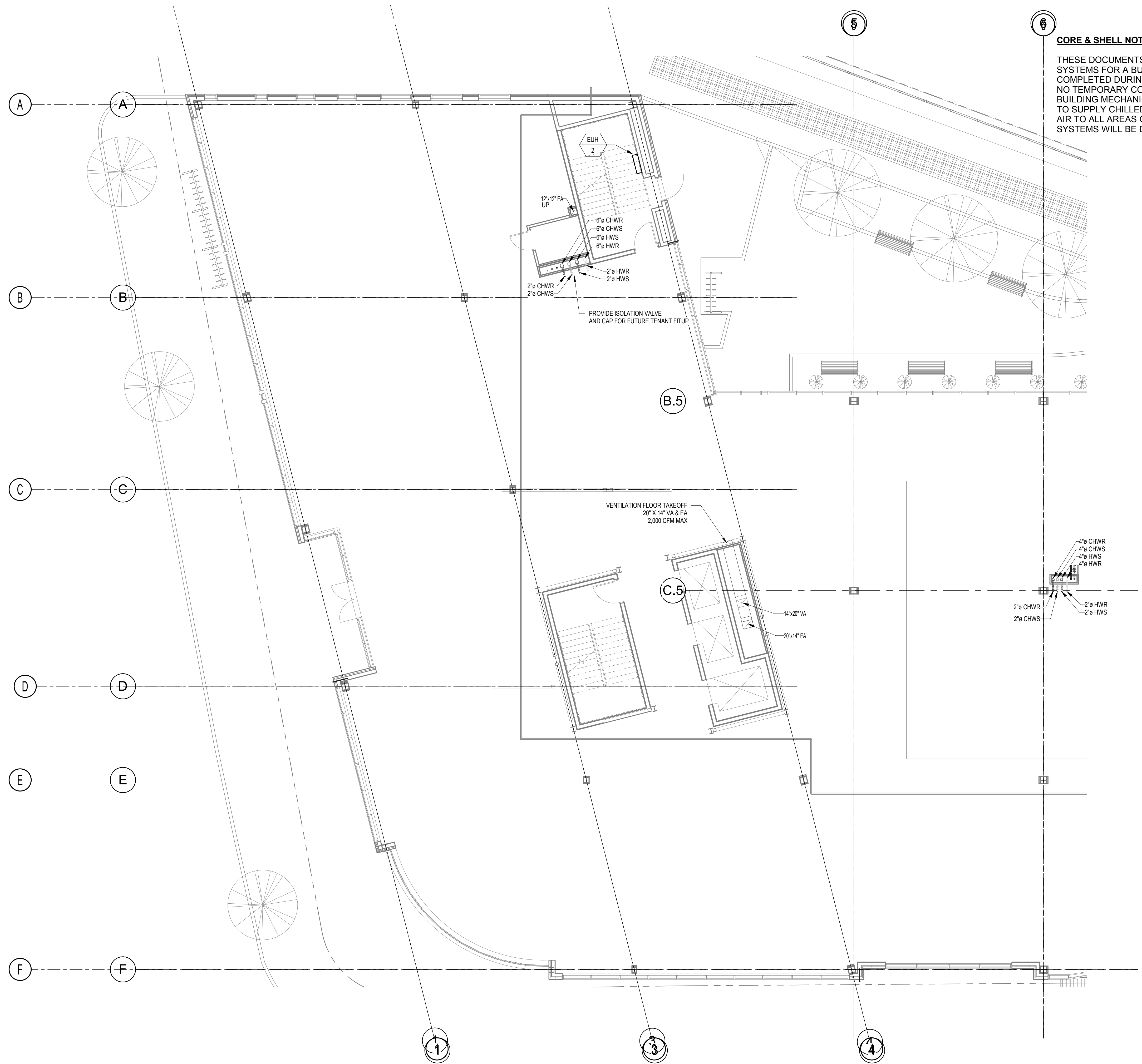
① 1ST FLOOR HVAC A 1/8" = 1'-0"
