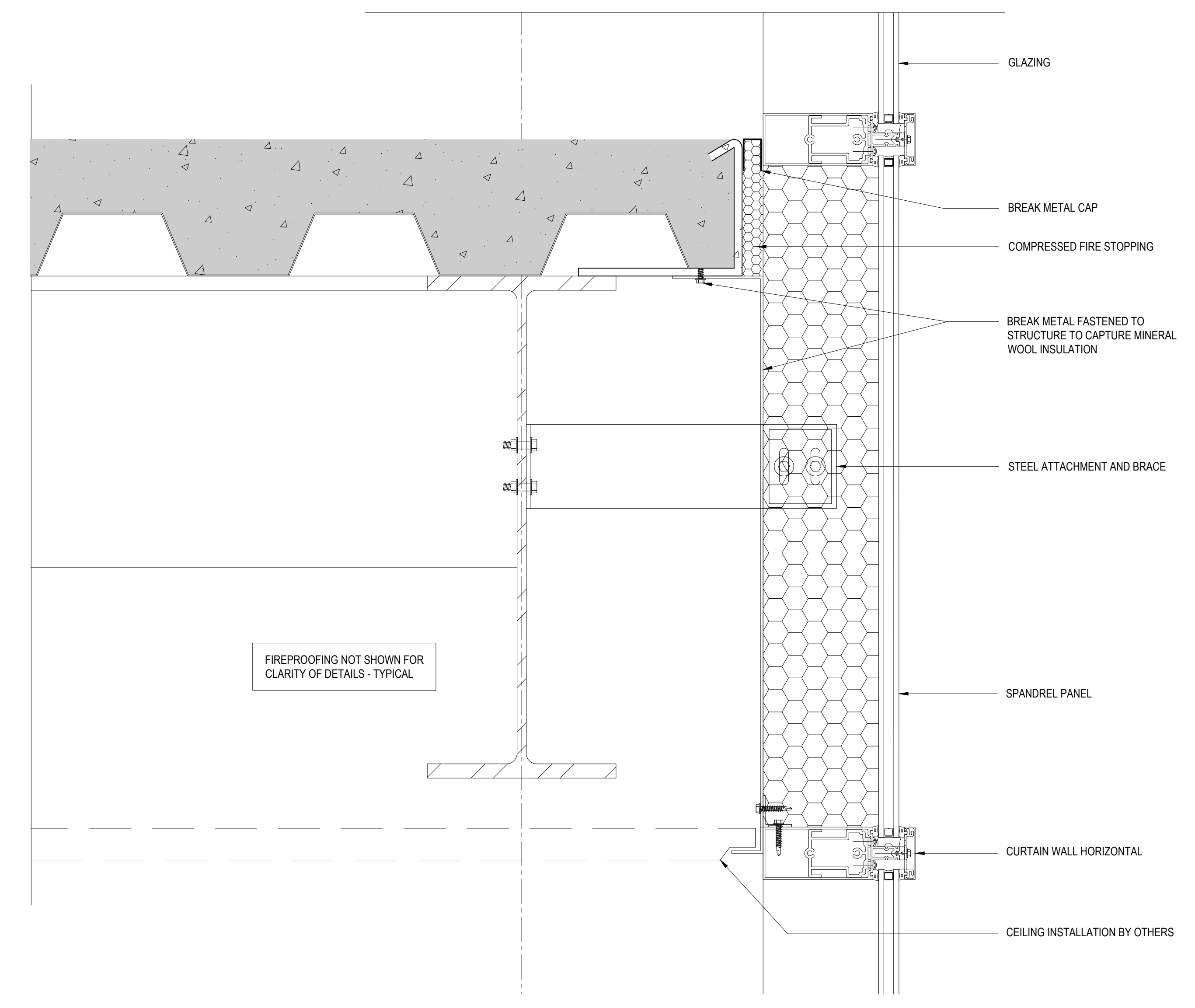
4 FLOOR PLATE AT EXTERIOR CURTAIN WALL WALL DETAIL SCALE: 3"=1'-0"
