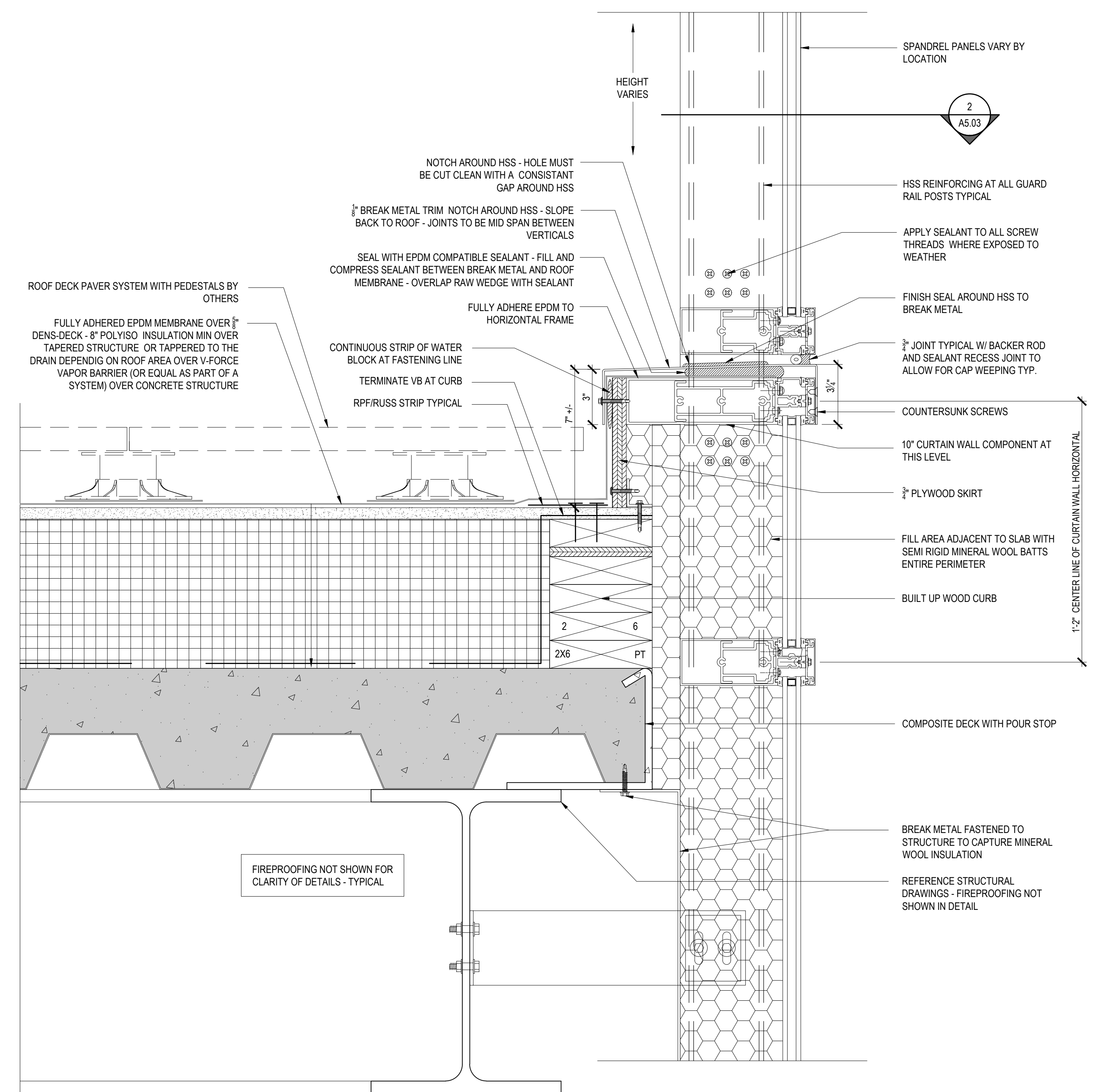
3 ROOF DECK DETAIL - CURTAIN WALL WALL DETAIL - ROOF DETAILS SCALE: 3"=1'-0"
