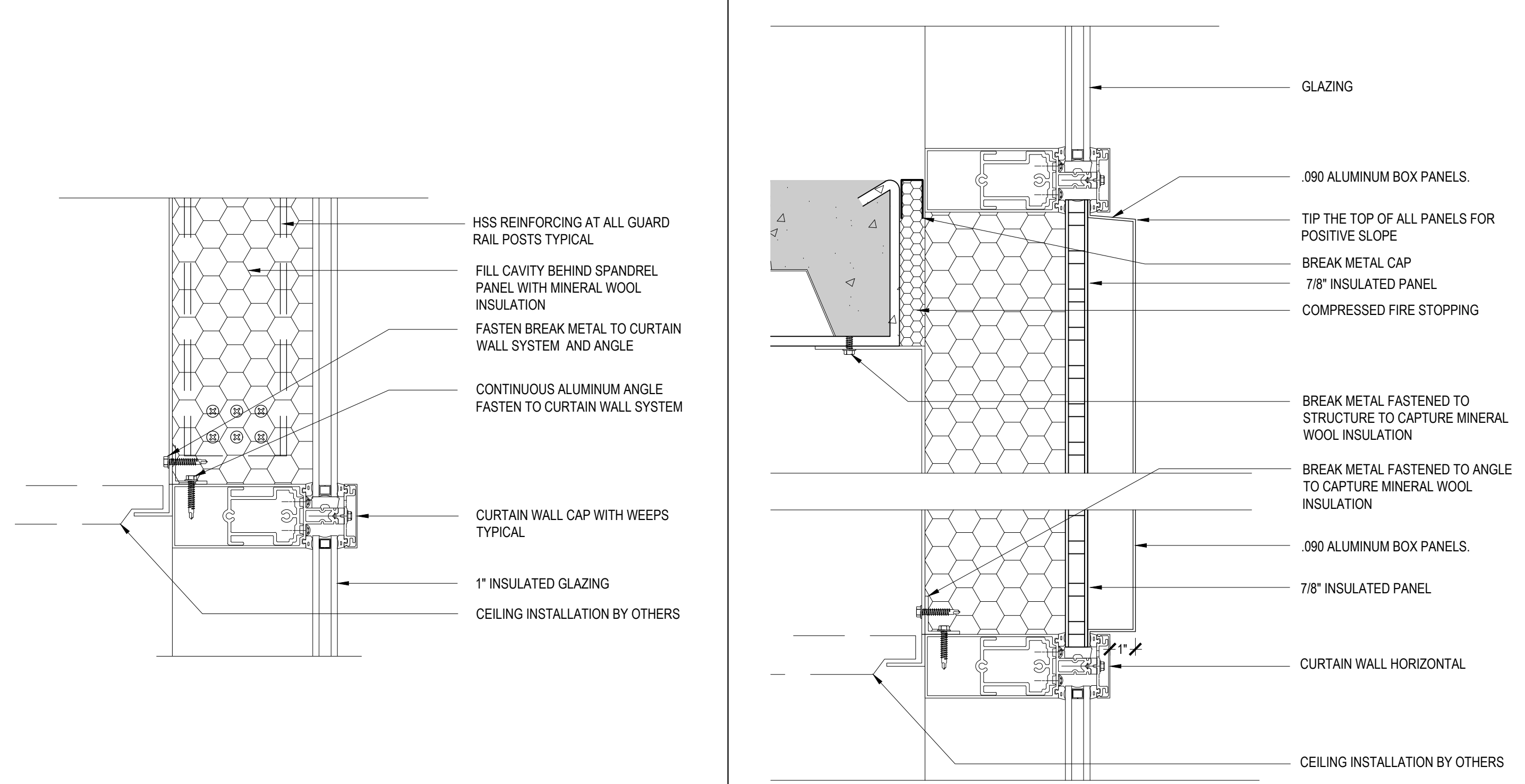
4 FLOOR PLATE AT EXTERIOR CURTAIN WALL WALL DETAIL SCALE: 3"=1'-0"
