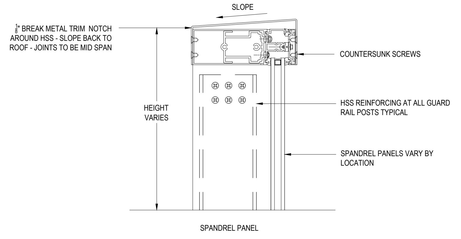
5 GUARD RAIL TOP DETAIL - CURTAIN WALL WALL DETAIL SCALE: 3"=1'-0"
