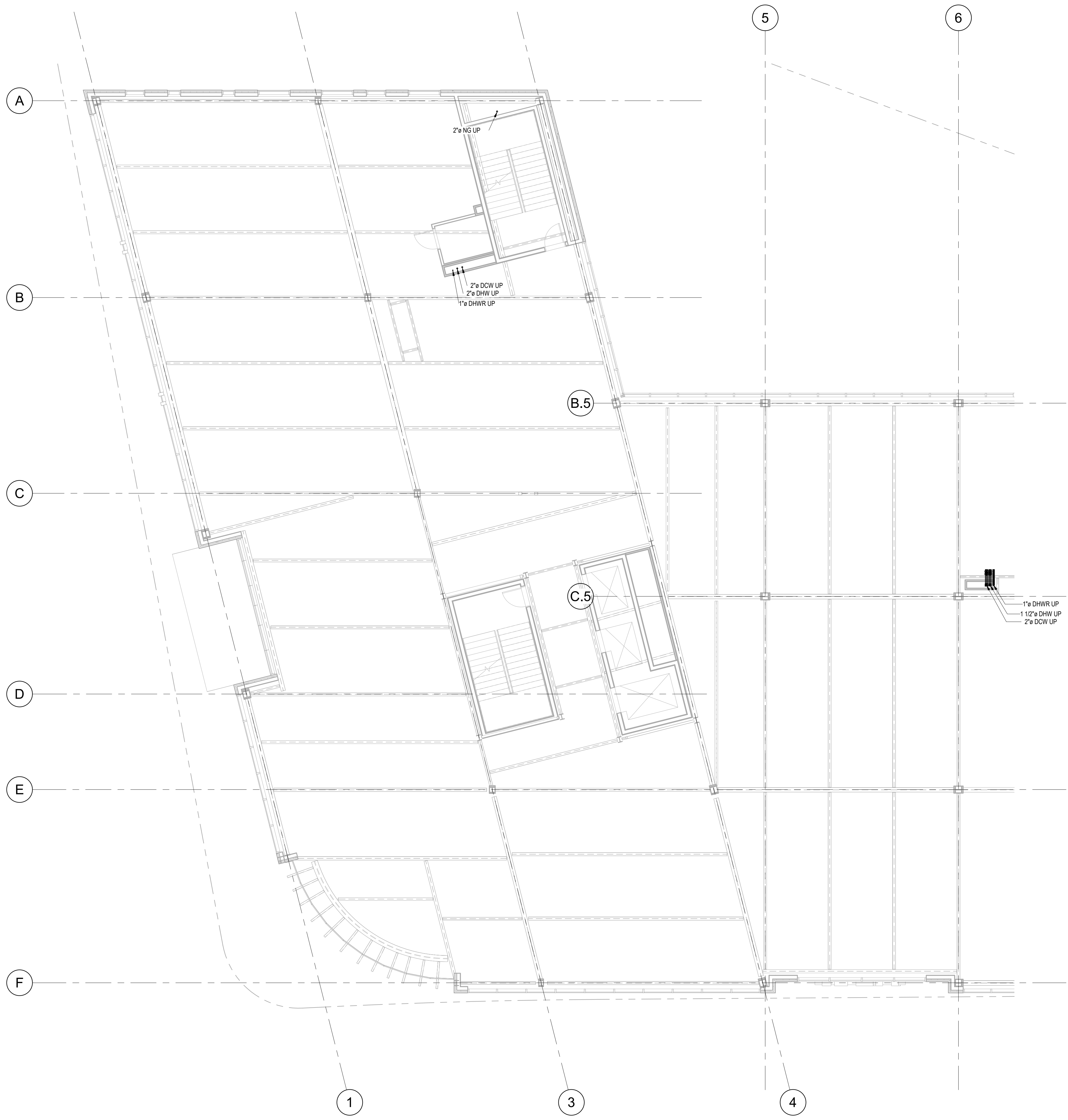
① 3RD FLOOR PPE A 1/8" = 1'-0"
