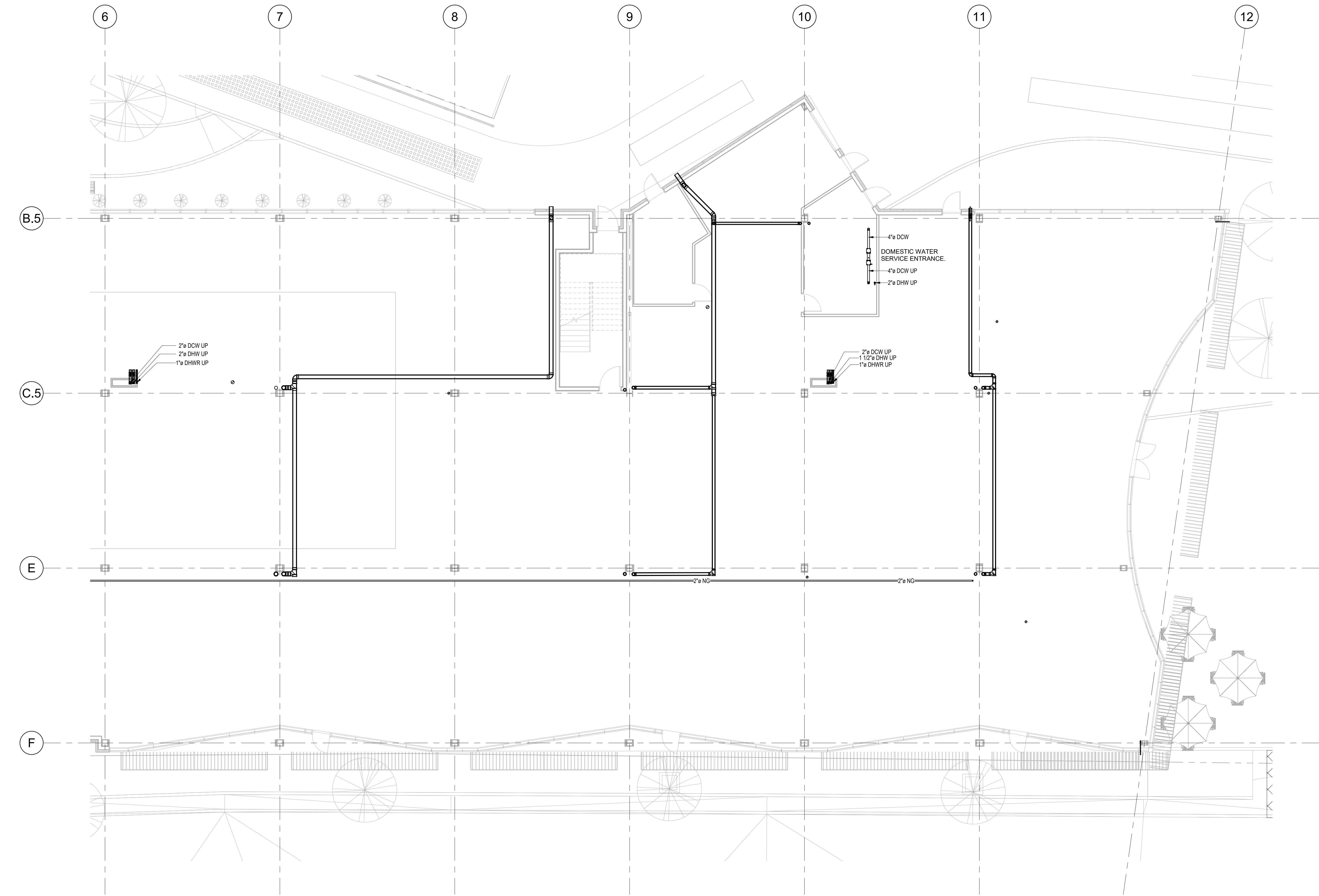
1 1ST FLOOR PPE B 1/8" = 1'-0"
