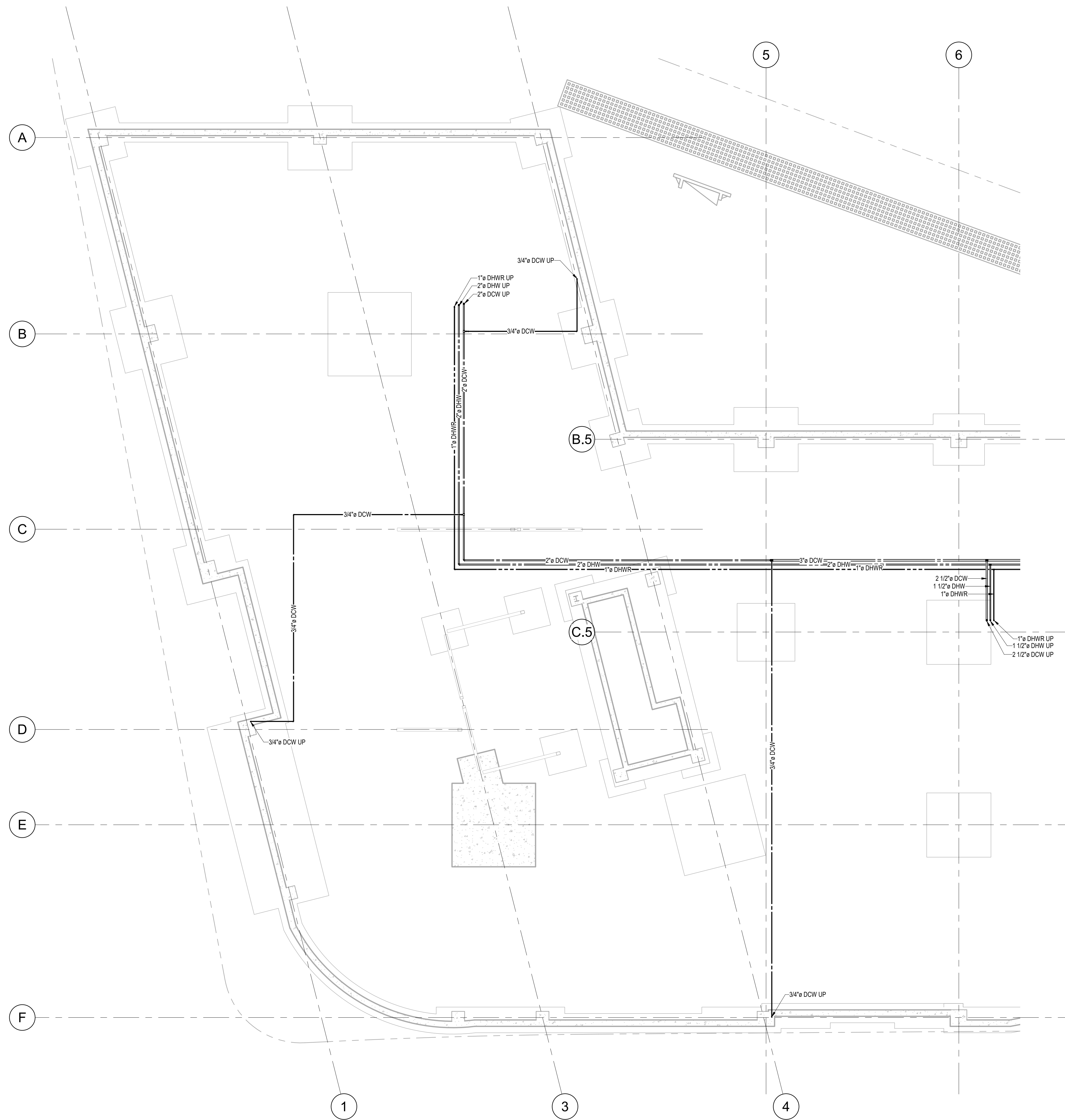
① LEVEL 0 - UNDER SLAB PPE A 1/8" = 1'-0"
