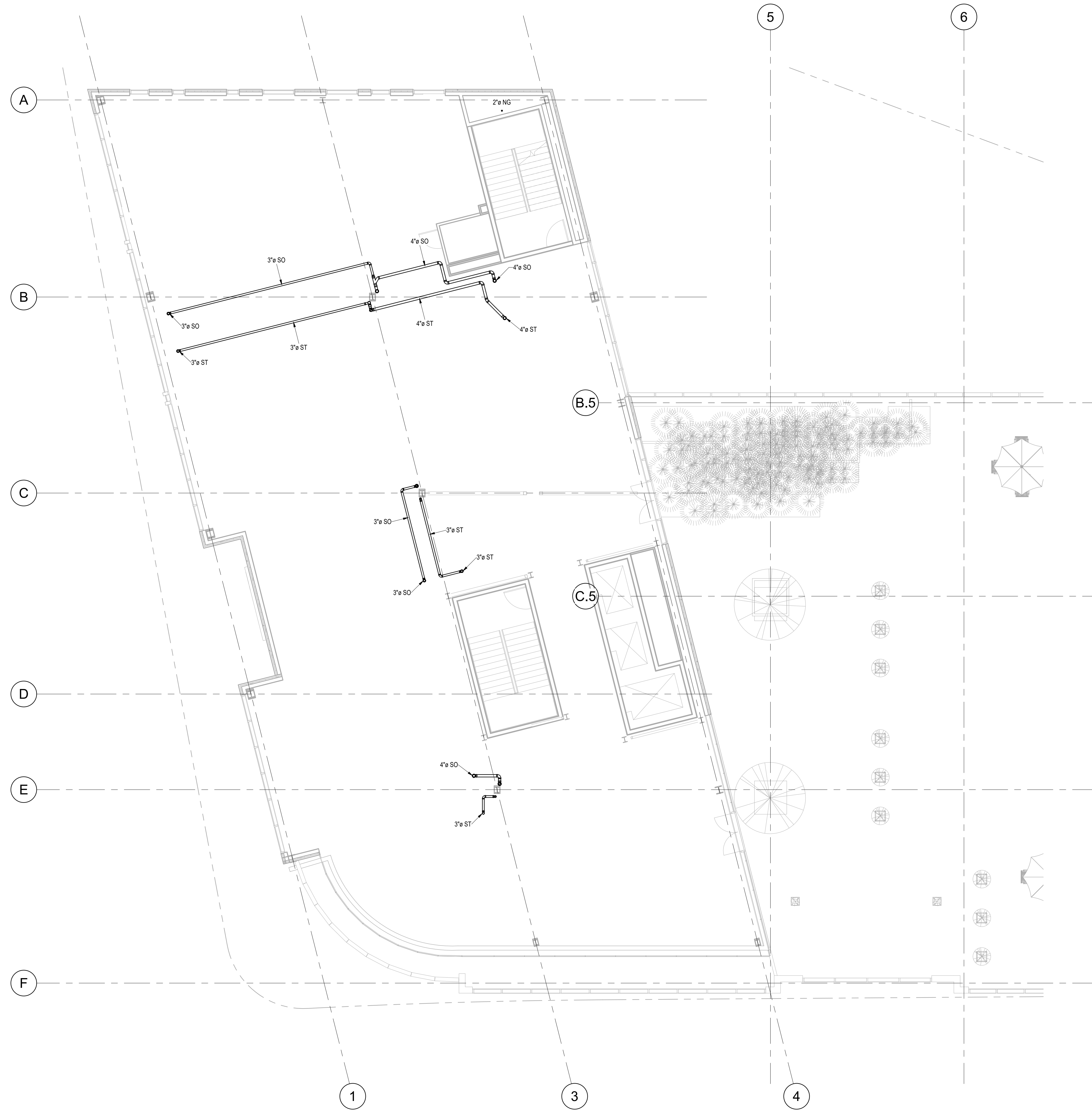
① 4TH FLOOR DWV A 1/8" = 1'-0"
