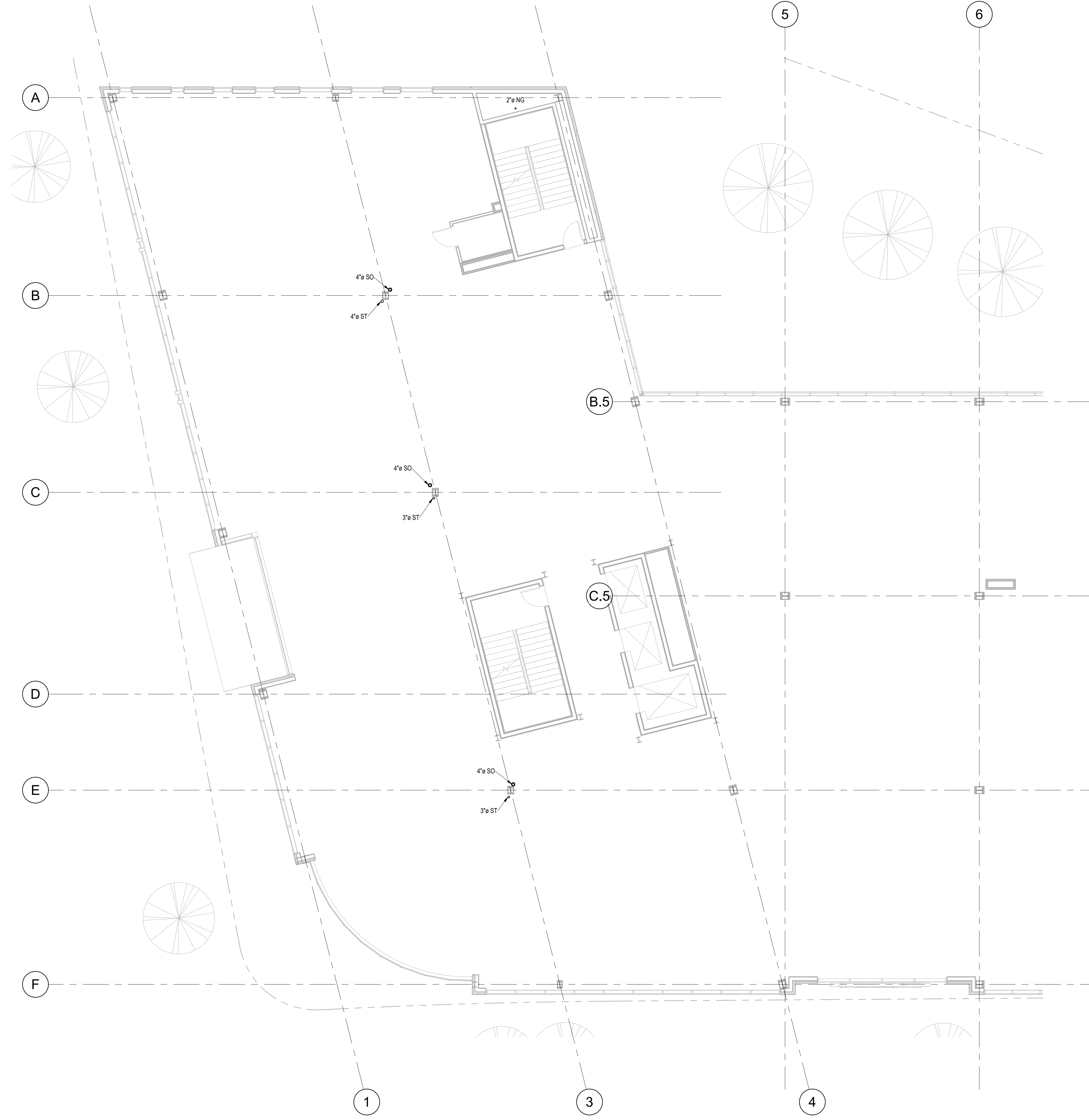
① 2ND FLOOR DWV A 1/8" = 1'-0"
