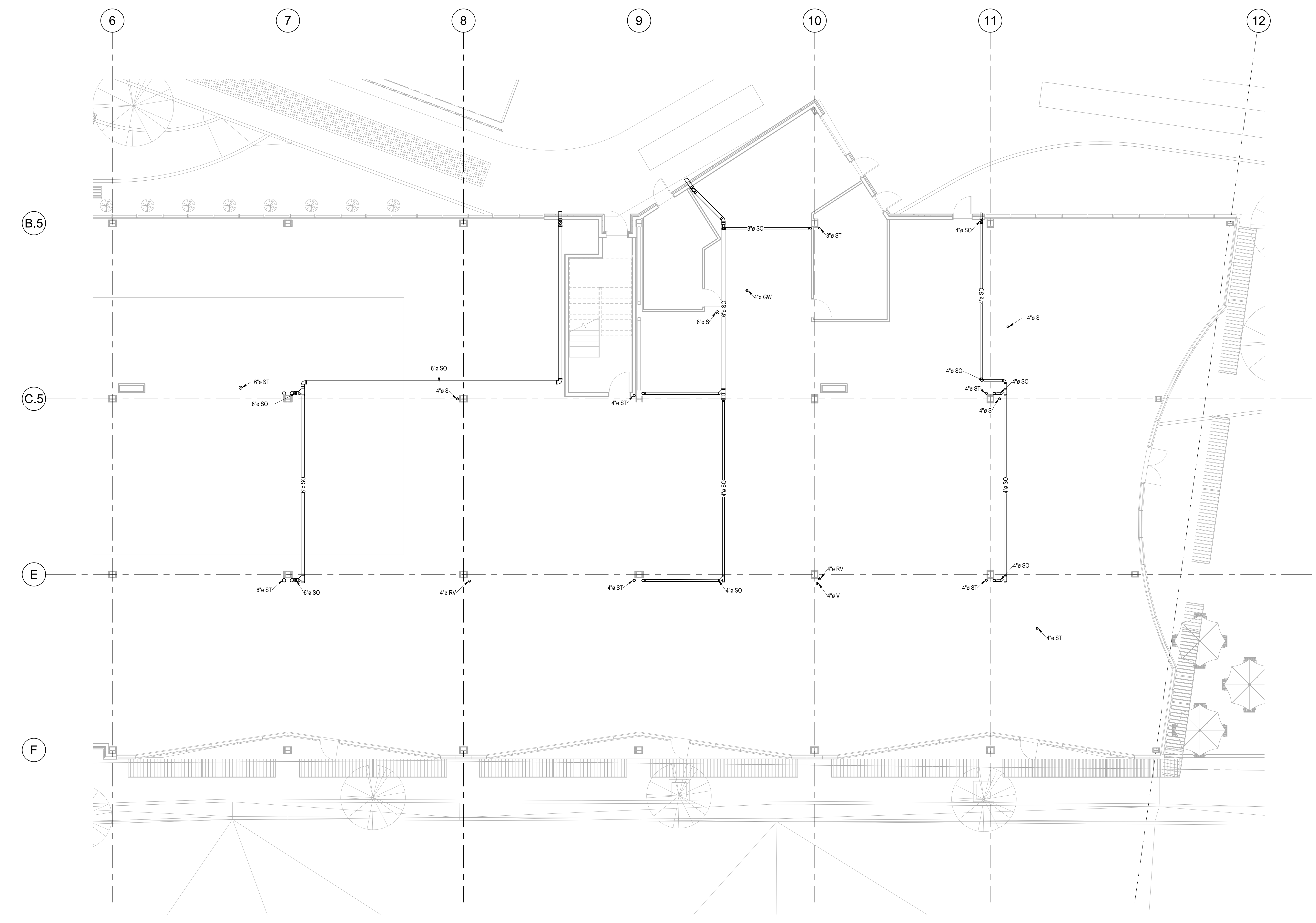
1 1ST FLOOR DWV B 1/8" = 1'-0"
