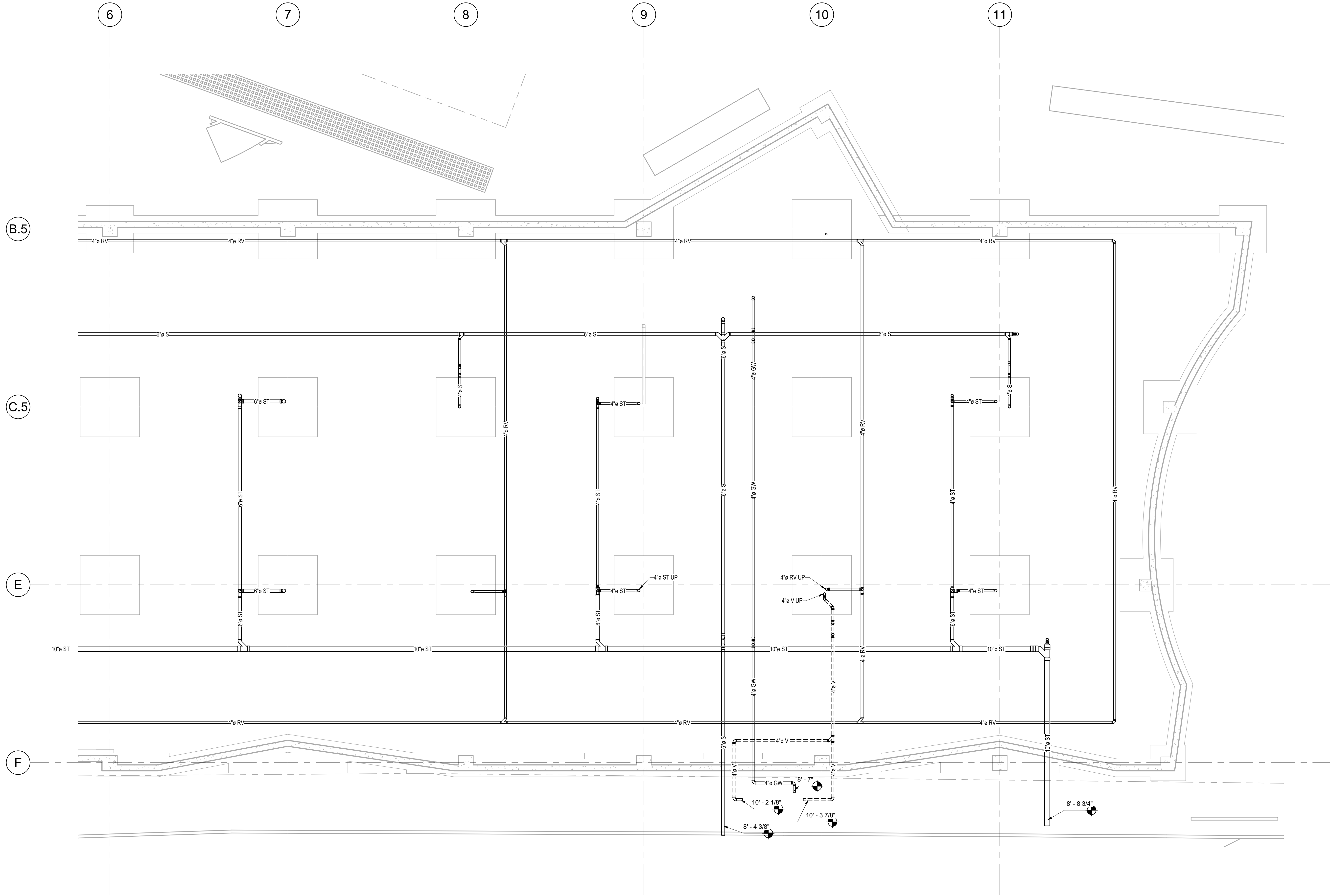
① LEVEL 0 - UNDER SLAB DWV B 1/8" = 1'-0"
