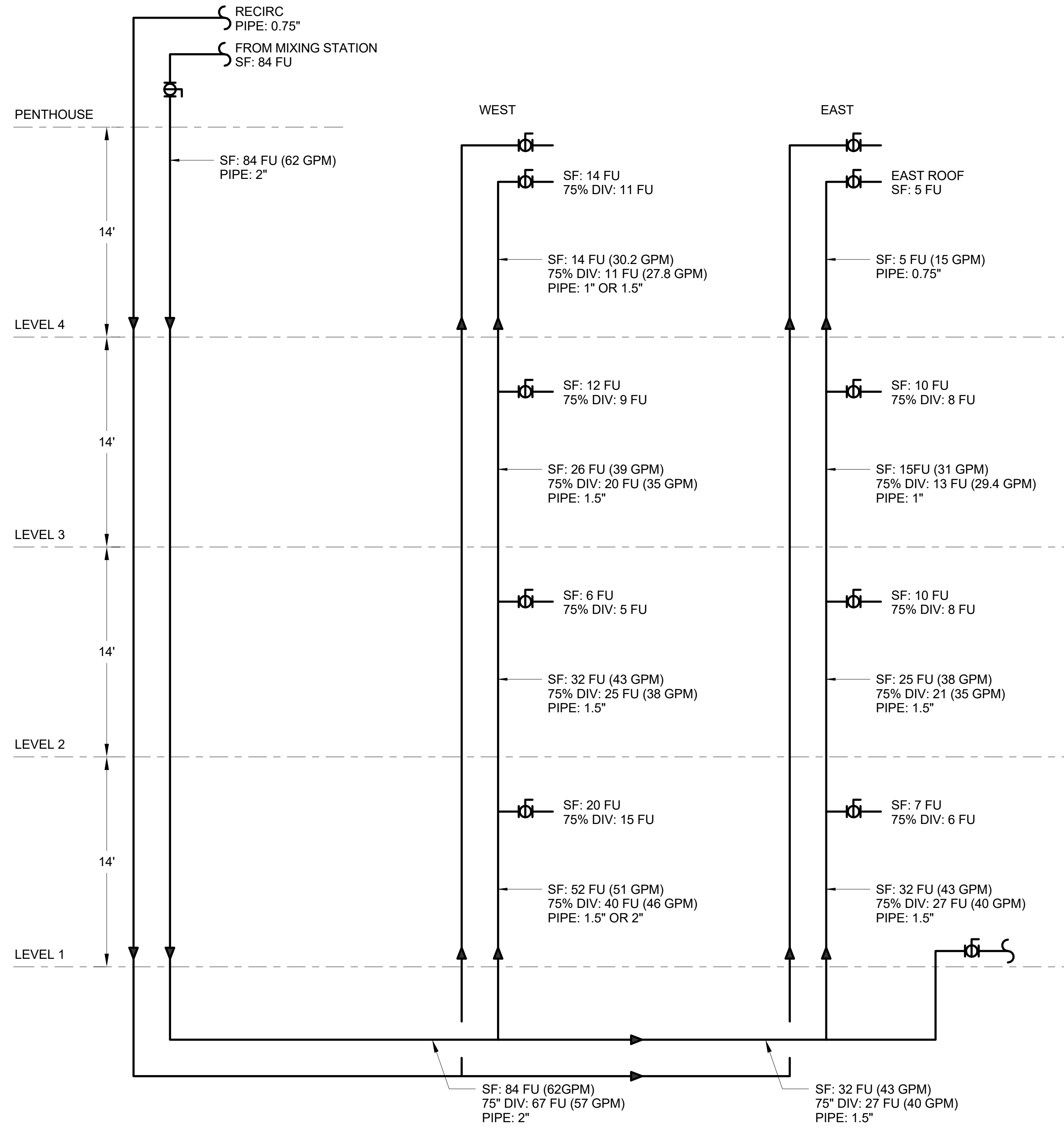
HOT WATER RISER DIAGRAM
