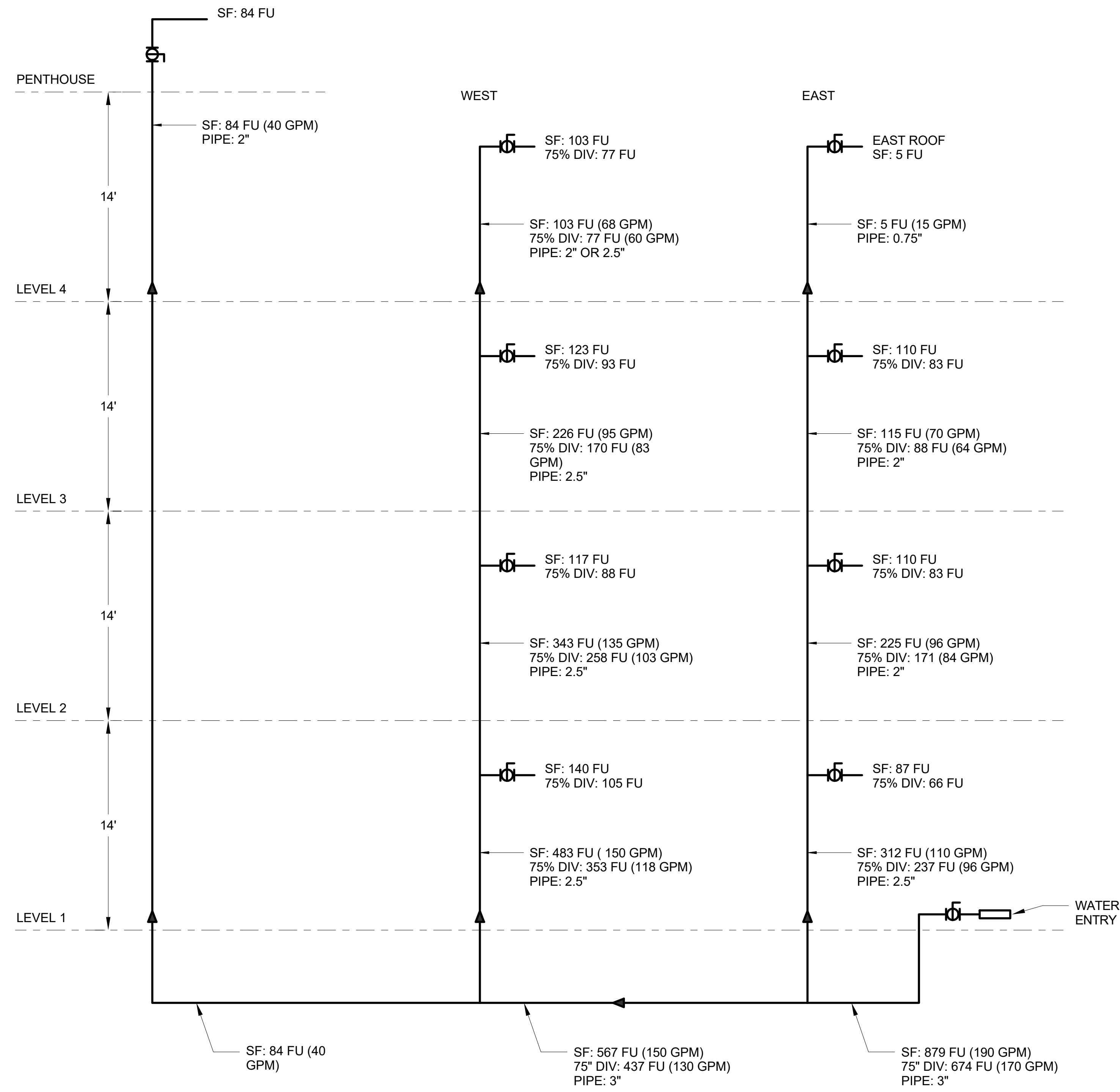
COLD WATER RISER DIAGRAM
